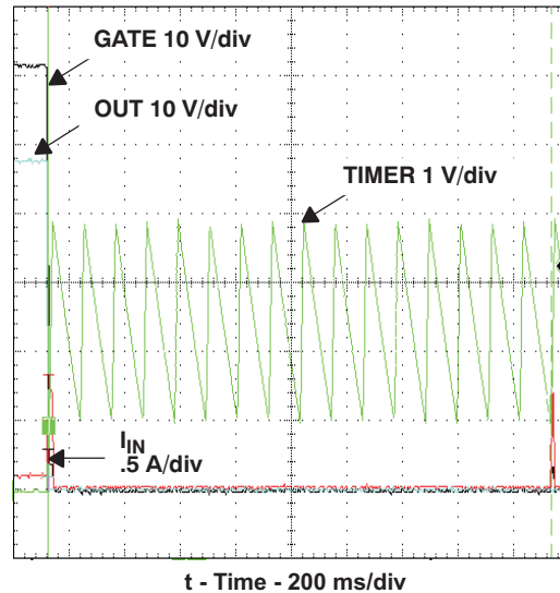
Figure 17. TPS2491 Restart Cycle Timing
