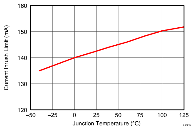
Figure 13. PoE Inrush Current Limit vs Temperature
