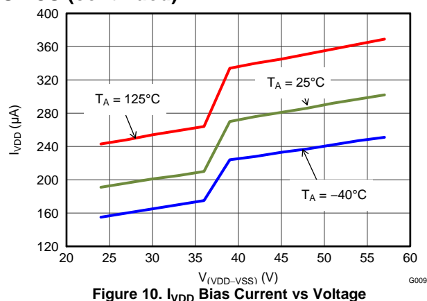
Figure 10. I_VDD Bias Current vs Voltage
