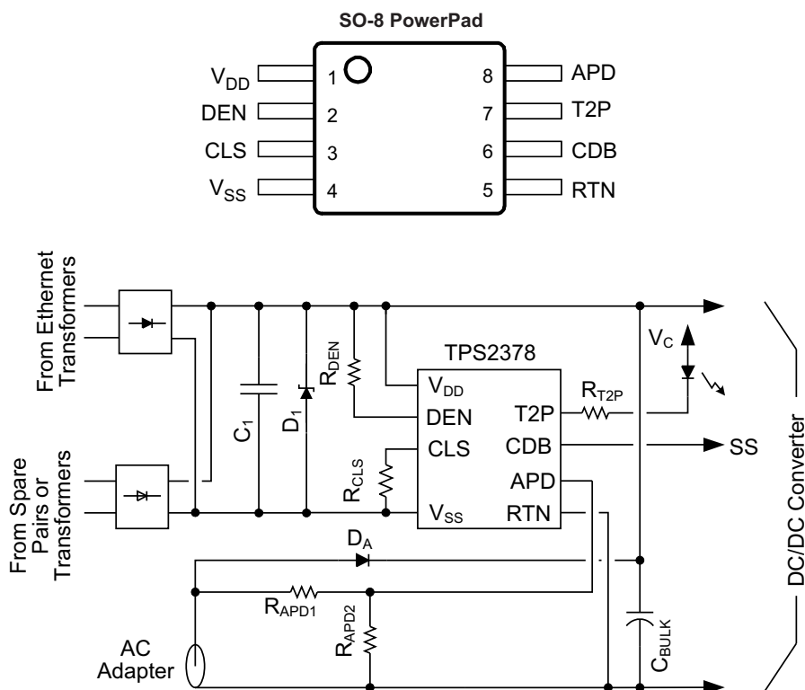
Figure 1. Typical Application
