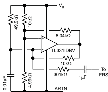
Figure 37. Frequency Dithering
