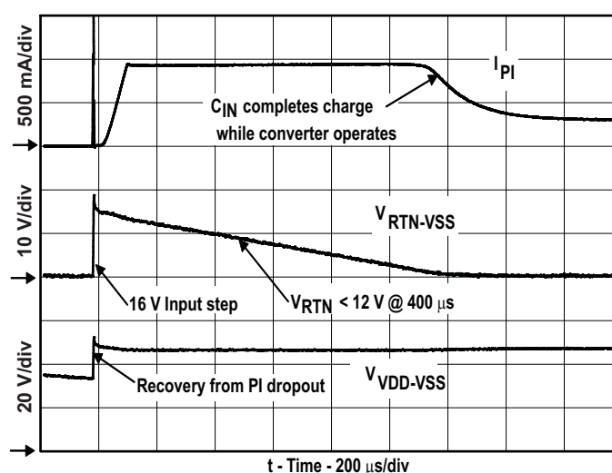
Figure 26. Response to PSE Step Voltage
