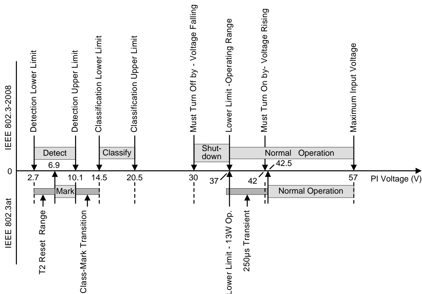
Figure 20. Threshold Voltages
