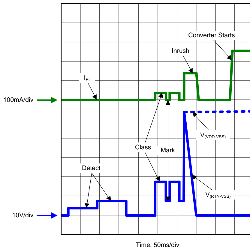
Figure 22. Startup
