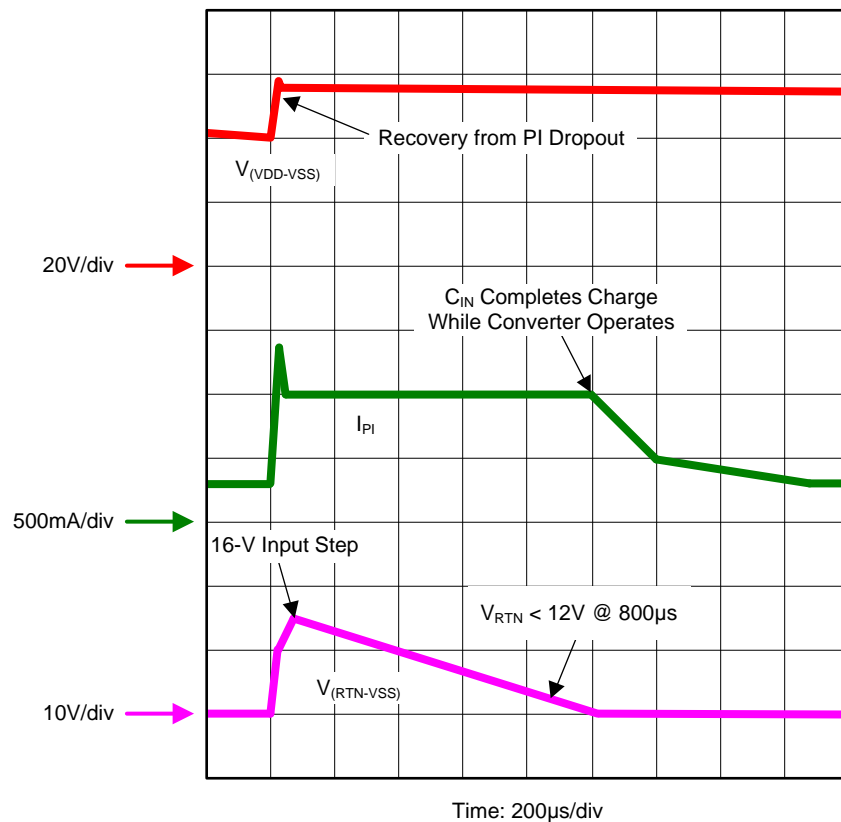
Figure 25. Response to Output Short Circuit
