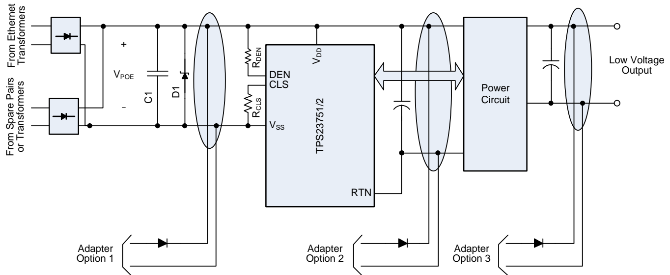
Figure 28. ORing Configurations
