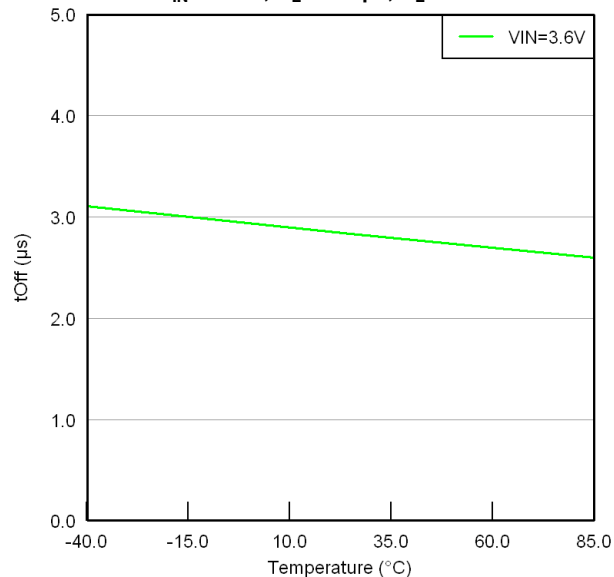
TURN-OFF TIME vs TEMPERATURE VIN = 3.6 V, CL = 0.1 \mu F, RL = 10 \Omega
