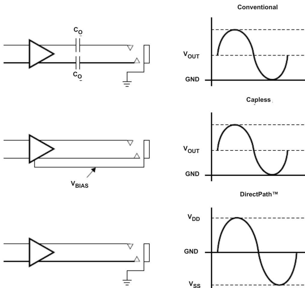
Figure 28. Amplifier Applications
