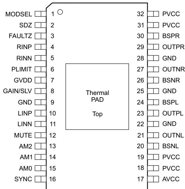
TPA3116D2 32-PIN HTSSOP PACKAGE (DAD) PACKAGE (TOP VIEW)
