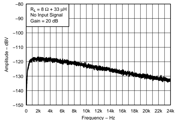
Figure 16. A-WEIGHTED OUTPUT NOISE vs FREQUENCY
