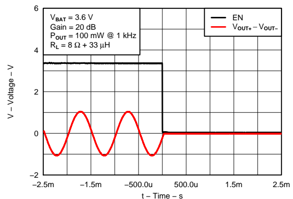
Figure 18. SHUTDOWN TIMING
