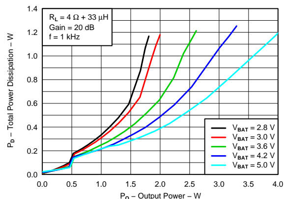
Figure 12. TOTAL POWER DISSIPATION vs OUTPUT POWER
