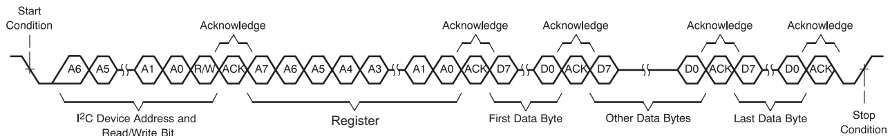
Figure 42. Multiple-Byte Write Transfer
