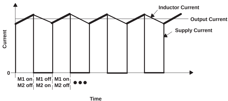
Figure 5. Class-D Currents
