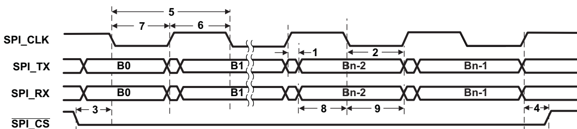
Figure 6-27. SPI Mode 1 Transfer (CKP n = 0, CKPH n = 1)
