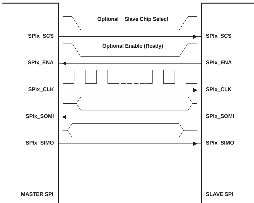
Figure 5-36. Illustration of SPI Master-to-SPI Slave Connection
