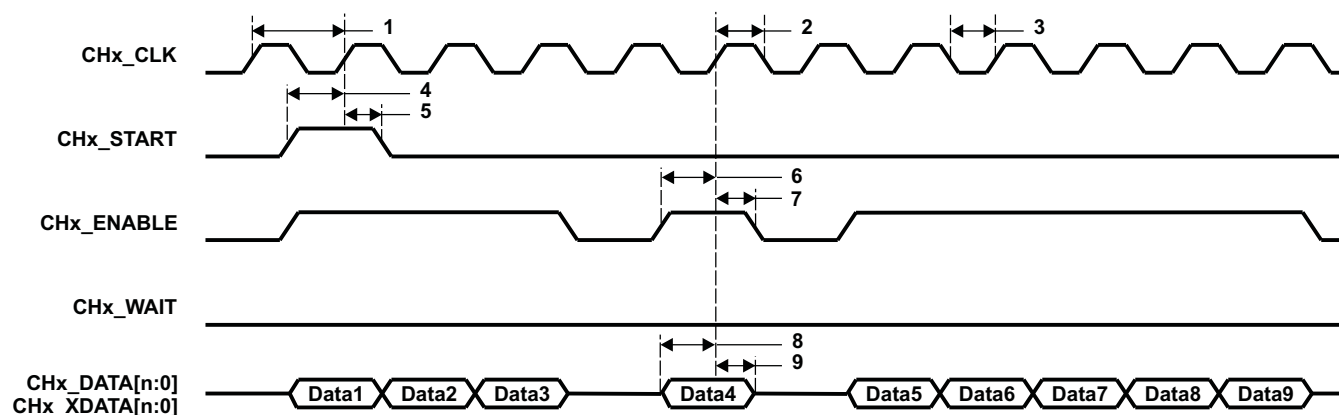
Figure 5-57. uPP Single Data Rate (SDR) Receive Timing
