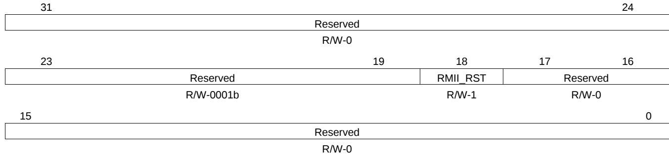
Figure 3-8. EMAC Configuration Register (EMACCFG) - 0x02AC 0020
