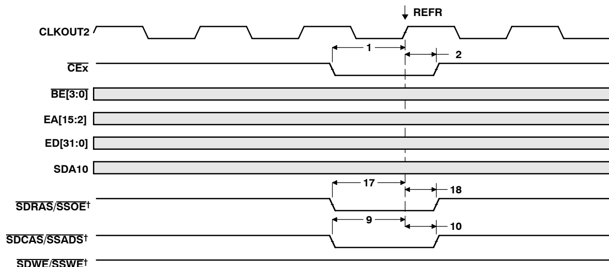
Figure 27. SDRAM REFR Command
