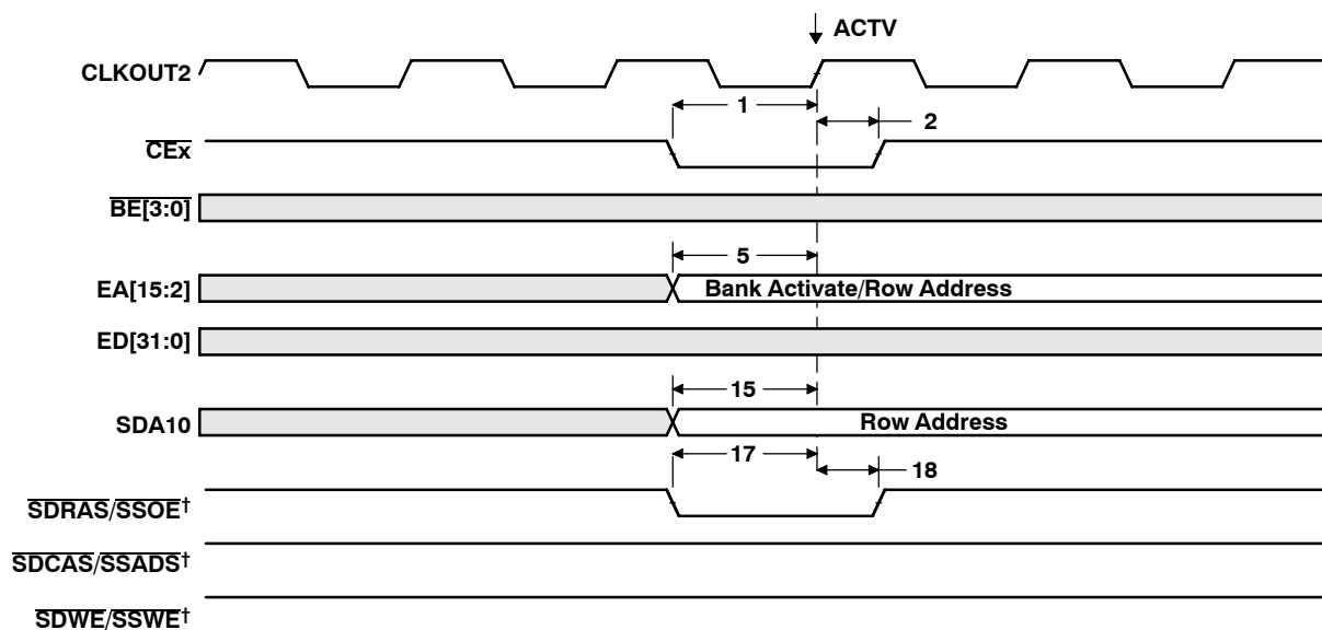
Figure 25. SDRAM ACTV Command
