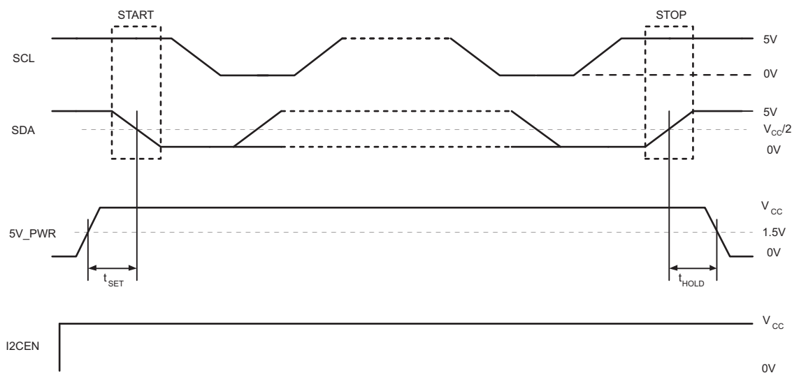
Figure 12. I²C Setup and Hold Definition
