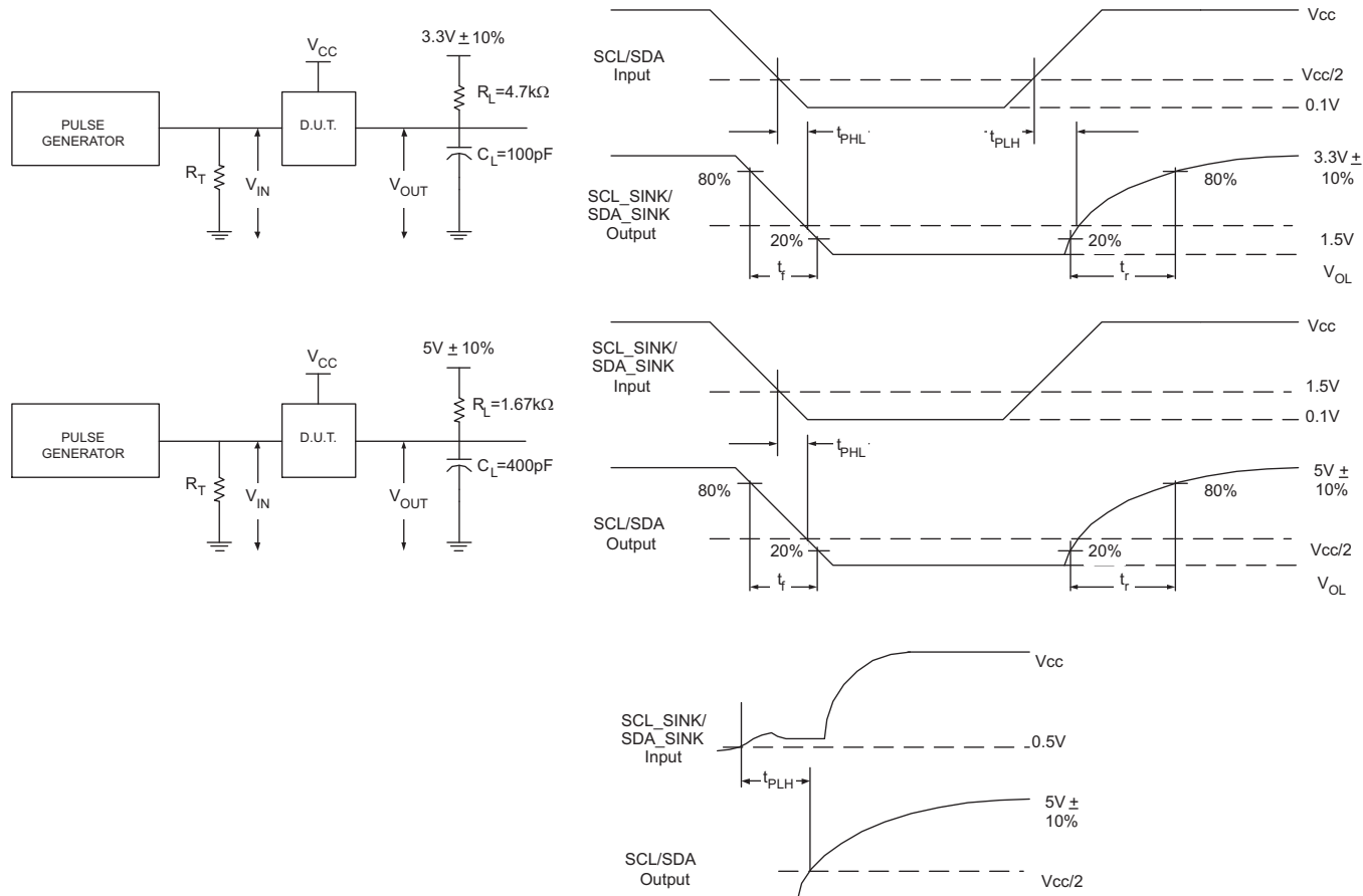
Figure 11. I²C Timing Test Circuit and Definition
