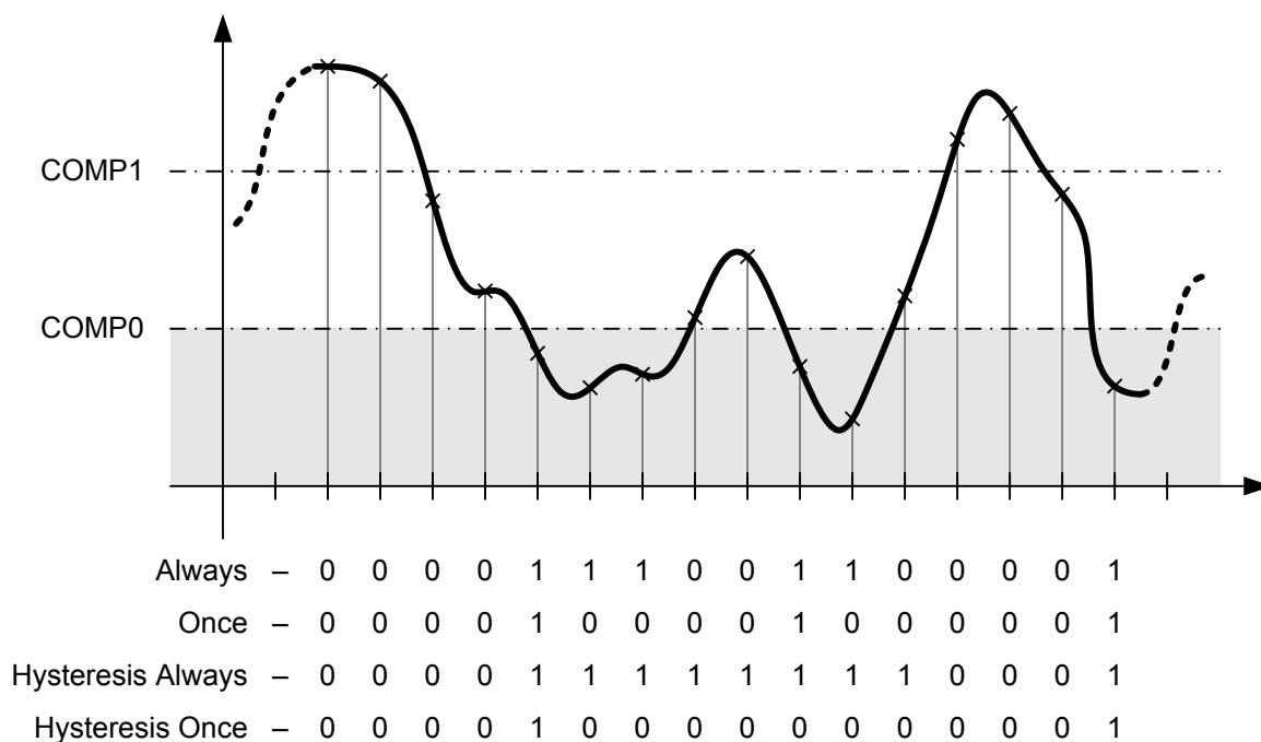
Figure 13-12. Low-Band Operation (C1C=0x0 and/or CTC=0x0)
