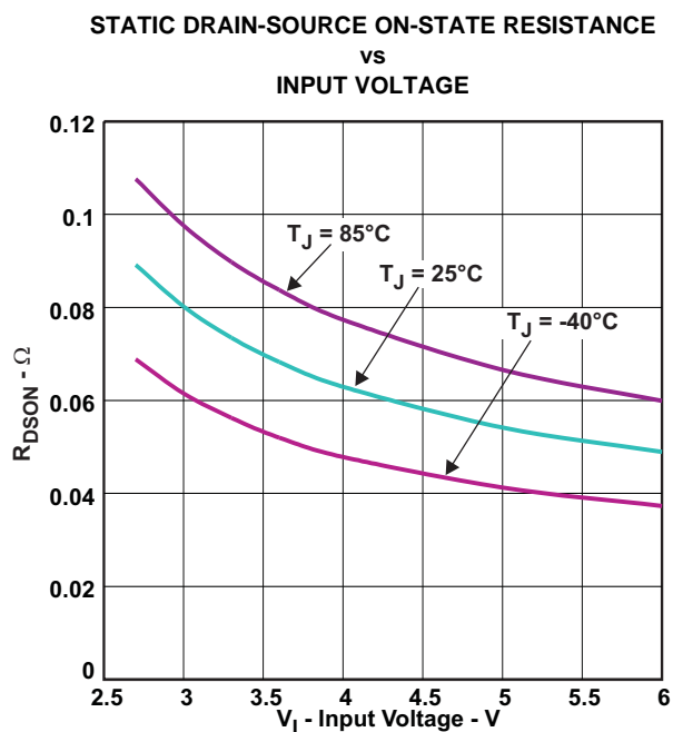
Figure 10. Low-Side Switch
