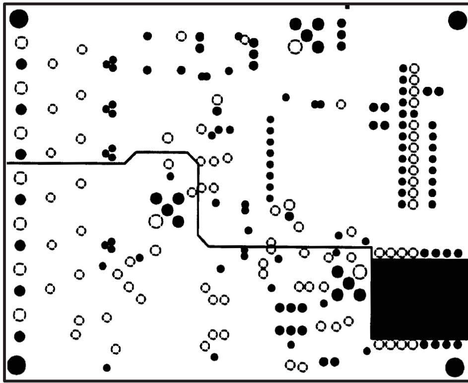
Internal Plane 1
