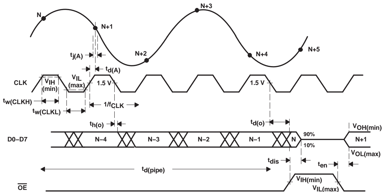
Figure 1. Timing Diagram
