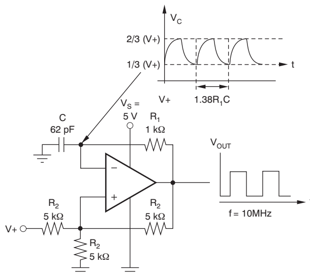
Figure 18. Relaxation Oscillator
