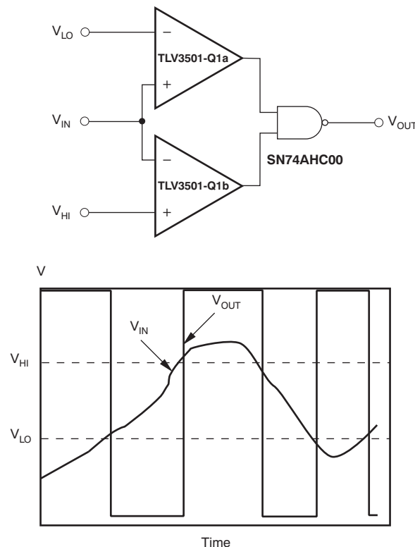
Figure 20. Window Comparator: Active Low
