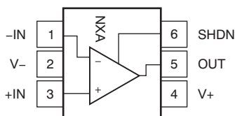
SOT23-6 (1) DBV PACKAGE (TOP VIEW)
