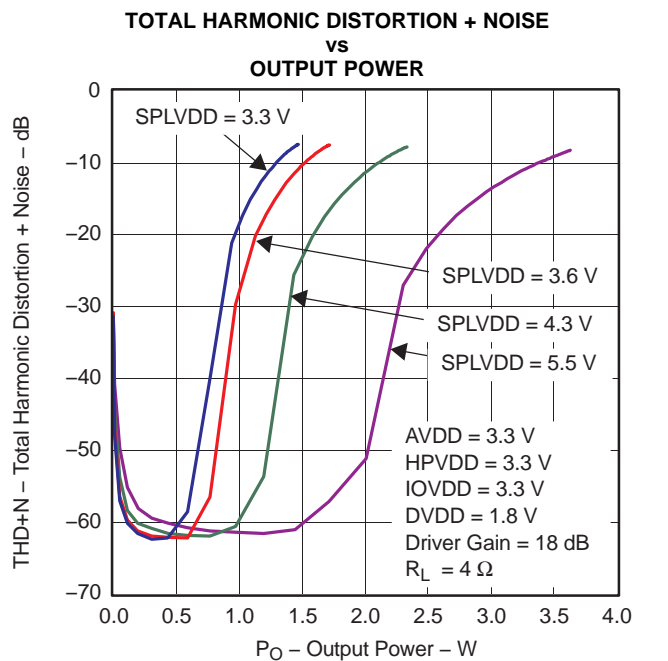
Figure 4-11. Class-D Speaker-Driver Output Power ( R_L = 4 \Omega )
