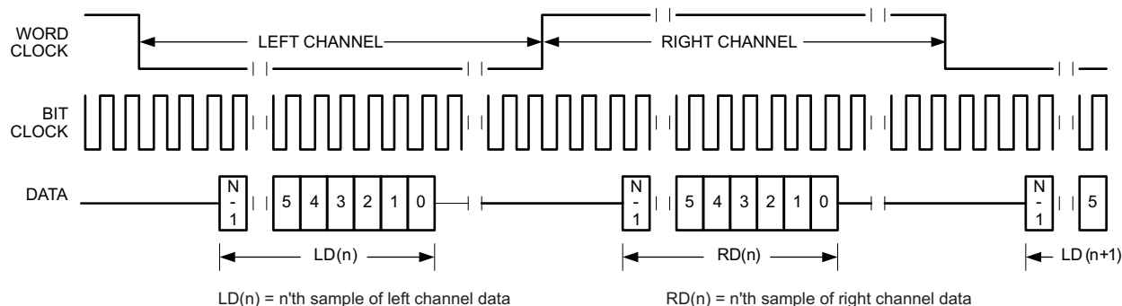
Figure 5-43. Timing Diagram for I²S Mode With Offset = 2
