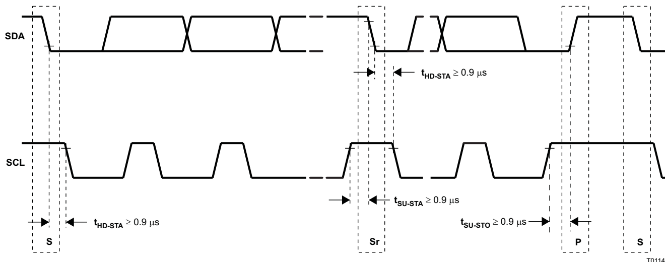
Figure 14. I 2 C Interface Timing
