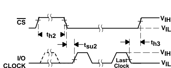
Figure 27. \overline{CS} and I/O CLOCK Voltage Waveforms
