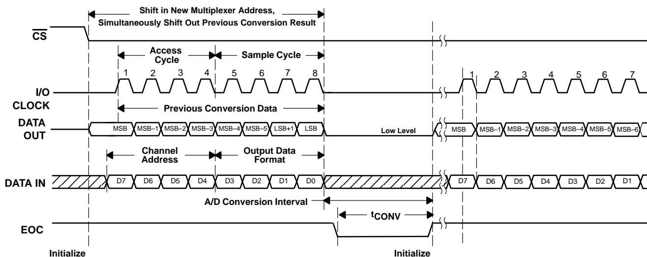
Figure 36. Timing for 8-Clock Transfer Not Using \overline{CS} With DATA OUT Set for MSB First
