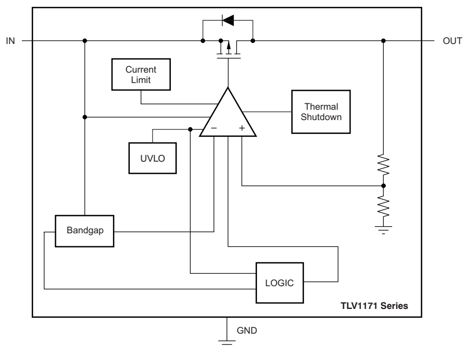
Figure 1. Block Diagram
