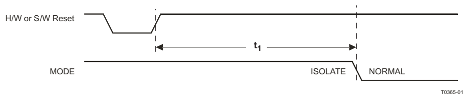
Figure 9-25. Isolation Timing
