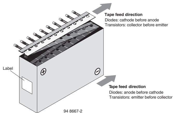
Fig. 7 - Tape Direction
