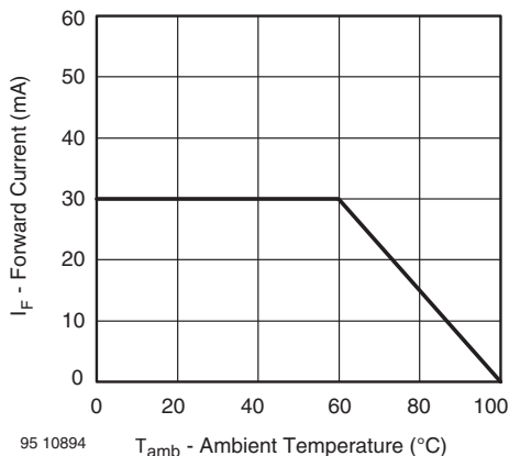
Fig. 1 - Forward Current vs. Ambient Temperature for InGa
