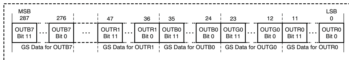
Figure 45. Grayscale Data Latch Configuration
