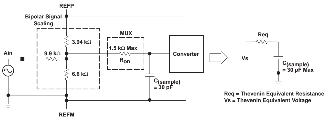
Figure 33. Equivalent Input Circuit Including the Driving Source
