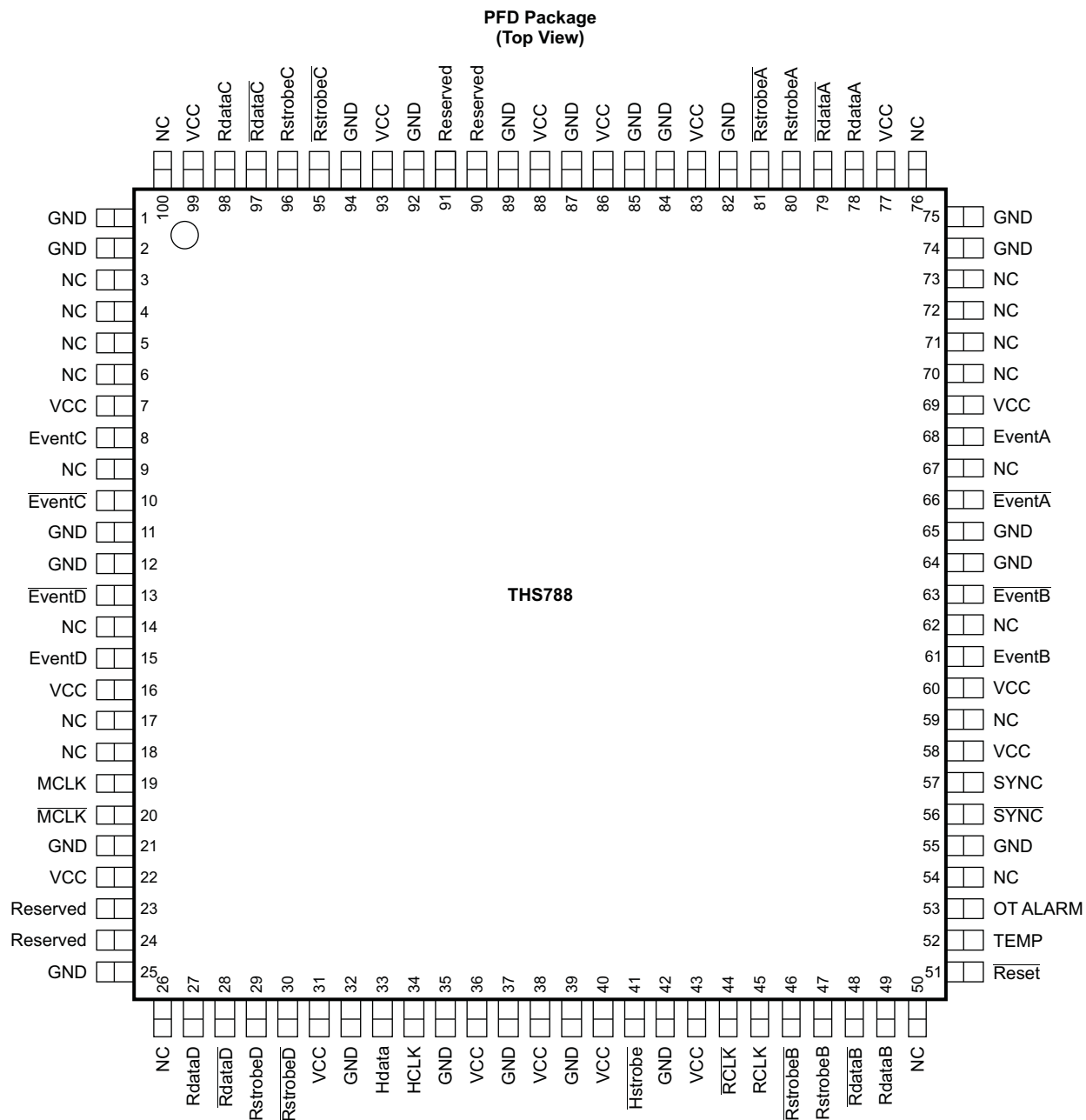
Figure 2. Pinout Diagram
