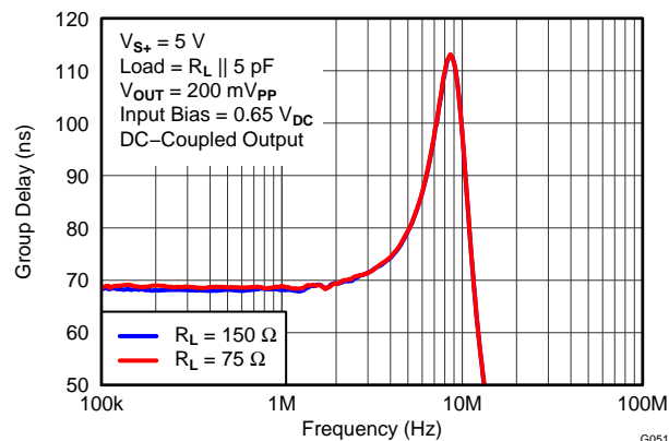
Figure 59. SD GROUP DELAY vs FREQUENCY
