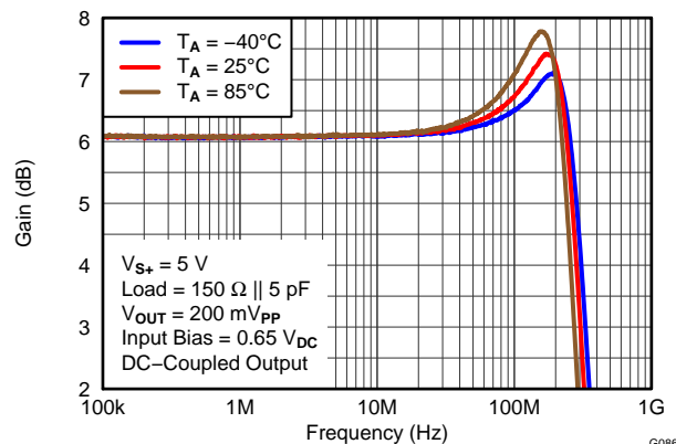
Figure 101. HD BYPASS SMALL-SIGNAL GAIN vs FREQUENCY
