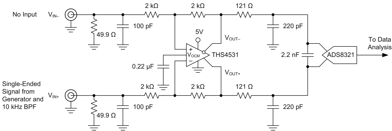
Figure 89. THS4531 and ADS8321 Test Circuit
