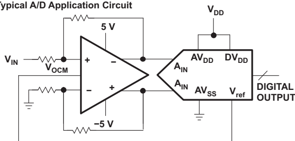
Typical A/D Application Circuit
