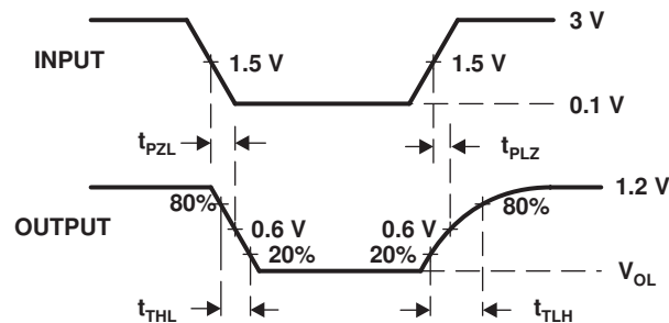
Figure 3. Waveform 1 – Propagation Delay and Transition Times for B Side to A Side
