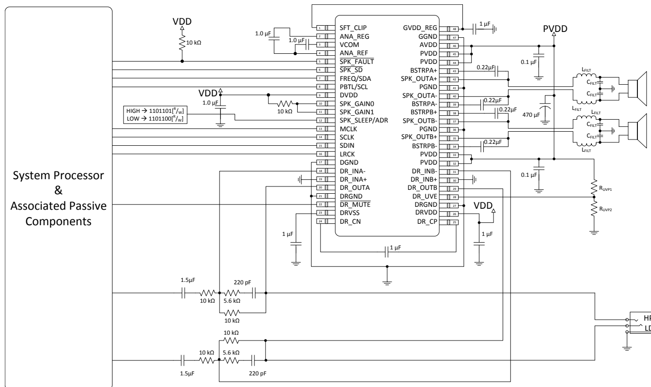
Figure 44. Stereo BTL using Software Control
