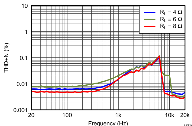
Figure 26. THD+N vs Frequency with PVDD = 12 V, P_{\text{OSP}_K} = 1\text{ W}
