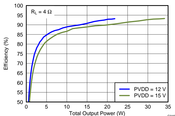
Figure 37. Efficiency vs Output Power
