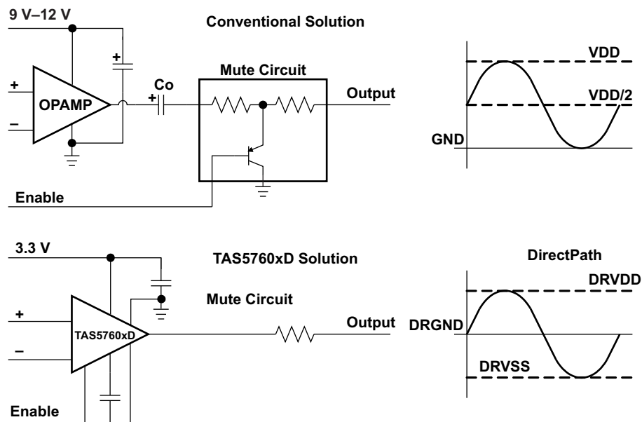
Figure 48. Conventional and DirectPath Line Drivers
