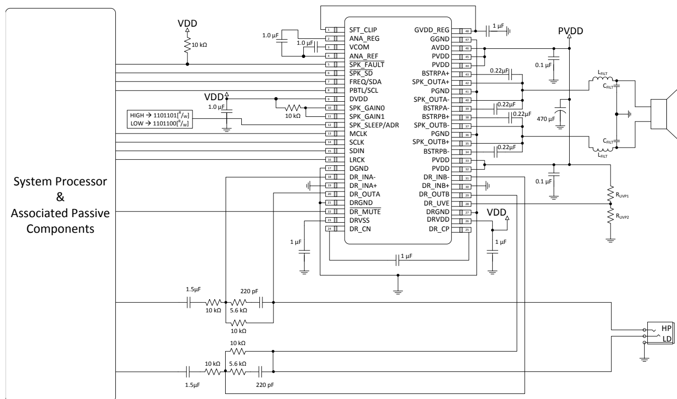
Figure 46. Mono PBTL using Software Control
