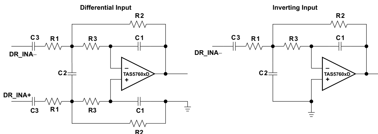
Figure 49. Second-Order Active Low-Pass Filter
