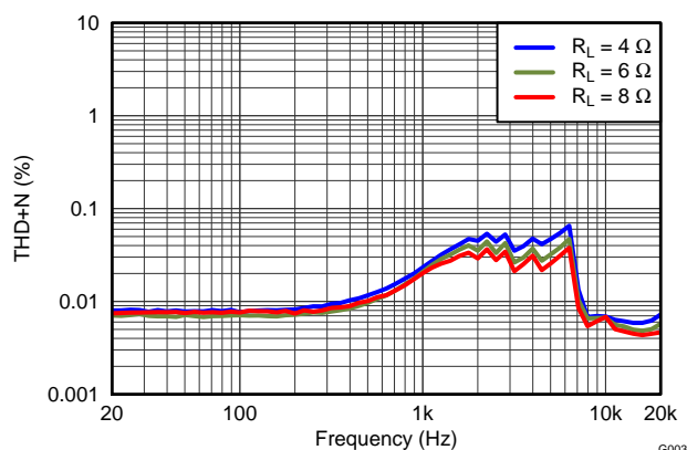
Figure 16. THD+N vs Frequency with PVDD = 12 V, P_{\text{OSPK}} = 1 \text{ W}
