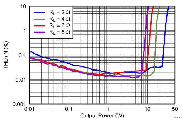
Figure 35. THD+N vs Output Power with PVDD = 12 V
