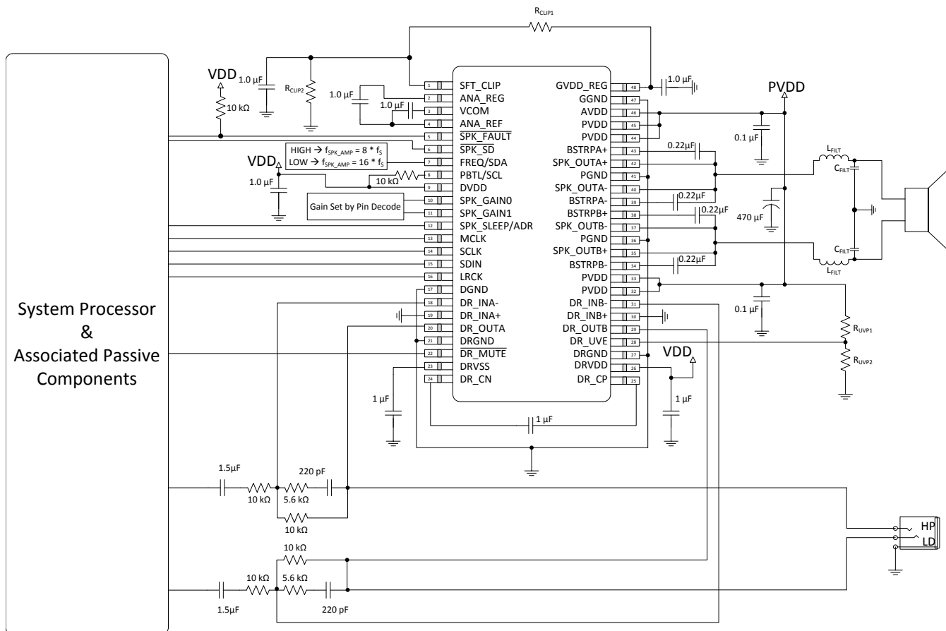
Figure 47. Mono PBTL using Hardware Control
