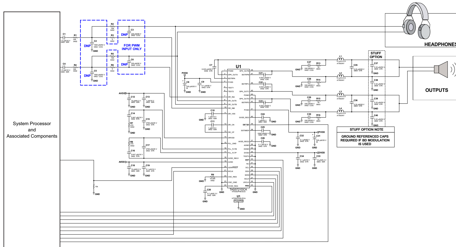
Figure 2. Typical Application Circuit for Mono (PBTL) Configuration
