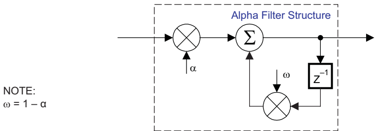
Figure 67. DRC Structure
