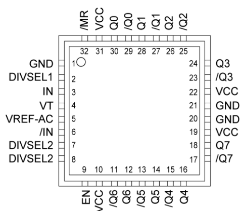
32-Pin QFN
