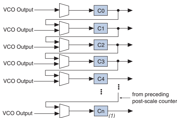
Figure 5-30. Counter Cascading
