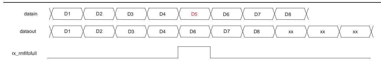
Figure 1-70. Rate Match FIFO Full Condition in Basic Single-Width Mode
