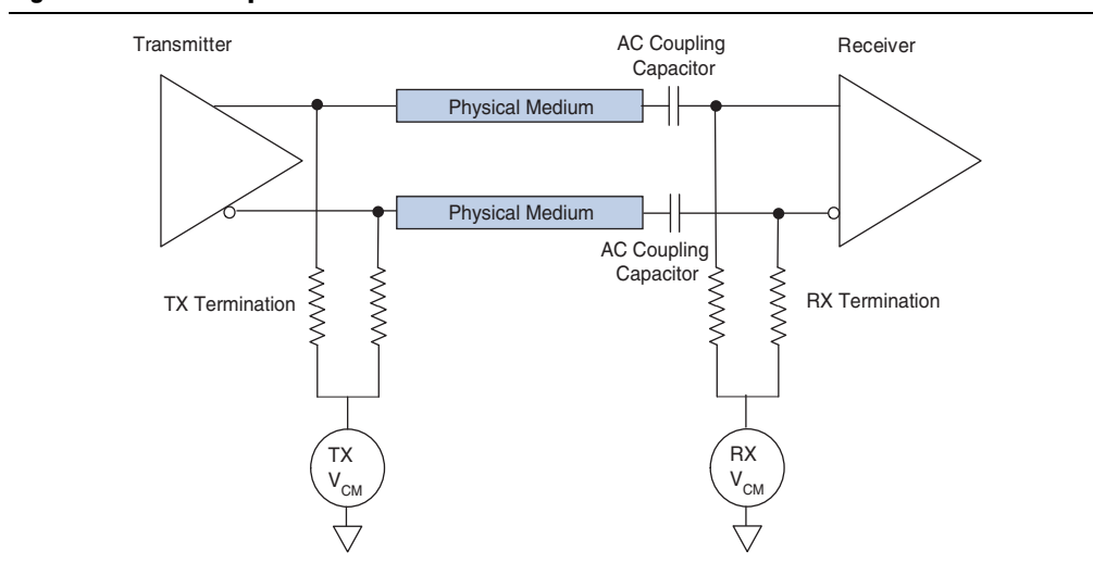
Figure 1-33. AC-Coupled Link
