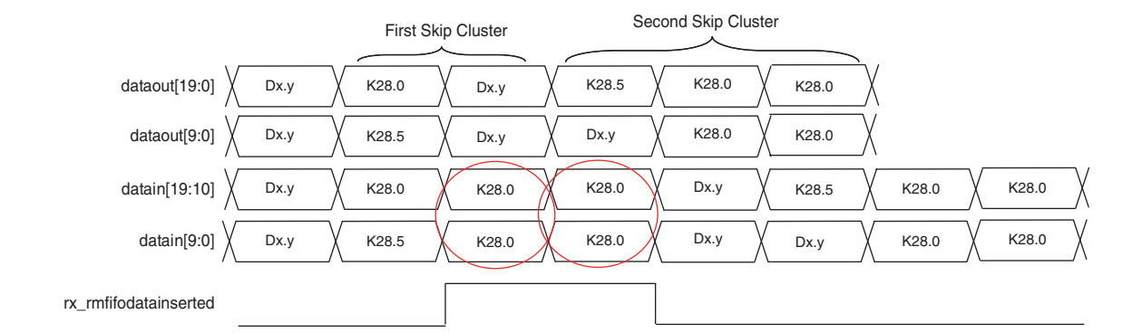
Figure 1-73. Rate Match Insertion in Basic Double-Width Mode
