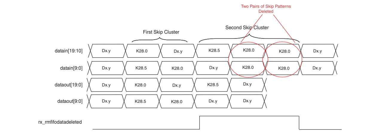
Figure 1-72. Rate Match Deletion in Basic Double-Width Mode
