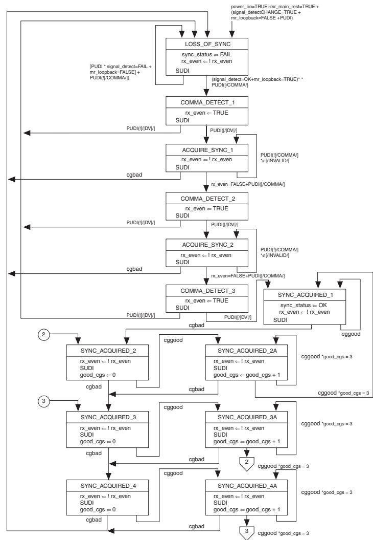
Figure 1-136. Synchronization State Machine in GIGE Mode (1)
