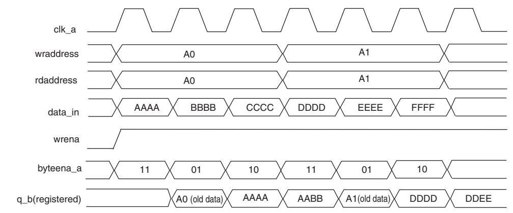
Figure 3-19. MLABs Mixed-Port Read-During-Write: Old Data Mode
