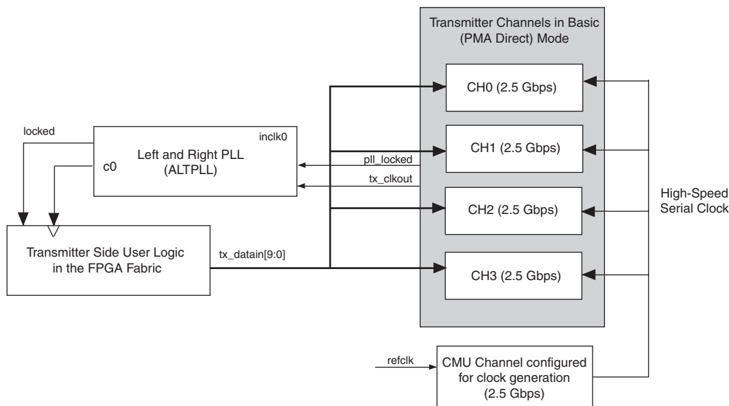
Figure 4-14. Identical Channels
