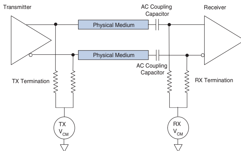
Figure 1-37. AC-Coupled Link
