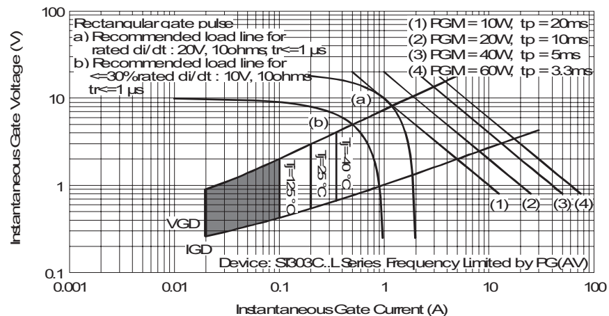
Fig. 17 - Gate Characteristics
