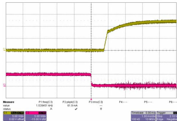
Figure 6. Turn-on transient at full rated load current (resistive) with no output capacitor at V_{in}=48\text{V} , triggered via ON/OFF pin. Bottom trace: ON/OFF signal (5V/div.). Top trace: Output voltage (5V/div.). Time scale: 1ms/div.
