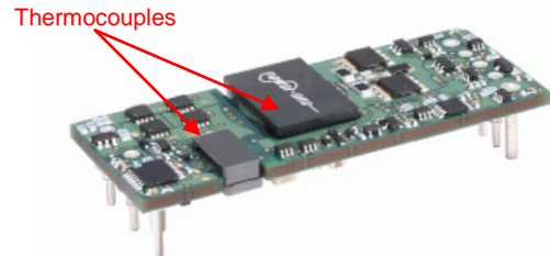
Fig. H: Locations of the thermocouple for thermal testing.
