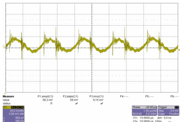
Figure 9. Output voltage ripple (20 mV/div.) at full rated load current into a resistive load with C_o = 10\text{ }\mu\text{F} tantalum + 1µF ceramic and V_{in} = 48\text{V} . Time scale: 1µs/div.
