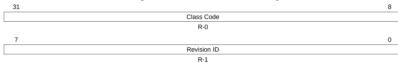
Figure 17-75. CLASSCODE_REVID Register
