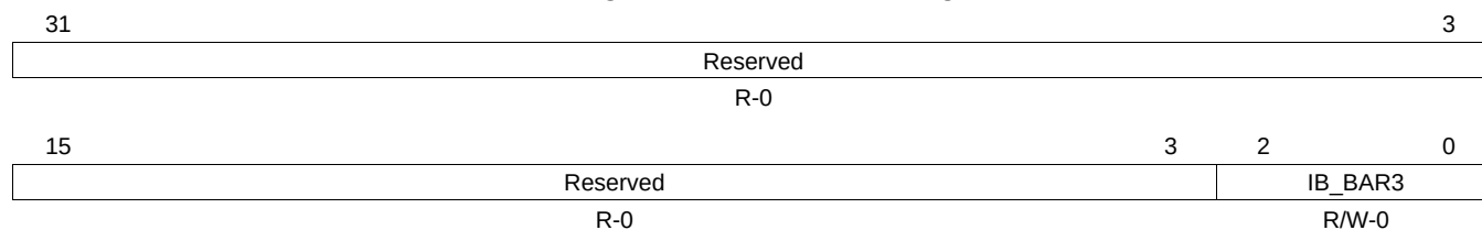
Figure 17-64. IB_BAR3 Register
