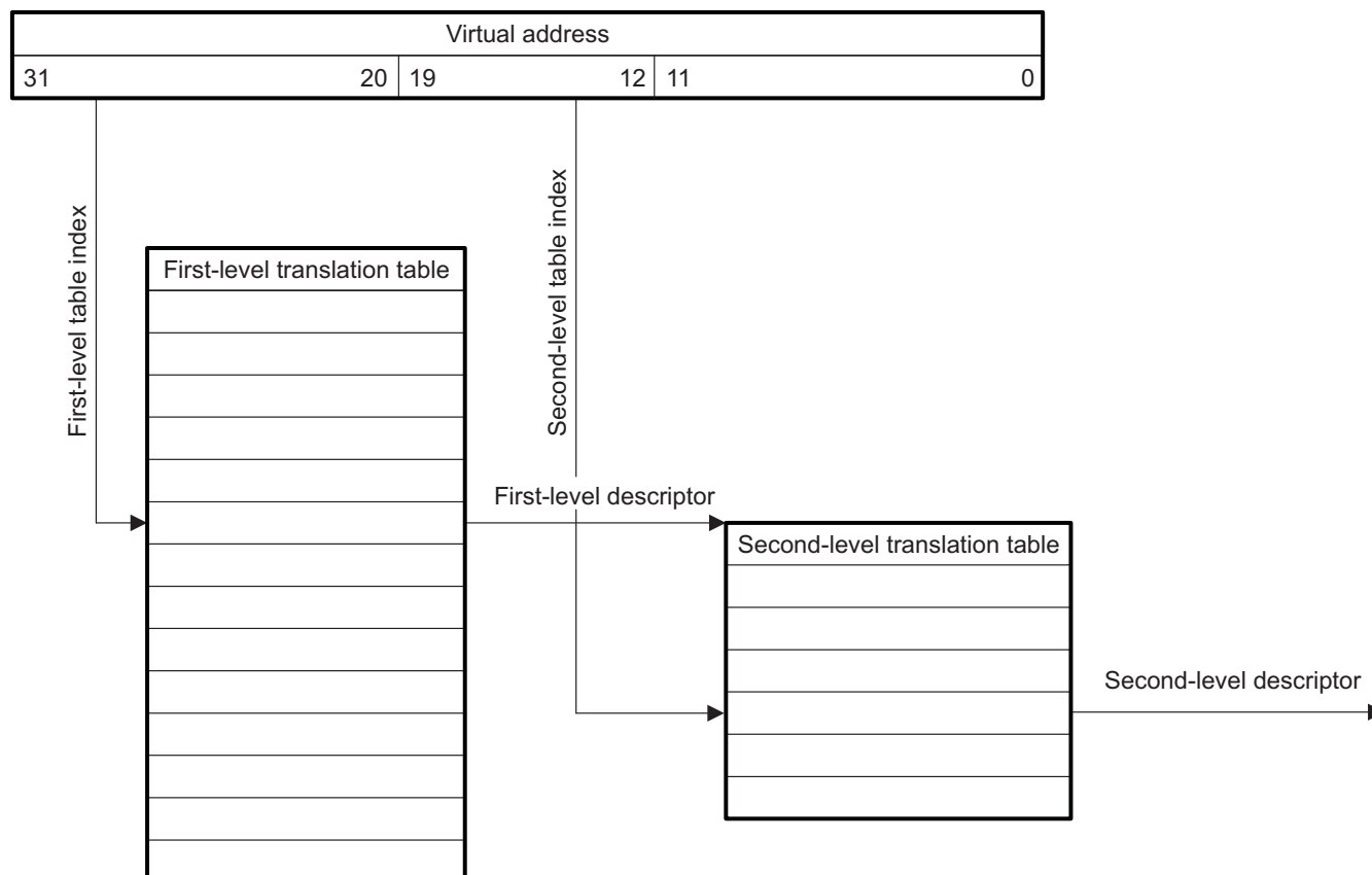
Figure 1-20. Two-Level Translation
