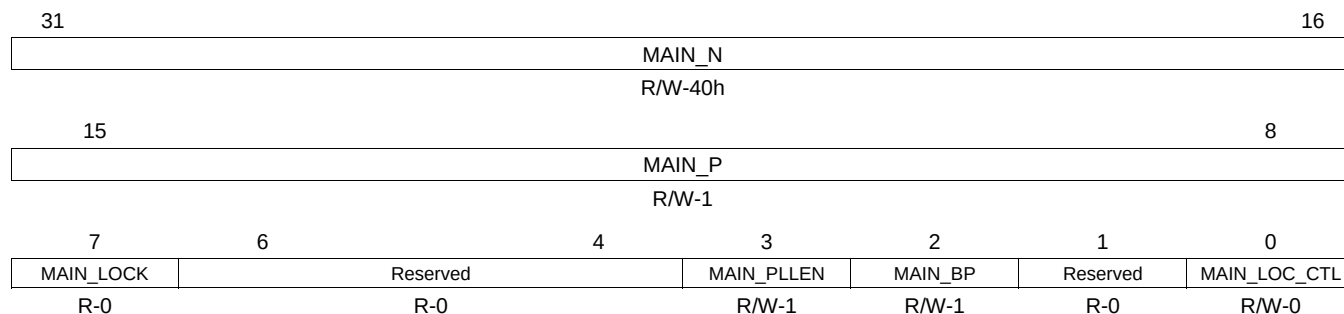
Figure 1-120. Main PLL Control Register (MAINPLL_CTRL)
