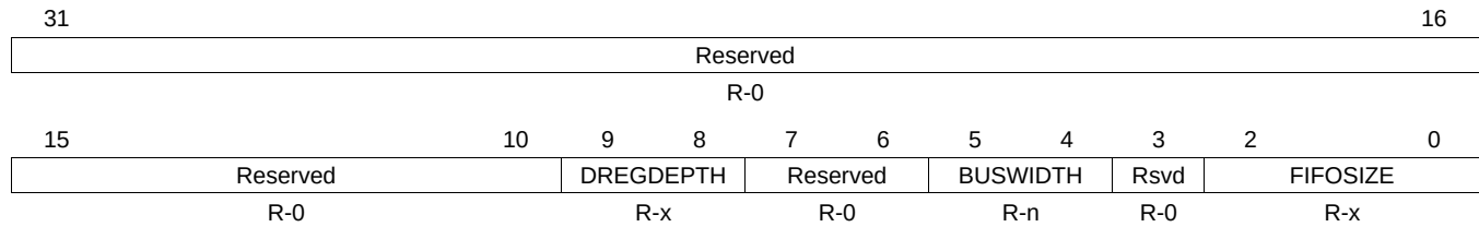
Figure 5-102. EDMA3TC Configuration Register (TCCFG)
