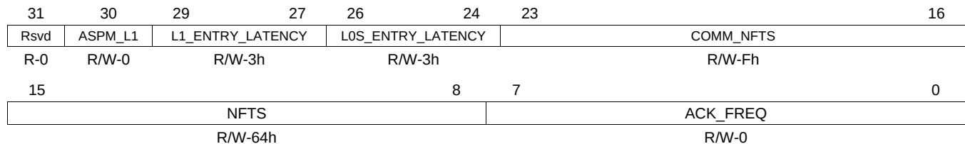
Figure 17-139. ACK_FREQ Register
