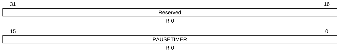
Figure 6-65. Receive Pause Timer Register (RXPAUSE)
