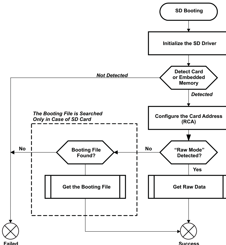
Figure 25-17. SD Booting
