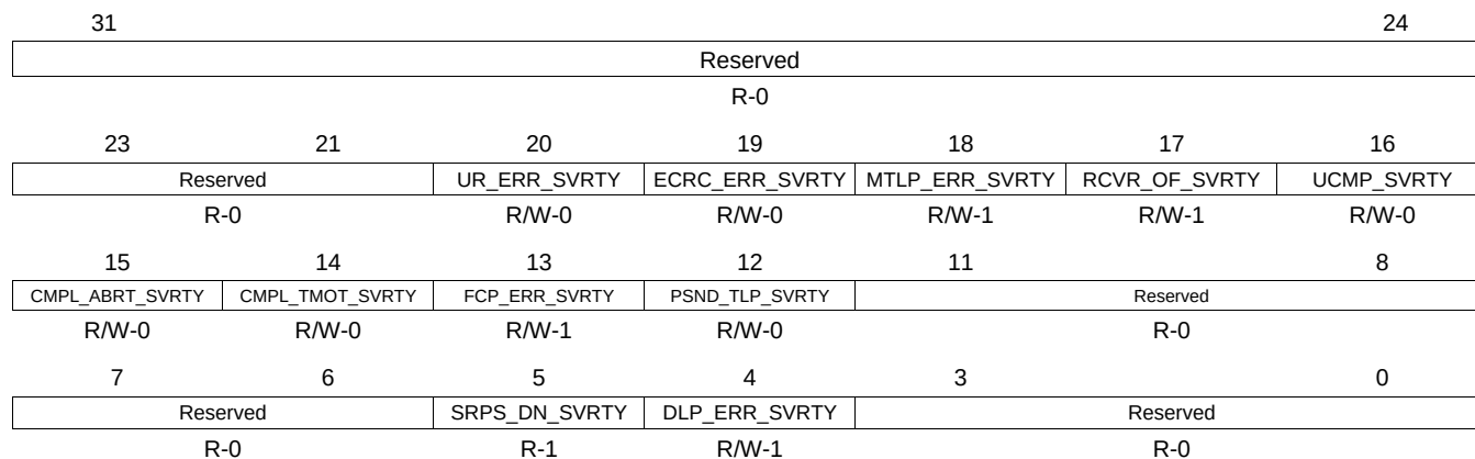
Figure 17-119. PCIE_UNCERR_SVRTY Register
