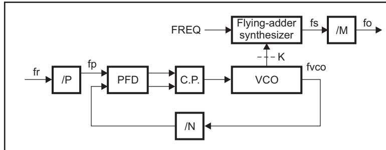
Figure 1-69. Flying Adder PLL
