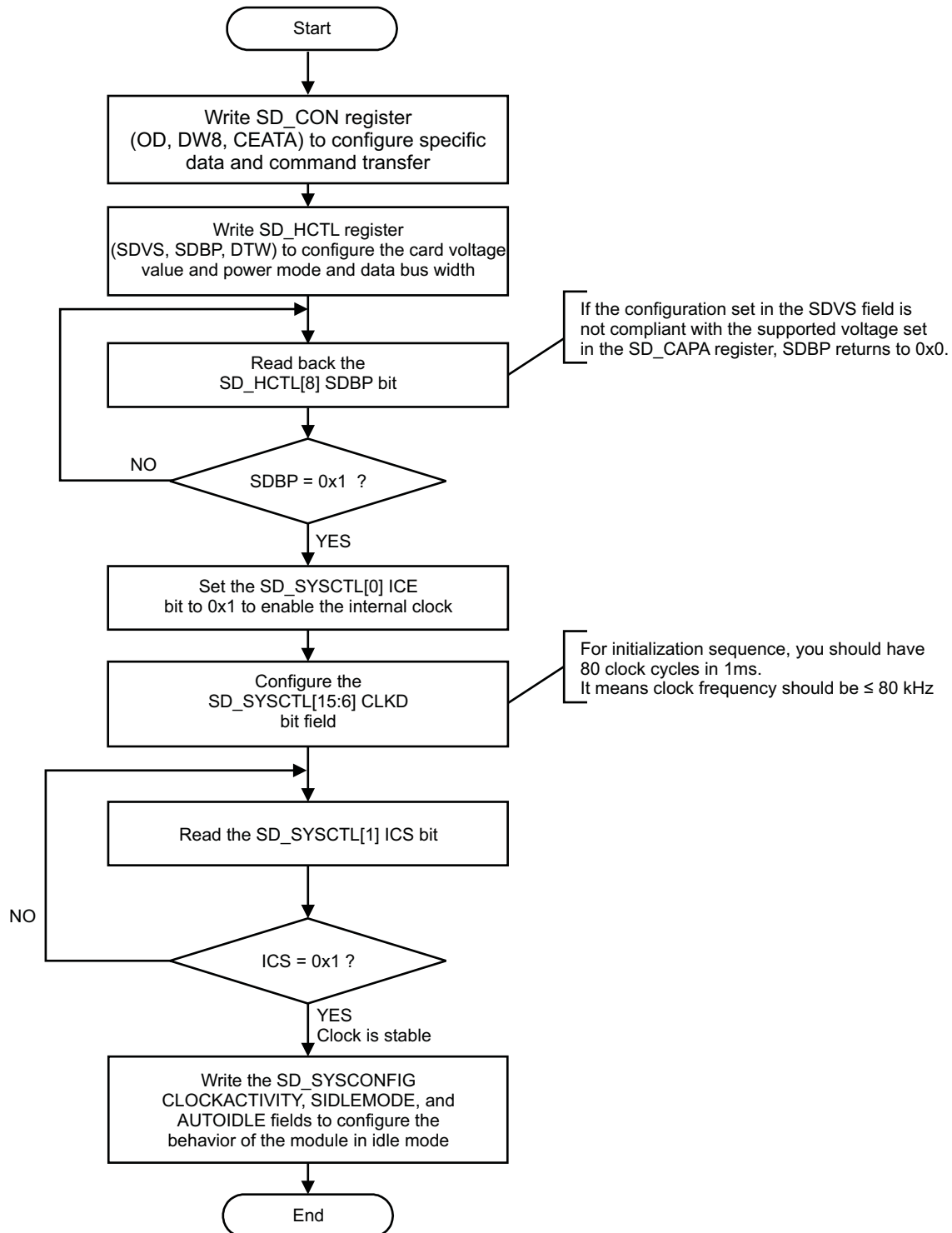
Figure 13-26. SD/SDIO Controller Bus Configuration Flow
