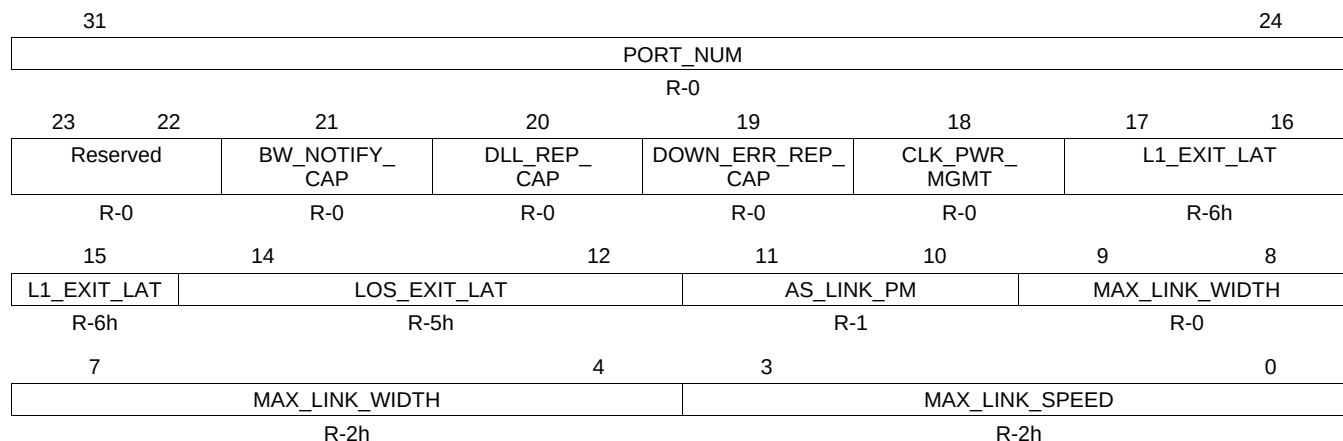
Figure 17-107. LINK_CAP Register
