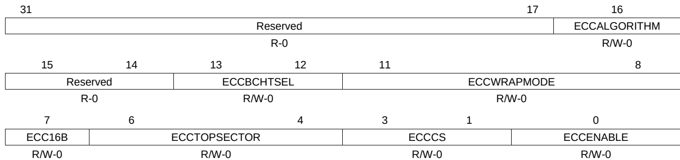
Figure 9-75. GPMC_ECC_CONFIG
