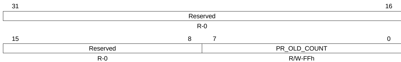
Figure 7-17. Peripheral Bus Burst Priority Register (PBBPR)
