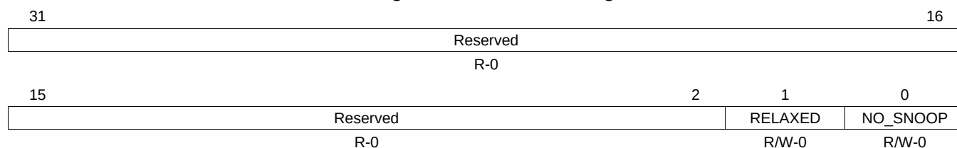
Figure 17-17. TLPCFG Register
