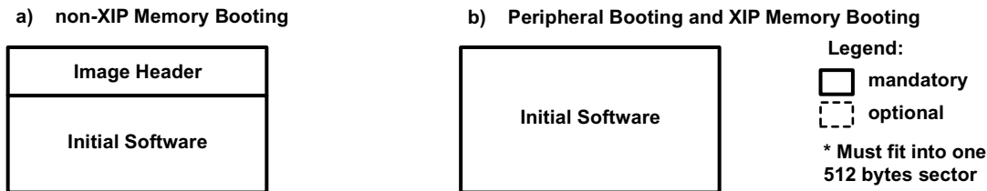
Figure 25-24. Image Formats
