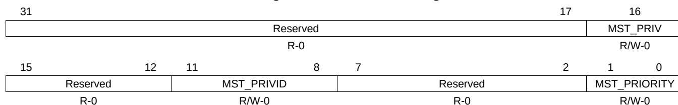
Figure 17-24. PRIORITY Register
