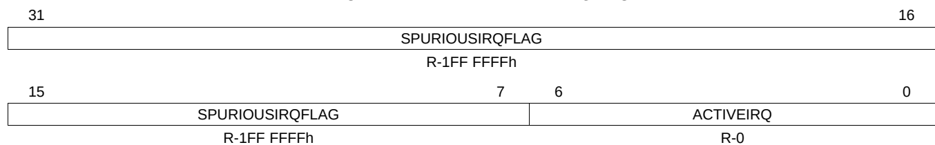
Figure 12-9. INTCPS_SIR_IRQ Register
