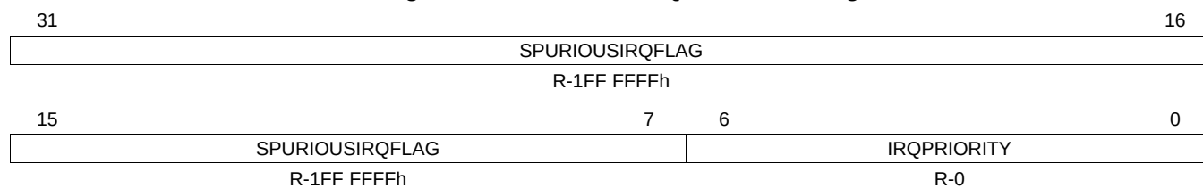
Figure 12-14. INTCPS_IRQ_PRIORITY Register
