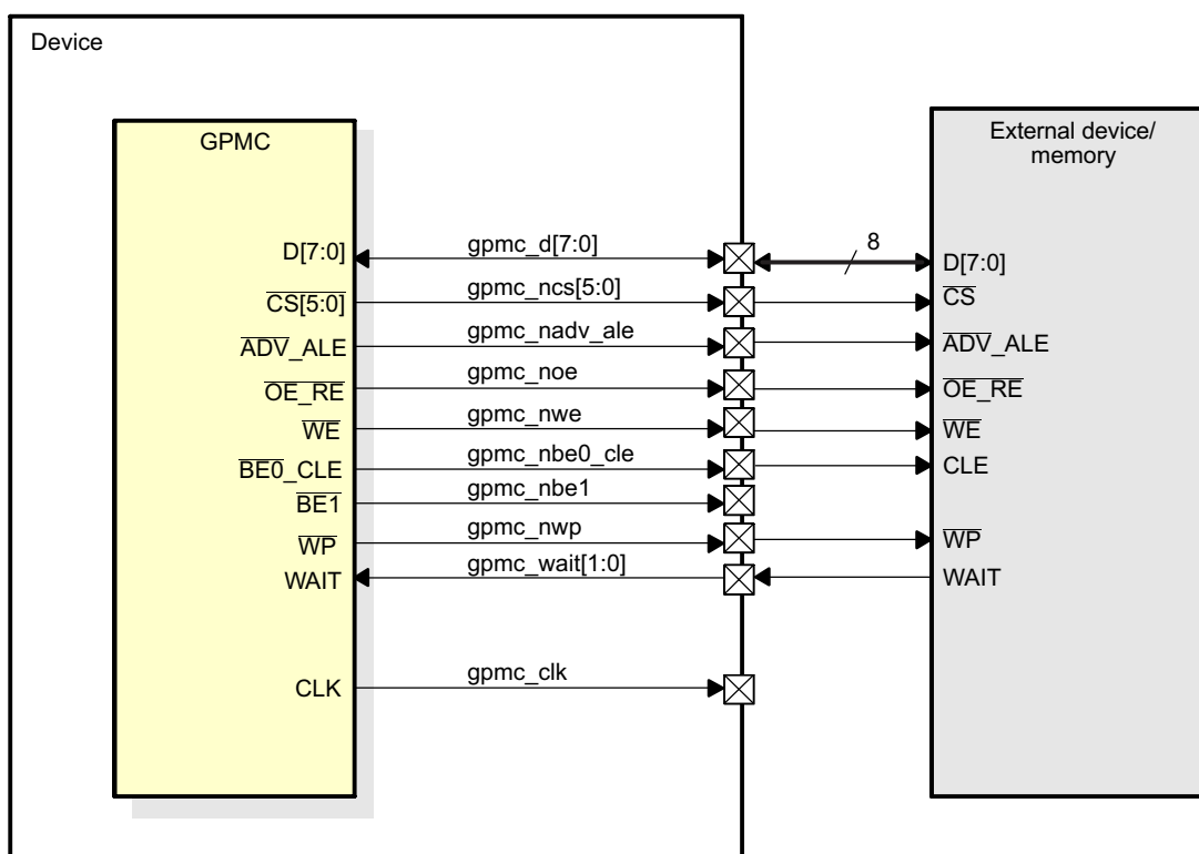
Figure 9-4. GPMC to 8-Bit NAND Device
