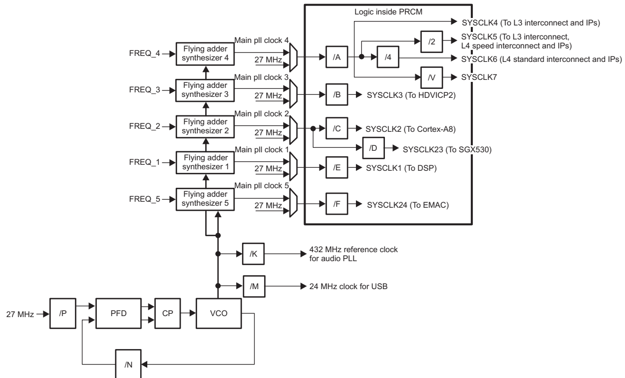
Figure 1-70. Main PLL Structure
