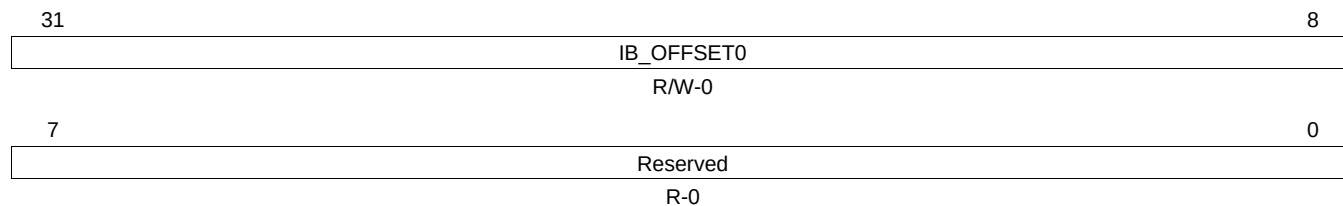
Figure 17-55. IB_OFFSET0 Register
