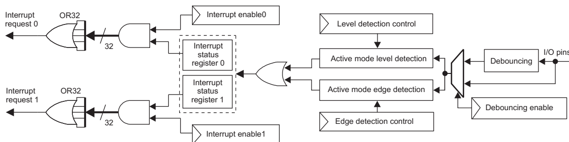
Figure 8-2. Synchronous Path Block Diagram
