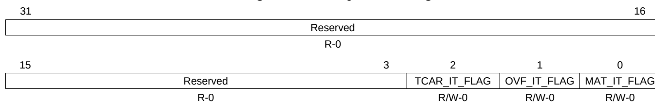
Figure 21-12. IRQSTATUS Register
