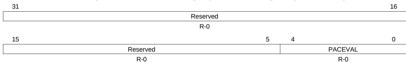
Figure 6-64. Transmit Pacing Algorithm Test Register (TPACETEST)
