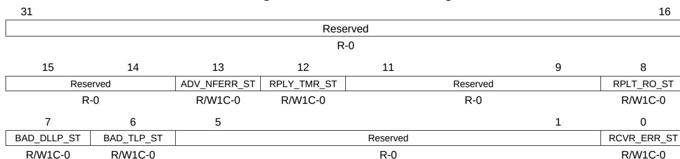
Figure 17-120. PCIE_CERR Register
