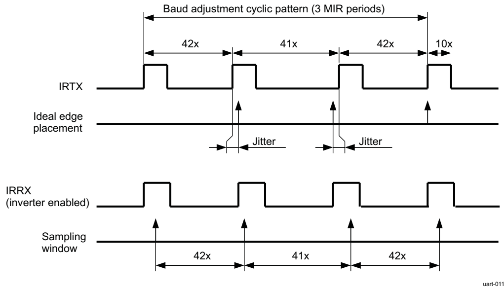
Figure 23-9. MIR Baud Rate Adjustment Mechanism
