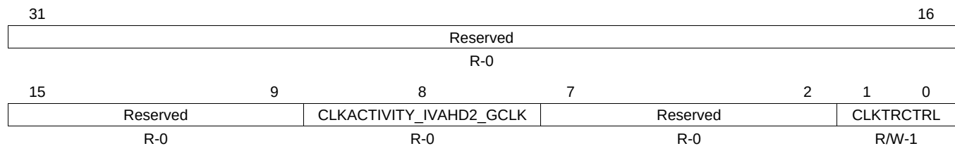
Figure 18-77. CM_IVAHD2_CLKSTCTRL Register
