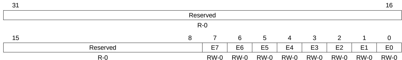
Figure 5-57. QDMA Region Access Enable for Region m (QRAEm) 32-bit, 2 Rows
