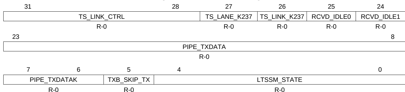
Figure 17-145. DEBUG0 Register
