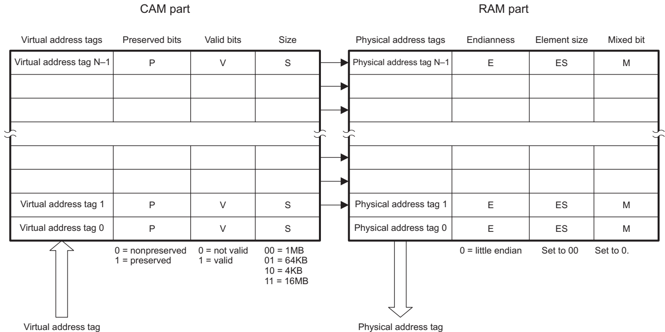
Figure 1-24. TLB-Entry Structure
