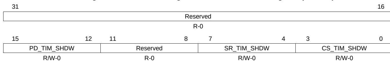
Figure 7-16. Power Management Control Shadow Register (PMCSR)
