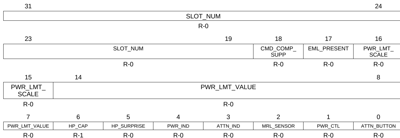
Figure 17-109. SLOT_CAP Register
