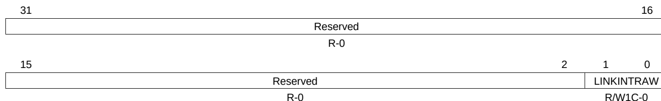
Figure 6-79. MDIO Link Status Change Interrupt (Unmasked) Register (LINKINTRA W )
