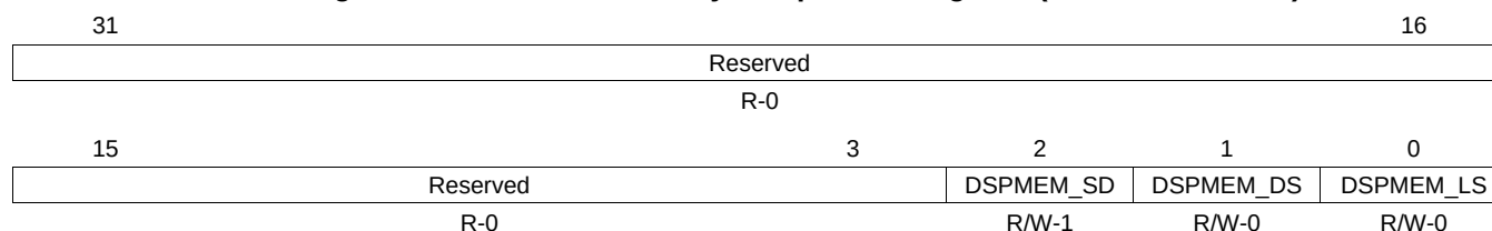
Figure 1-181. DSP L2 Memory Sleep Mode Register (DSPMEM_SLEEP)
