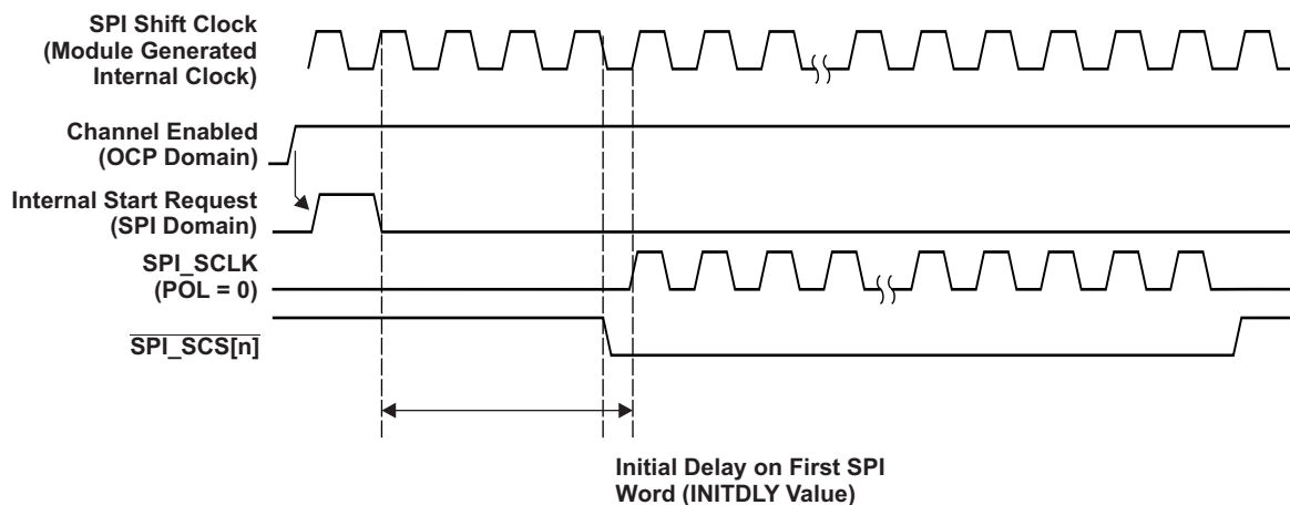
Figure 16-20. Master Single Channel Initial Delay
