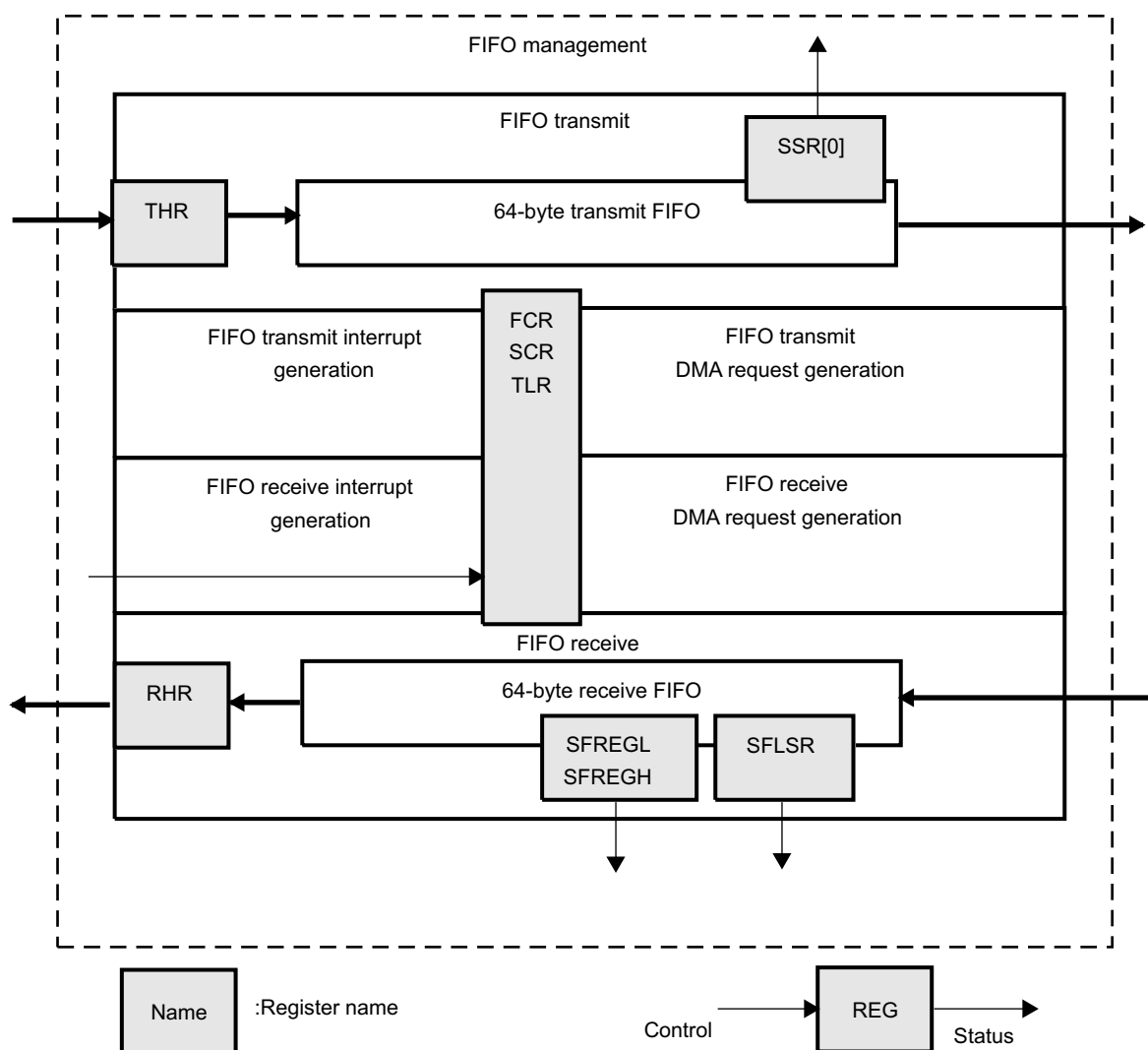
Figure 23-18. FIFO Management
