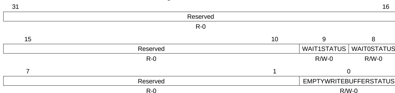
Figure 9-60. GPMC_STATUS
