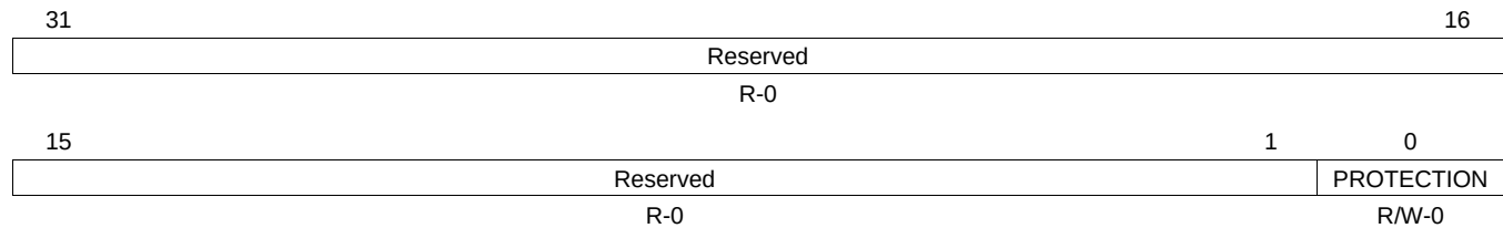
Figure 12-12. INTCPS_PROTECTION Register
