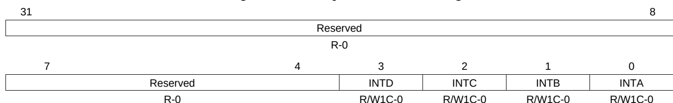
Figure 17-41. IRQ_ENABLE_CLR Register
