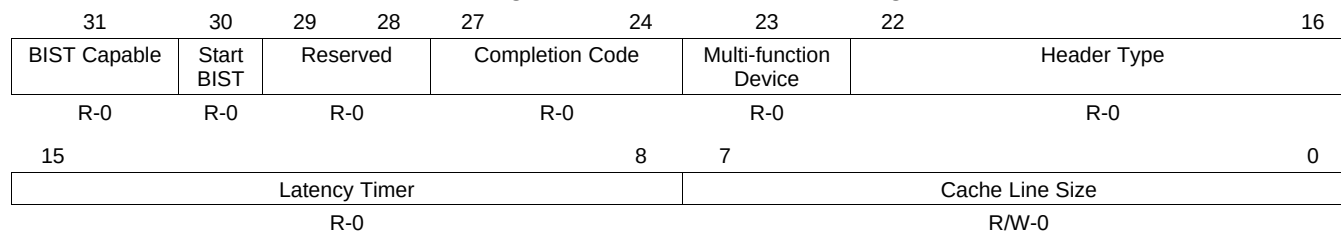
Figure 17-76. BIST_HEADER Register
