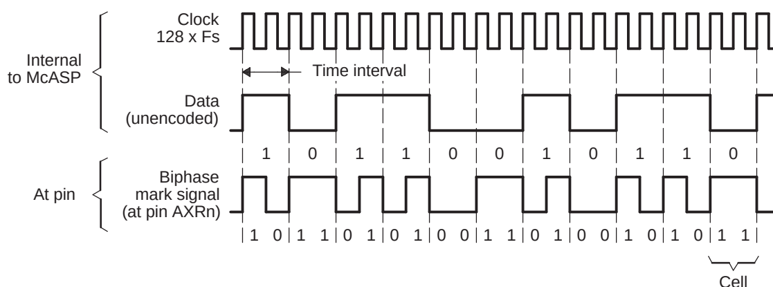
Figure 14-10. Biphasemark Code (BMC)
