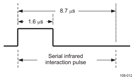
Figure 23-10. Serial Infrared Interaction Pulse (SIP)
