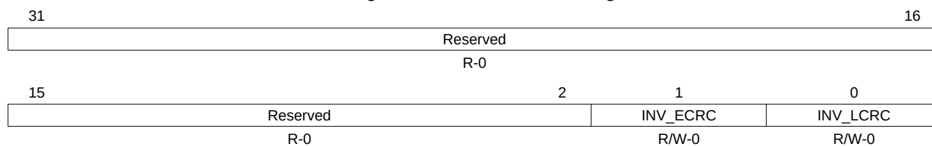
Figure 17-23. DIAG_CTRL Register
