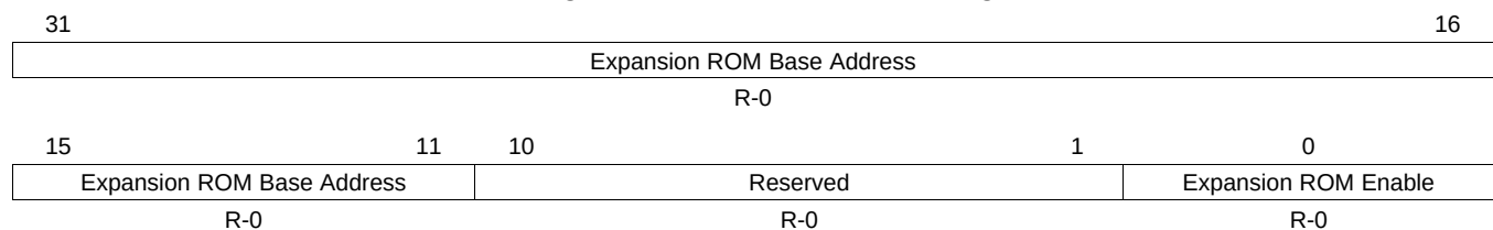
Figure 17-87. EXPNSN_ROM Register
