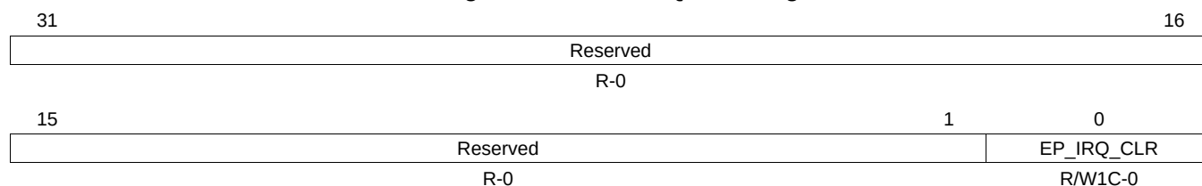
Figure 17-28. EP_IRQ_CLR Register
