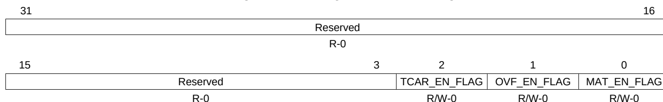
Figure 21-13. IRQENABLE_SET Register
