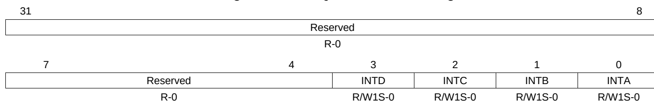
Figure 17-38. IRQ_STATUS_RAW Register
