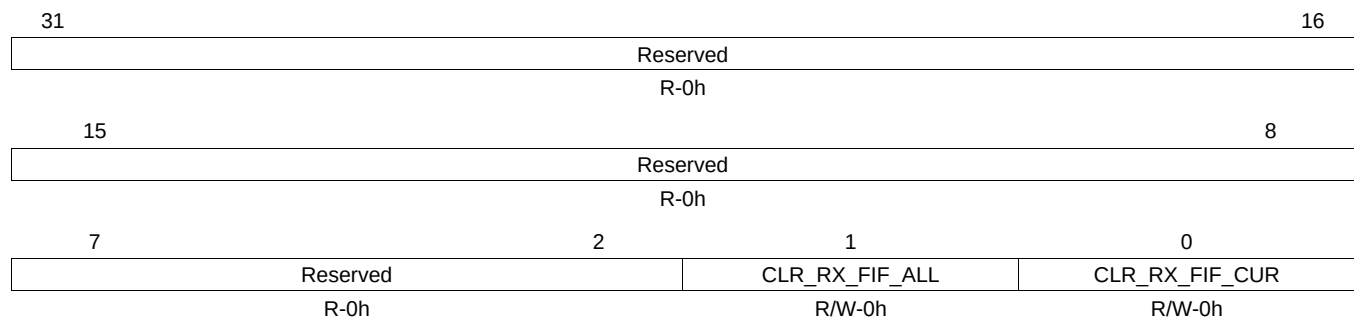
Figure 10-226. CEC RX Control Register (CEC_RX_CONTROL)
