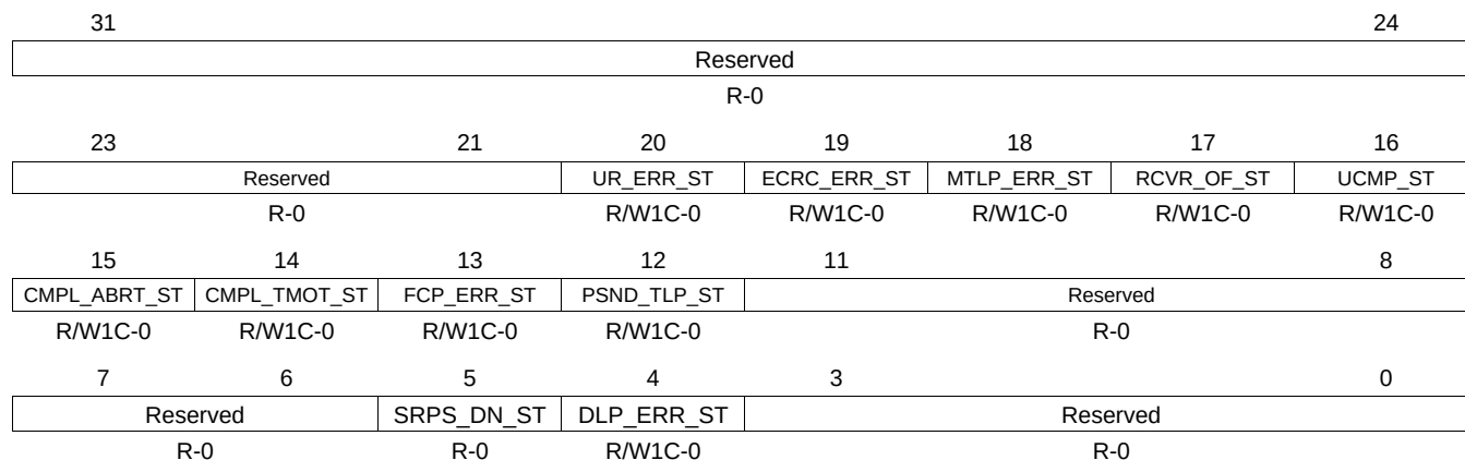
Figure 17-117. PCIE_UNCERR Register
