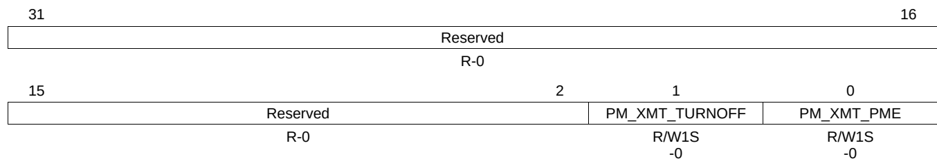
Figure 17-19. PMCMD Register
