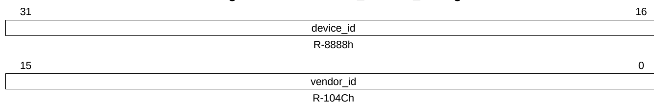
Figure 17-73. VENDOR_DEVICE_ID Register
