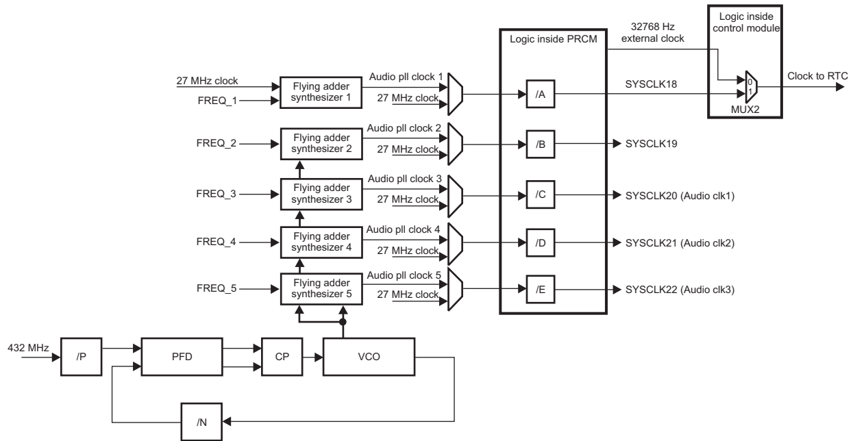
Figure 18-9. Audio FAPLL Interface to PRCM
