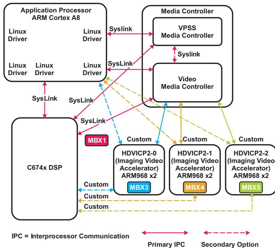
Figure 1-76. IPC Overview Diagram
