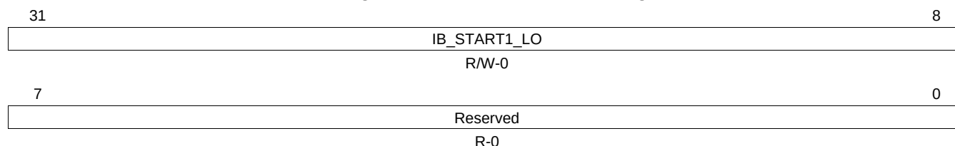
Figure 17-57. IB_START1_LO Register
