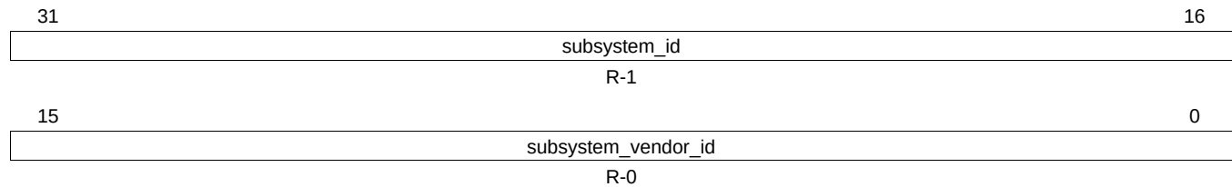
Figure 17-86. SUBSYS_VNDR_ID Register
