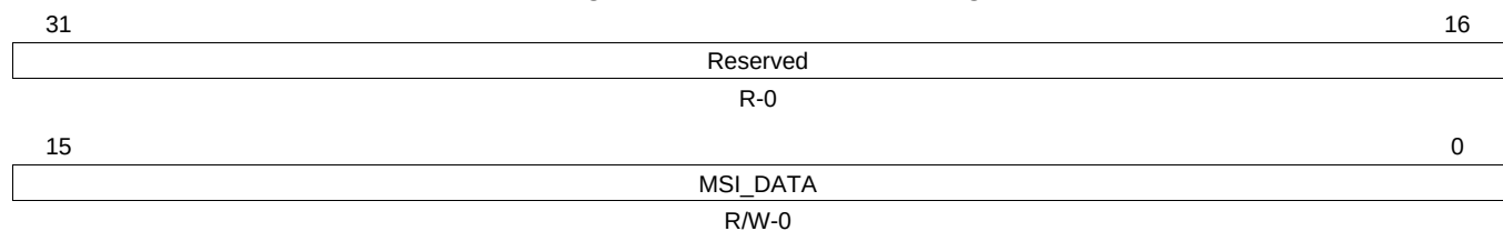
Figure 17-133. MSI_DATA Register
