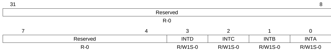
Figure 17-40. IRQ_ENABLE_SET Register
