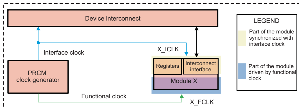
Figure 18-1. Functional and Interface Clocks
