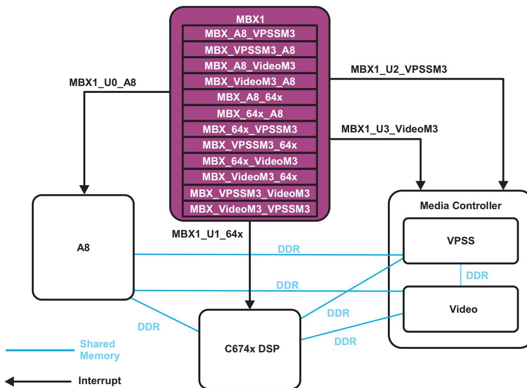
Figure 1-77. System IPCs
