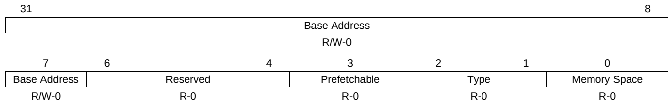
Figure 17-77. BAR0 Register
