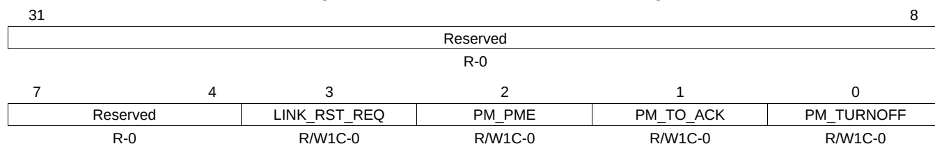
Figure 17-49. PMRST_ENABLE_CLR Register
