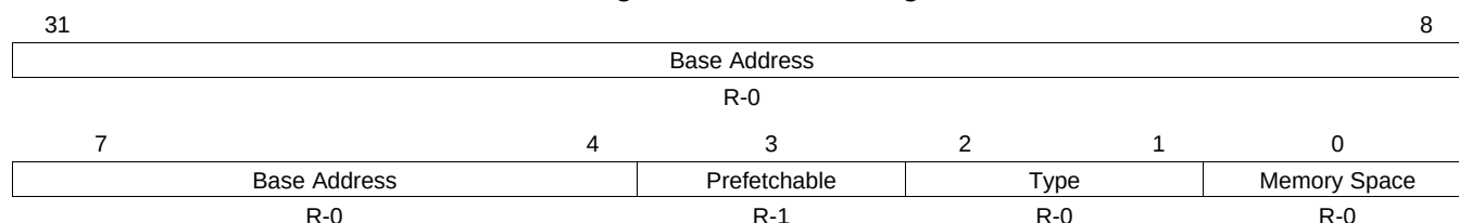
Figure 17-92. BAR1 Register
