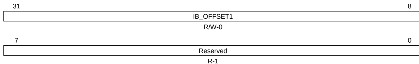
Figure 17-59. IB_OFFSET1 Register
