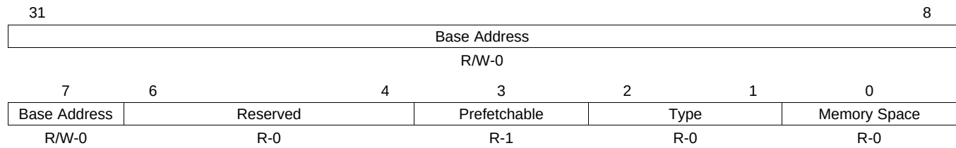
Figure 17-83. BAR4 Register
