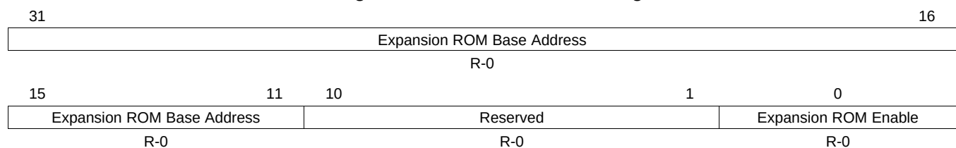
Figure 17-102. EXPNSN_ROM Register
