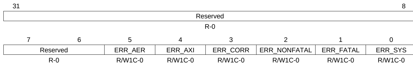
Figure 17-45. ERR_IRQ_ENABLE_CLR Register
