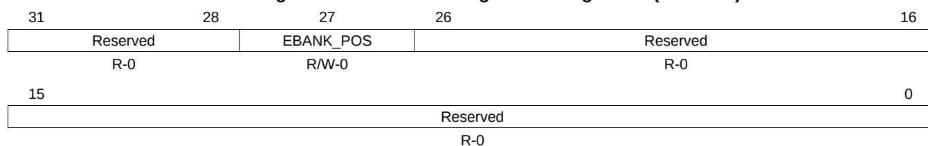
Figure 7-6. SDRAM Configuration Register 2 (SDRCR2)
