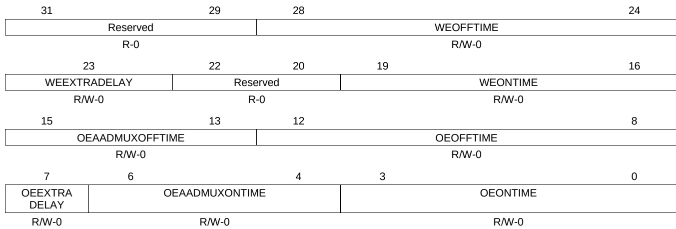
Figure 9-64. GPMC_CONFIG4_i
