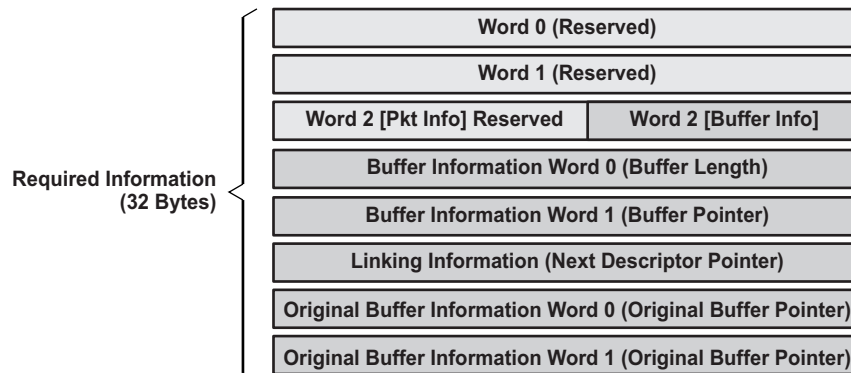
Figure 24-13. Buffer Descriptor (BD) Layout
