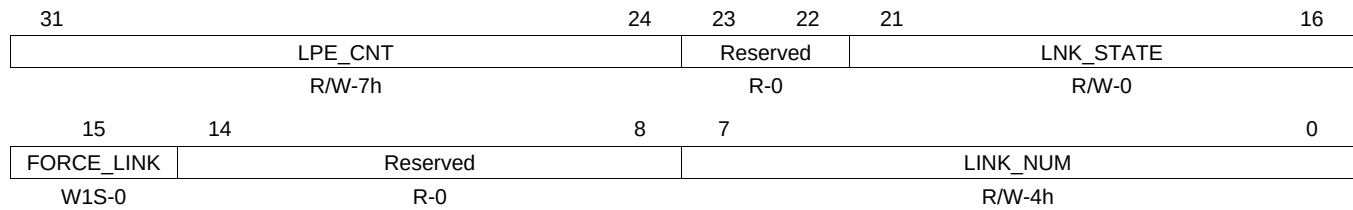
Figure 17-138. PL_FORCE_LINK Register
