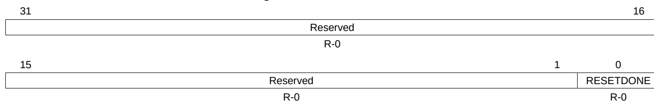
Figure 9-53. GPMC_SYSSTATUS
