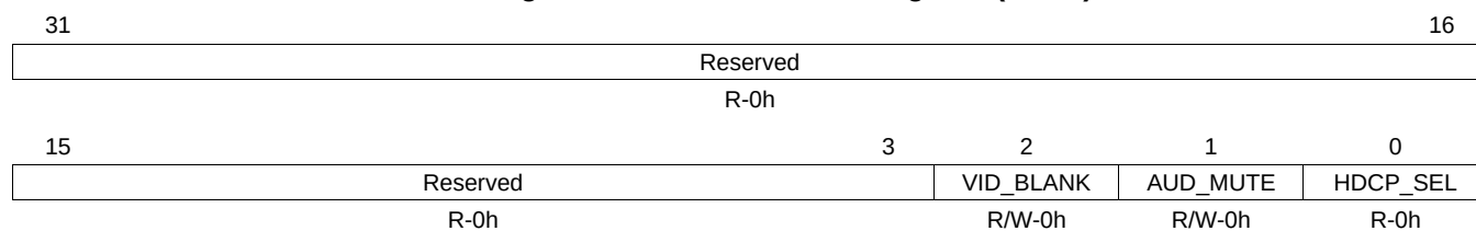
Figure 10-32. Data Control Register (DCTL)
