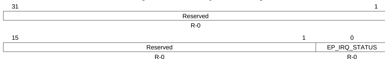
Figure 17-29. EP_IRQ_STATUS Register
