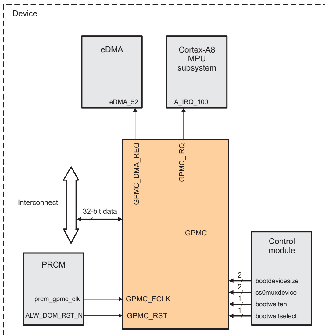
Figure 9-5. GPMC Integration
