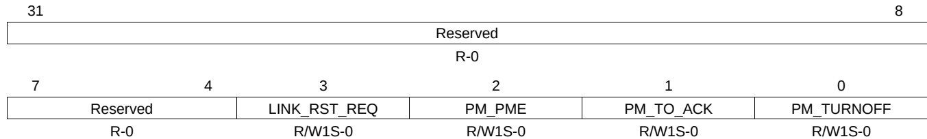
Figure 17-46. PMRST_IRQ_STATUS_RAW Register
