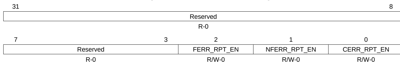
Figure 17-127. RC_ERR_CMD Register
