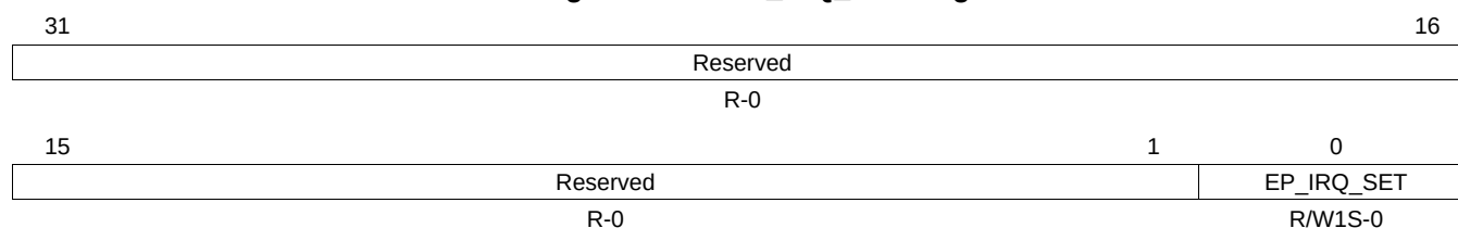
Figure 17-27. EP_IRQ_SET Register
