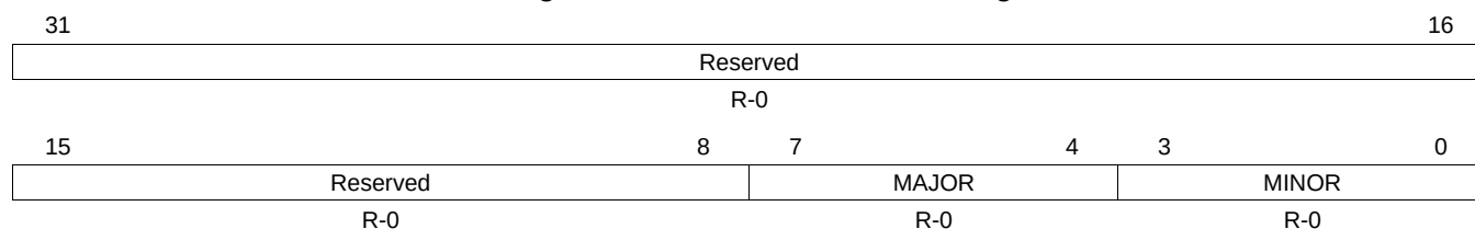
Figure 12-6. INTCPS_REVISION Register
