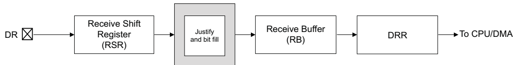
Figure 15-7. McBSP Reception Physical Data Path
