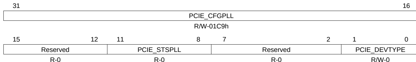
Figure 1-178. PCIE Configuration Register (PCIE_CFG)
