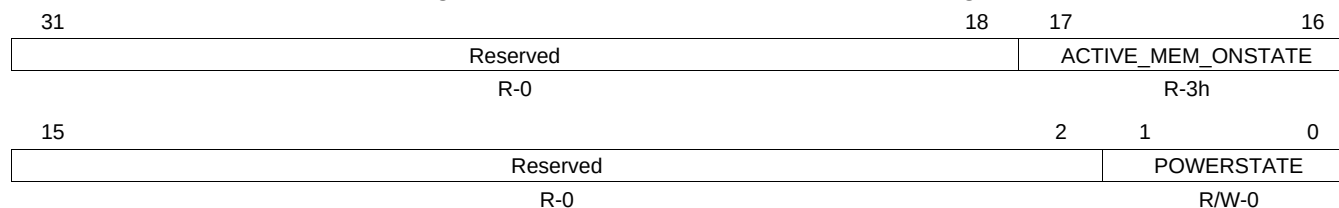
Figure 18-82. PM_ACTIVE_PWRSTCTRL Register
