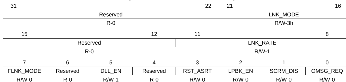
Figure 17-140. PL_LINK_CTRL Register
