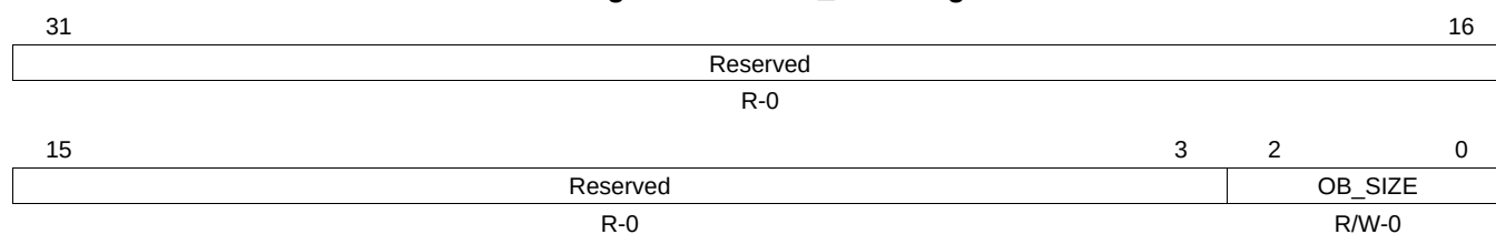
Figure 17-22. OB_SIZE Register
