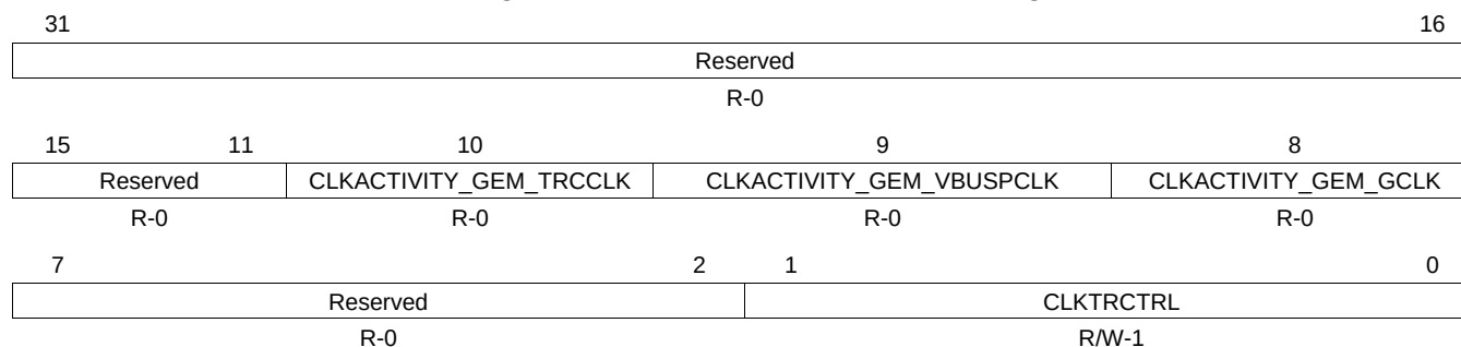
Figure 18-54. CM_GEM_CLKSTCTRL Register
