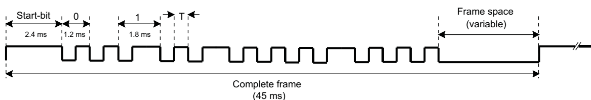
Figure 23-15. SIRC Bit Transmission Example
