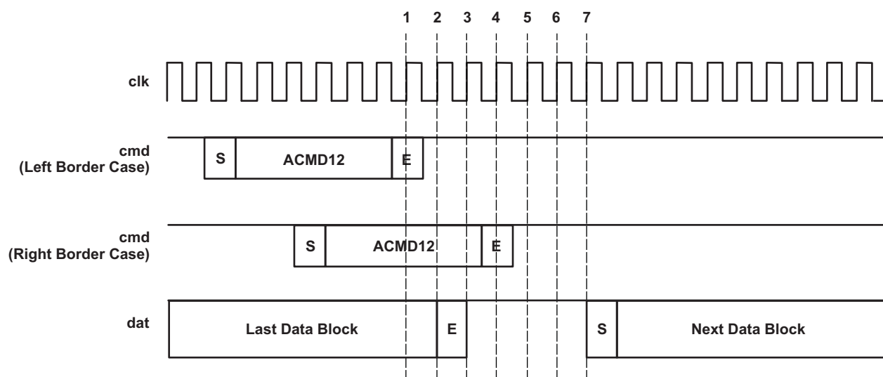
Figure 13-20. Auto CMD12 Timings During Read Transfer
