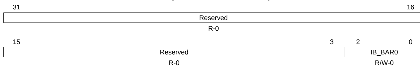
Figure 17-52. IB_BAR0 Register
