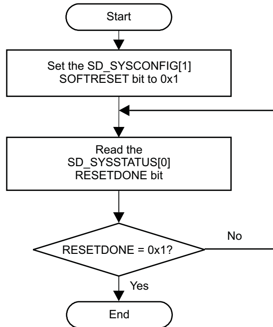
Figure 13-25. SD/SDIO Controller Software Reset Flow
