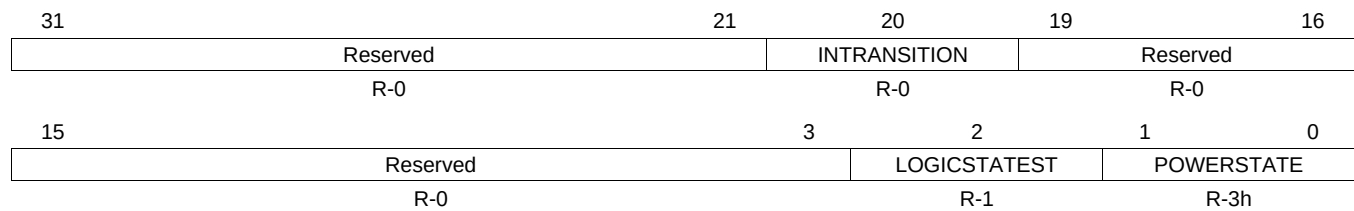
Figure 18-95. PM_IVAHD1_PWRSTST Register
