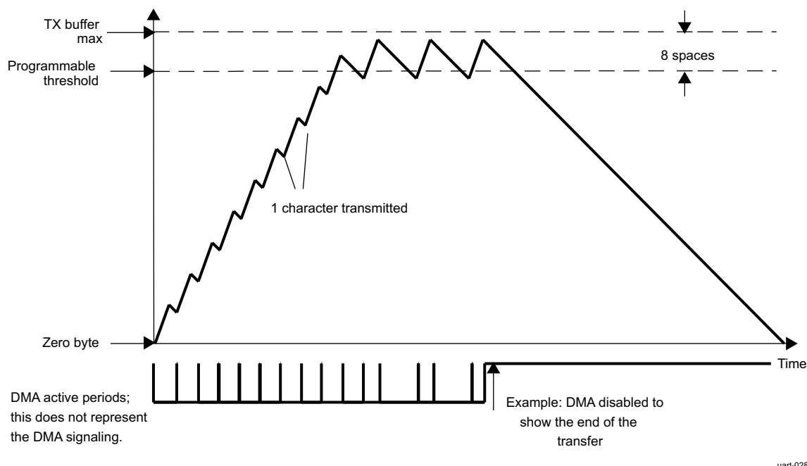
Figure 23-23. Transmit FIFO DMA Request Generation (8 Spaces)
