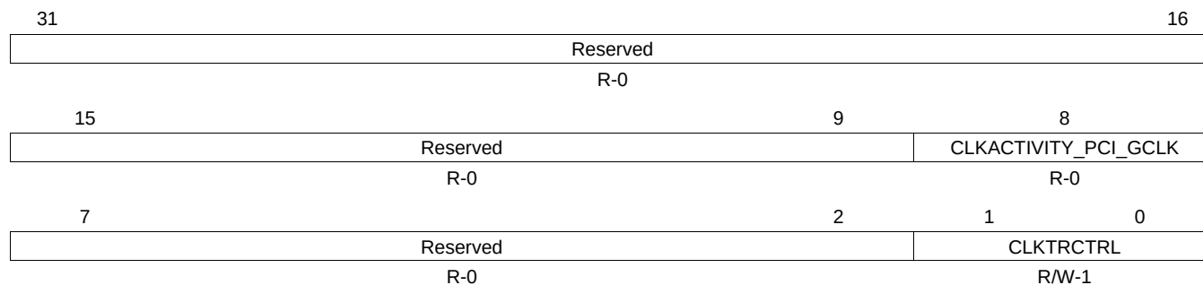
Figure 17-8. CM_DEFAULT_PCI_CLKSTCTRL Register
