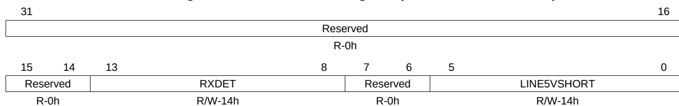
Figure 10-16. Glitch Filter Register (HDMI_WP_DEBOUNCE)
