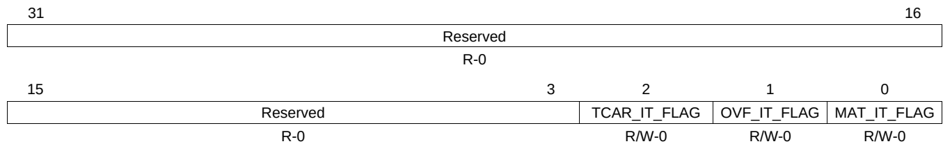
Figure 21-11. IRQSTATUS_RAW Register
