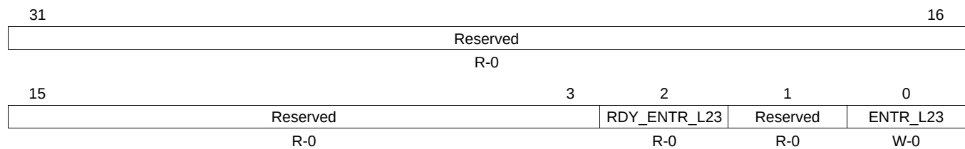
Figure 17-20. PMCFG Register
