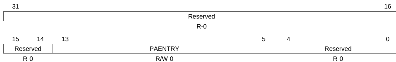
Figure 5-41. DMA Channel Map n Registers (DCHMAP n )
