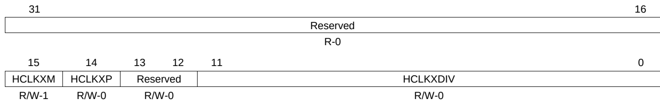
Figure 14-65. Transmit High-Frequency Clock Control Register (AHCLKXCTL)
