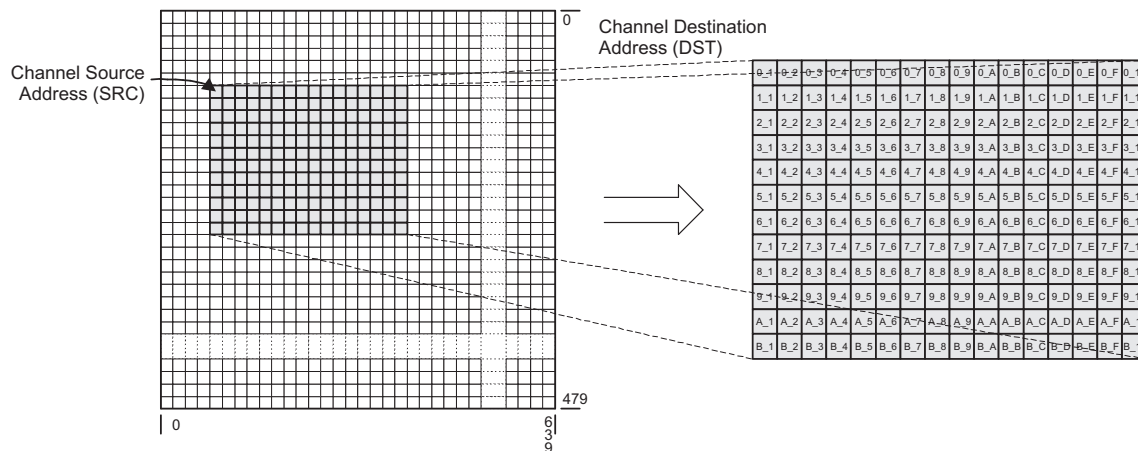
Figure 5-22. Subframe Extraction Example PaRAM Configuration
