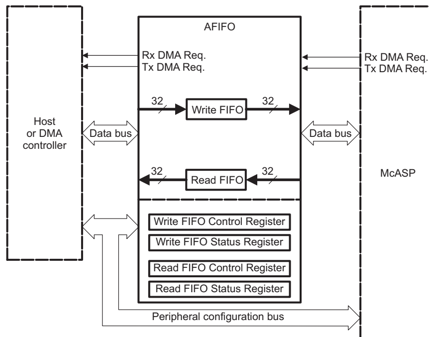
Figure 14-27. McASP Audio FIFO (AFIFO) Block Diagram
