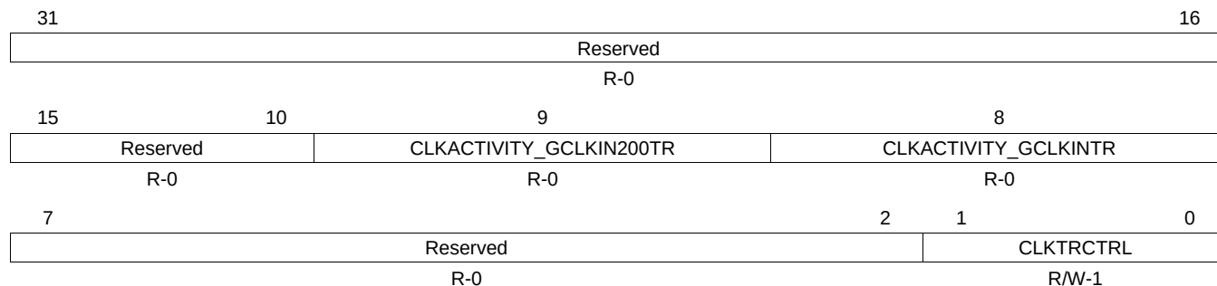
Figure 18-62. CM_DEFAULT_CLKSTCTRL Register
