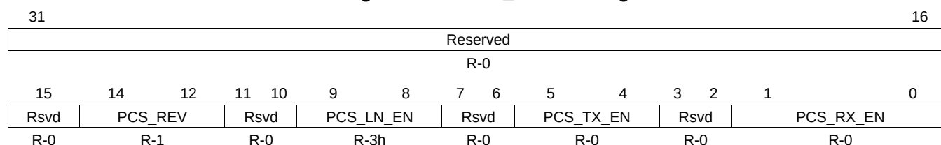
Figure 17-70. PCS_STATUS Register
