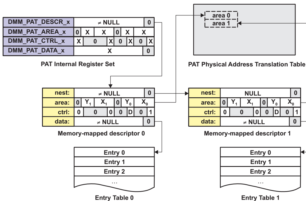
Figure 4-53. DMM Chained Auto-configured Area Refill
