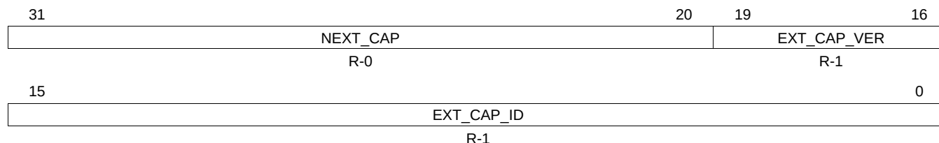
Figure 17-116. PCIE_EXTCAP Register
