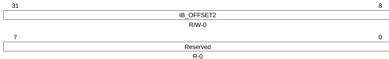
Figure 17-63. IB_OFFSET2 Register
