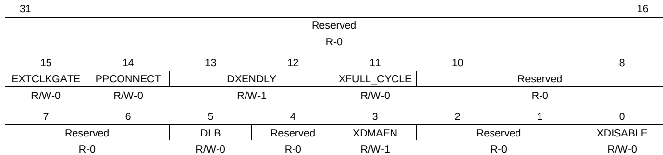
Figure 15-80. McBSP_XCCR_REG
