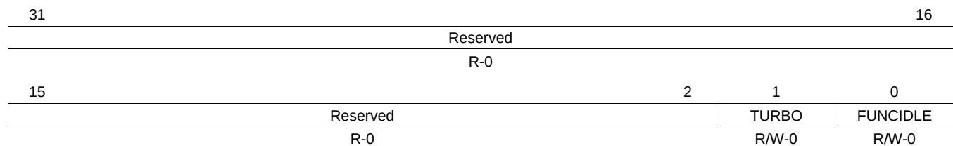
Figure 12-13. INTCPS_IDLE Register
