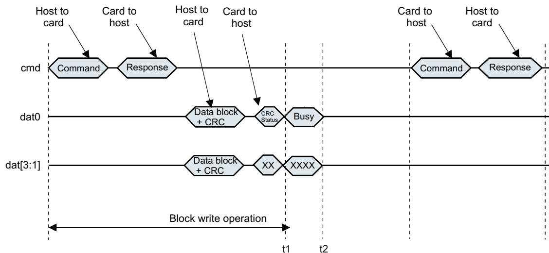
Figure 13-14. Busy Timeout After Write CRC Status
