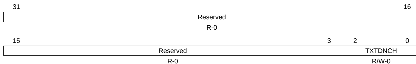
Figure 6-28. Transmit Teardown Register (TXTEARDOWN)
