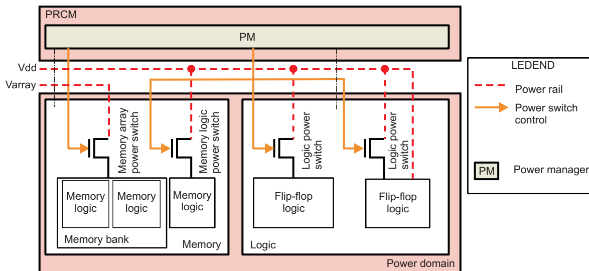
Figure 18-4. Power Domain Block Diagram
