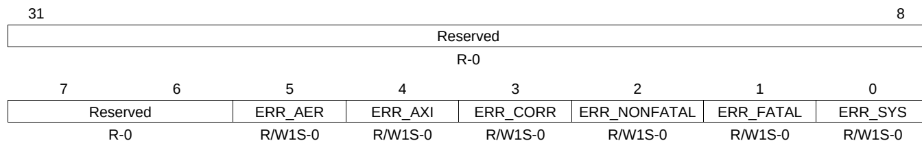
Figure 17-42. ERR_IRQ_STATUS_RAW Register
