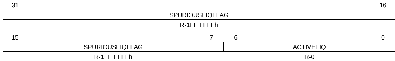
Figure 12-10. INTCPS_SIR_FIQ Register
