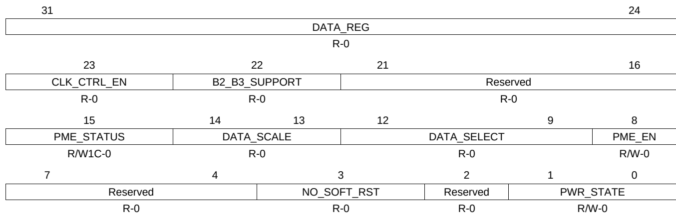
Figure 17-135. PM_CTL_STAT Register
