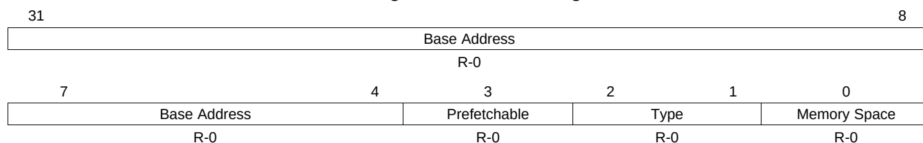
Figure 17-91. BAR0 Register
