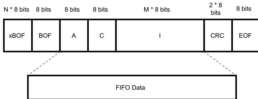
Figure 23-4. IrDA SIR Frame Format
