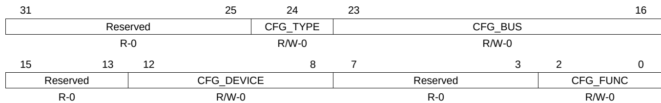
Figure 17-15. CFG_SETUP Register
