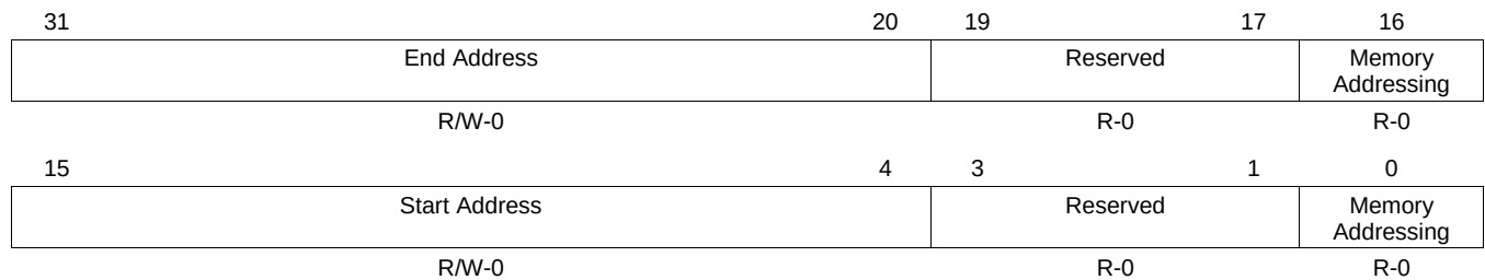
Figure 17-97. PREFETCH_MEM Register
