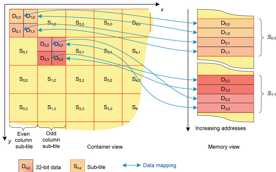
Figure 4-21. 32-bit Sub-tile
