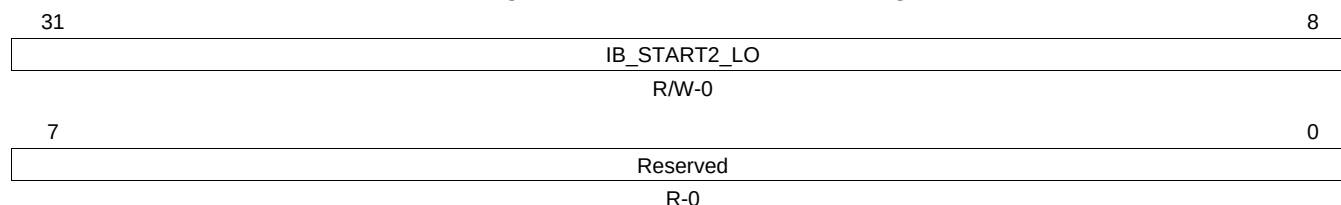
Figure 17-61. IB_START2_LO Register
