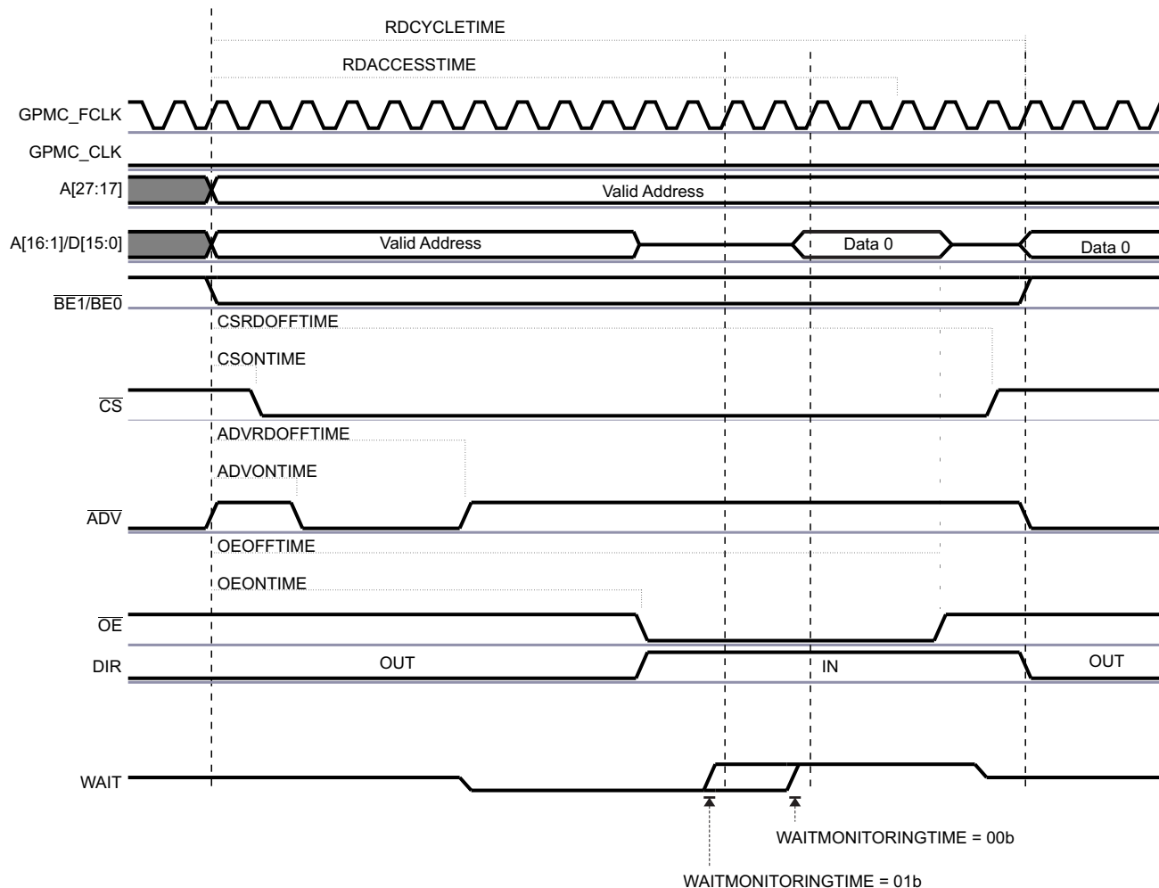
Figure 9-7. Wait Behavior During an Asynchronous Single Read Access (GPMCCLKDivider = 1)
