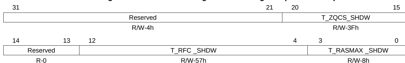
Figure 7-14. SDRAM Timing 3 Shadow Register (SDRTIM3SR)
