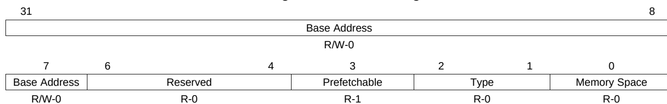
Figure 17-84. BAR5 Register
