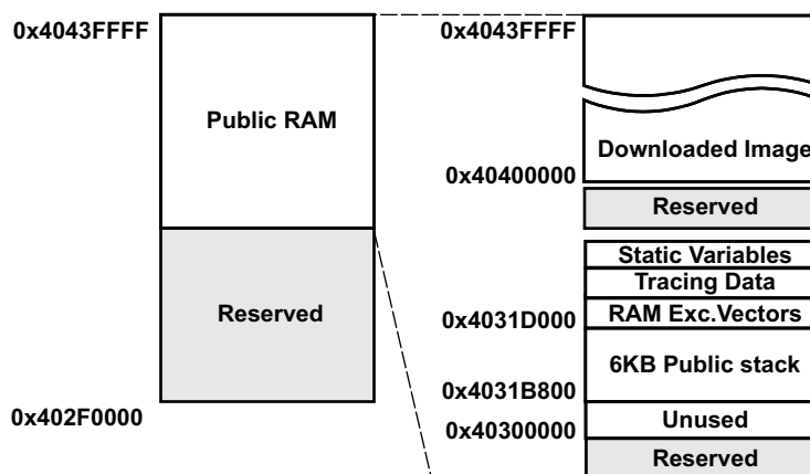
Figure 25-4. RAM Memory Map
