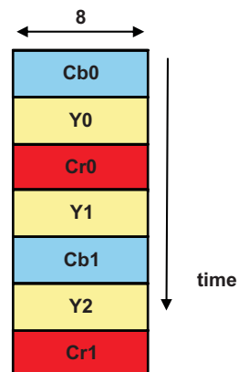
Figure 2-7. 8b Interface Discrete Sync Pixel Multiplexing
