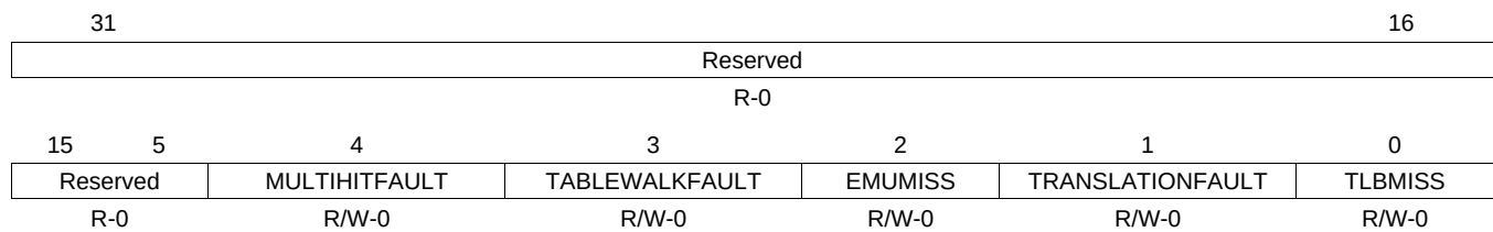
Figure 1-30. MMU_IRQENABLE
