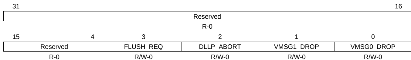
Figure 17-144. FLT_MASK2 Register
