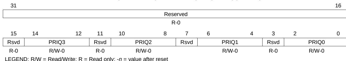
Figure 5-45. Queue Priority Register (QUEPRI)
