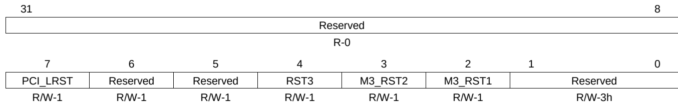
Figure 18-88. RM_DEFAULT_RSTCTRL Register
