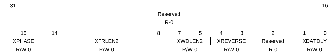
Figure 15-52. McBSP_XCR2_REG
