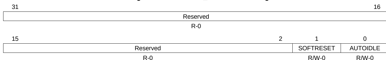
Figure 12-7. INTCPS_SYSCONFIG Register
