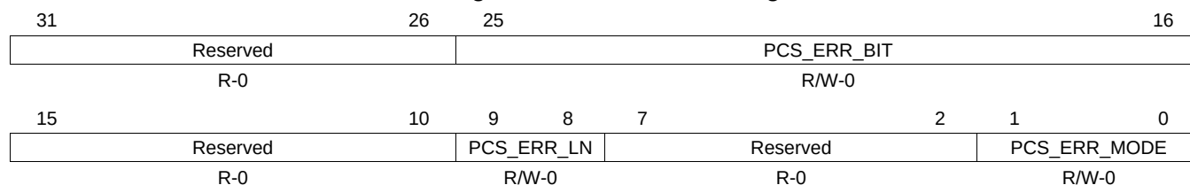
Figure 17-69. PCS_CFG1 Register
