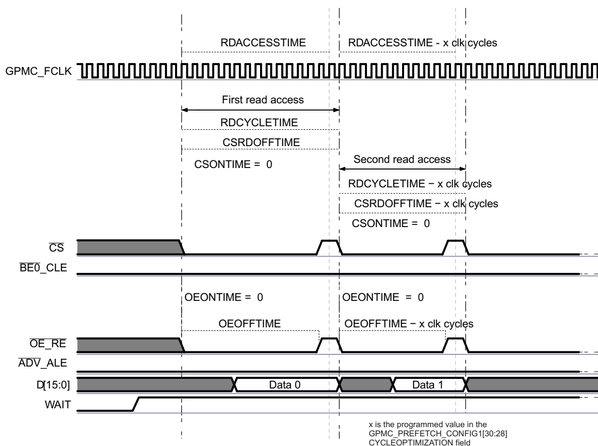
Figure 9-41. NAND Read Cycle Optimization Timing Description
