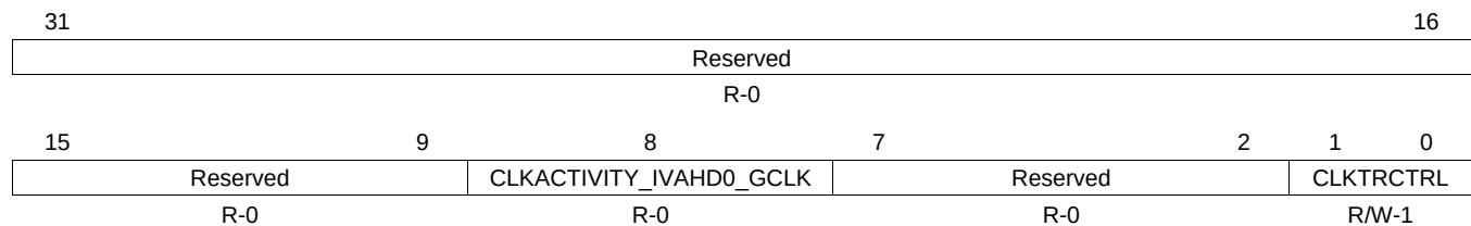
Figure 18-71. CM_IVAHD0_CLKSTCTRL Register
