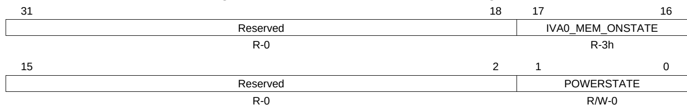
Figure 18-90. PM_IVAHD0_PWRSTCTRL Register
