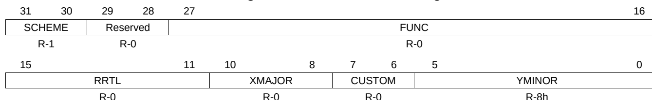
Figure 4-57. DMM_REVISION Register
