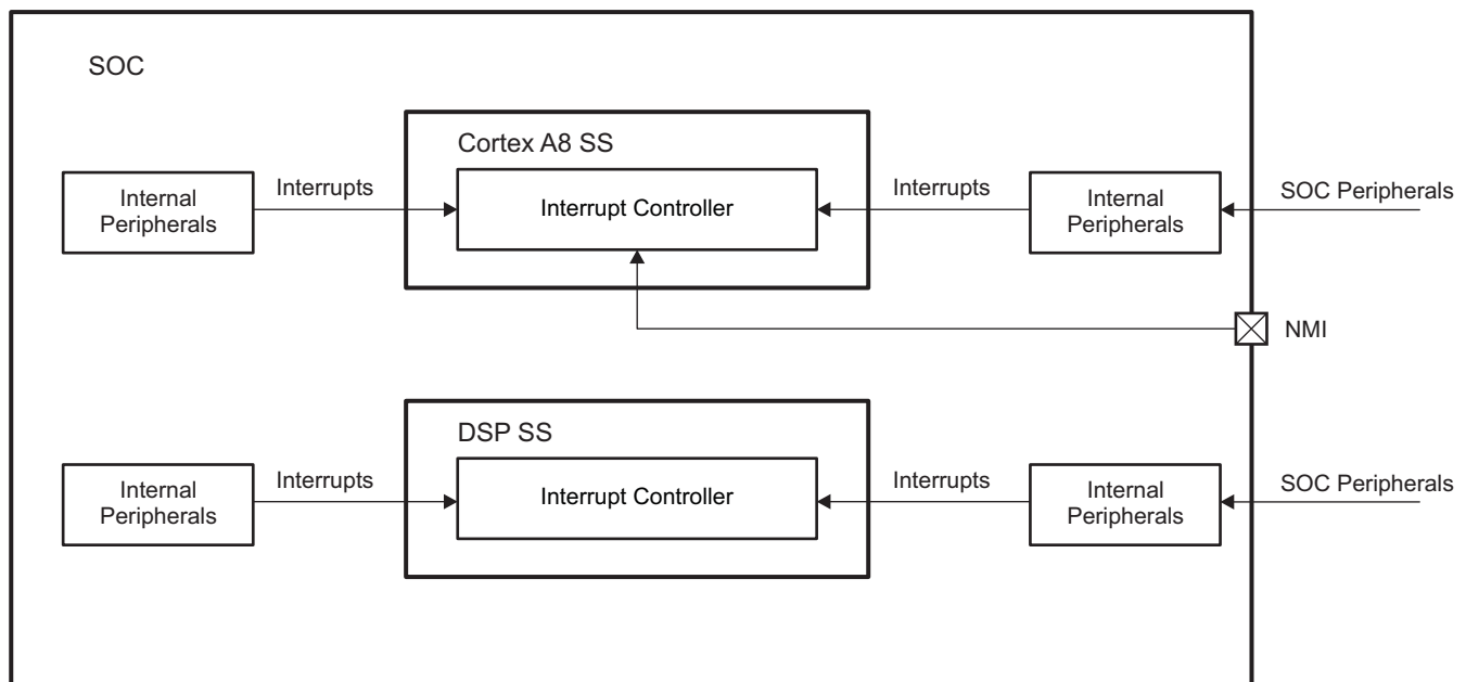
Figure 1-202. Interrupt Controller in Device
