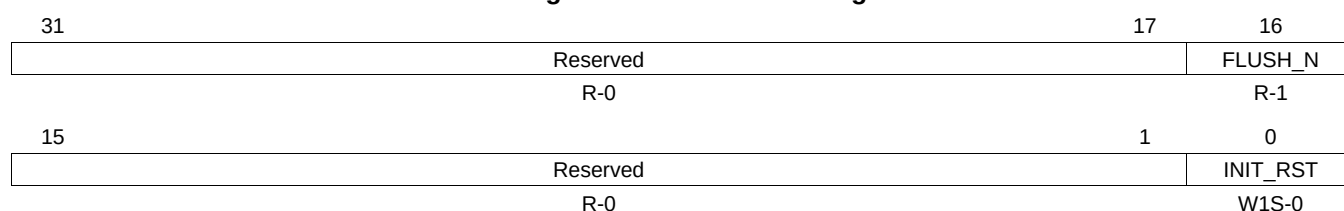
Figure 17-18. RSTCMD Register
