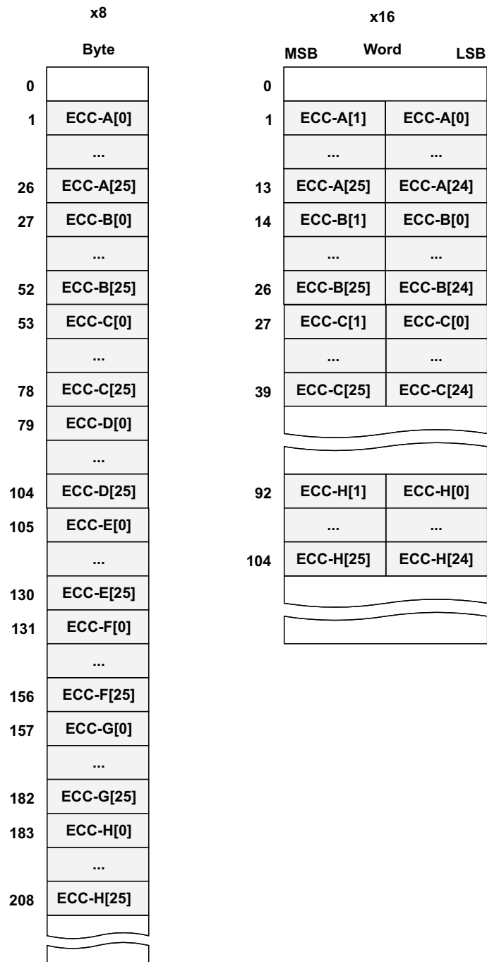
Figure 25-16. ECC Data Mapping for 4KB Page and 16b BCH Encoding
