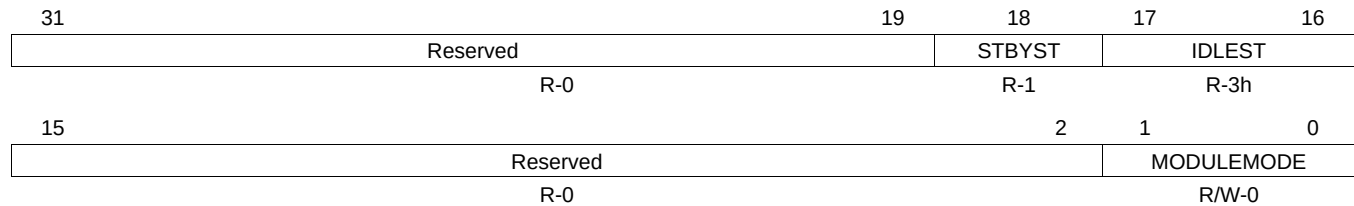
Figure 18-75. CM_IVAHD1_IVAHD_CLKCTRL Register
