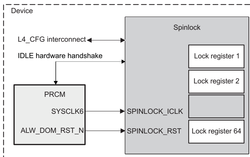
Figure 1-93. Spinlock Integration
