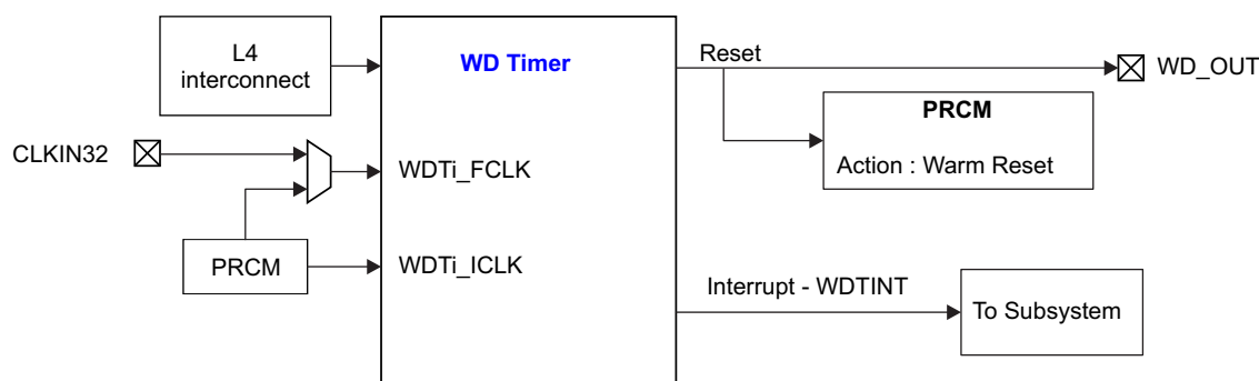
Figure 22-1. Watchdog Timer Block Diagram
