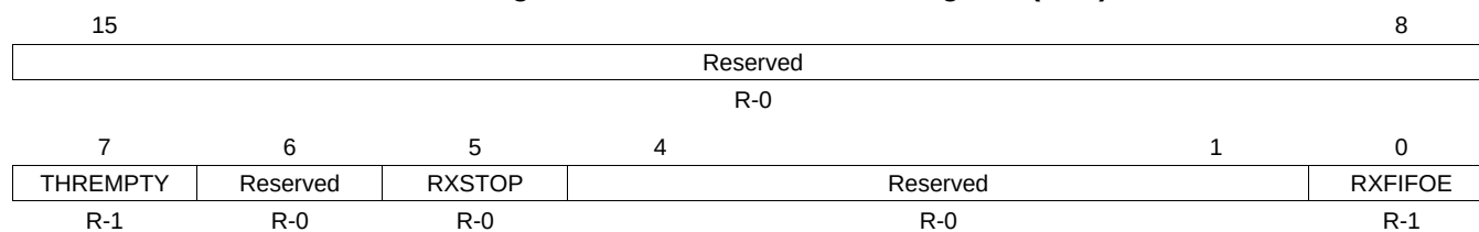
Figure 23-41. CIR Line Status Register (LSR)
