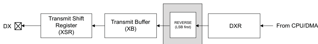
Figure 15-9. McBSP Transmission Physical Data Path
