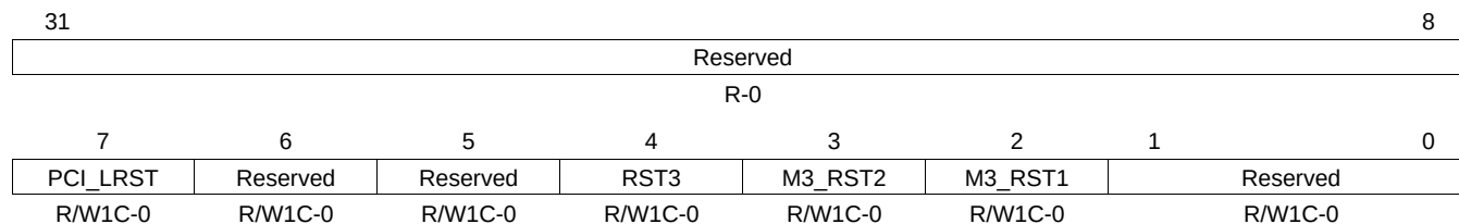
Figure 18-89. RM_DEFAULT_RSTST Register
