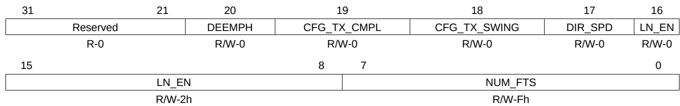
Figure 17-147. PL_GEN2 Register
