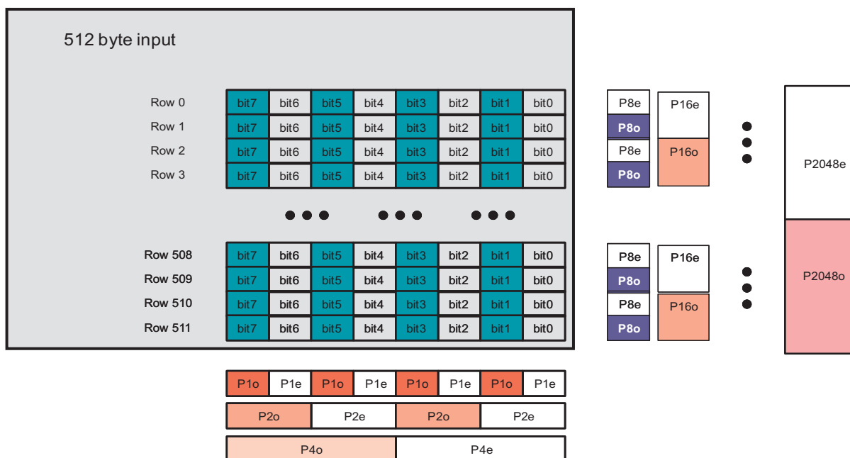
Figure 9-34. ECC Computation for a 512-Byte Data Stream (Read or Write)
