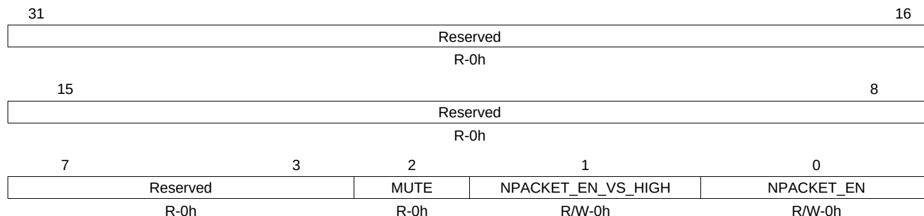
Figure 10-174. Audio Path Status Register (AUDIO_TXSTAT)
