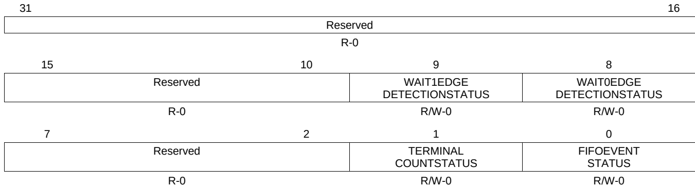
Figure 9-54. GPMC_IRQSTATUS
