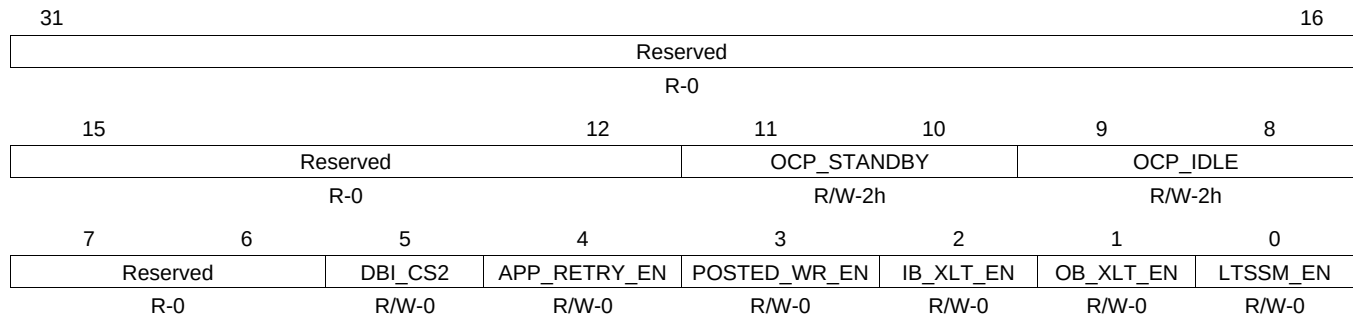
Figure 17-14. CMD_STATUS Register
