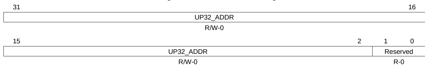
Figure 17-132. MSI_UP32 Register
