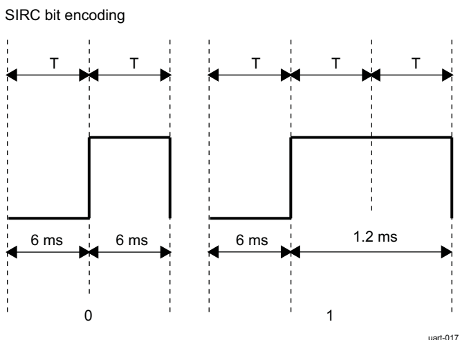
Figure 23-12. SIRC Bit Encoding
