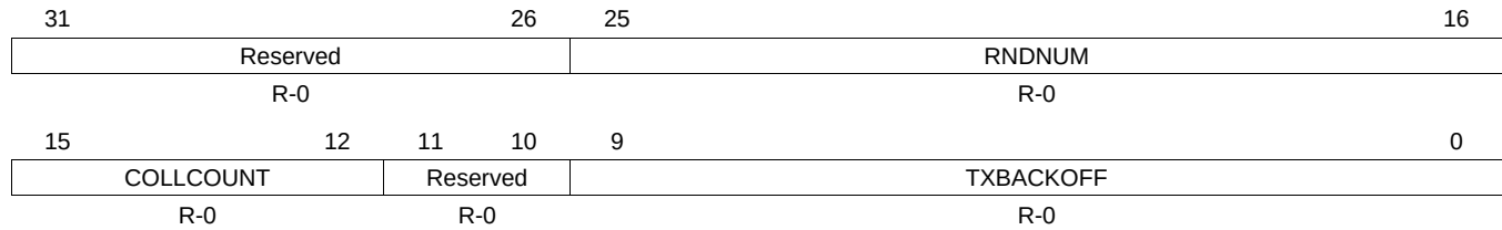
Figure 6-63. Back Off Random Number Generator Test Register (BOFFTEST)
