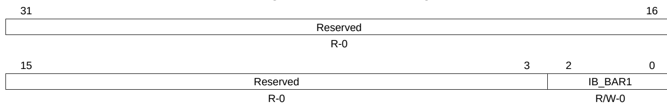
Figure 17-56. IB_BAR1 Register
