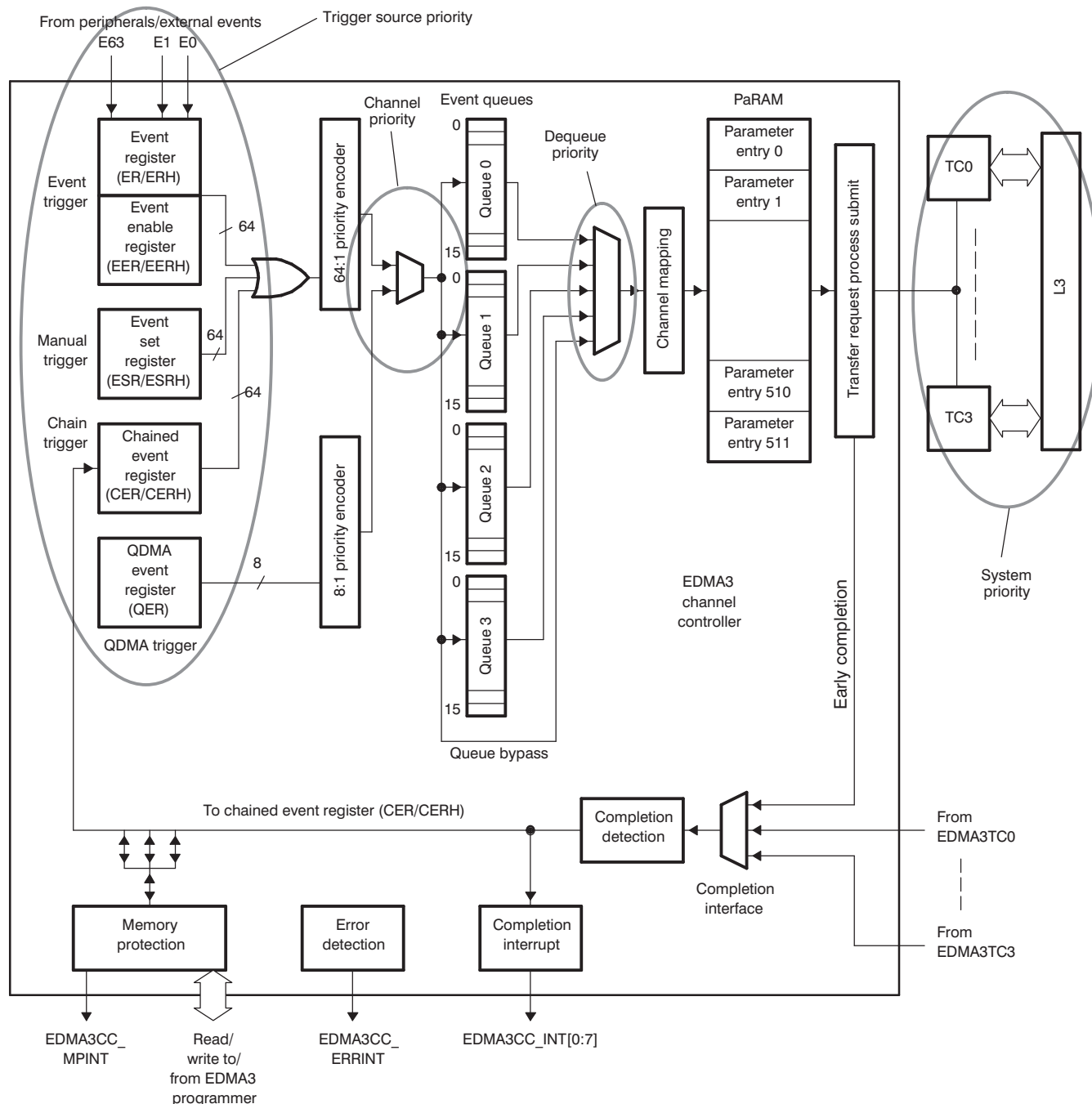
Figure 5-18. EDMA3 Prioritization
