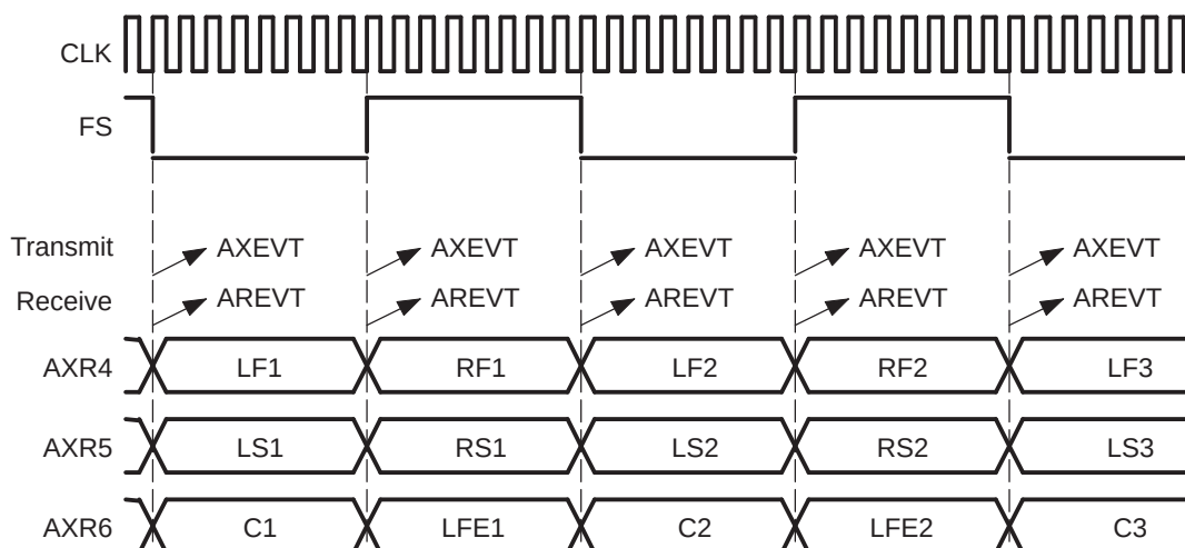
Figure 14-34. DMA Events in an Audio Example—Two Events (Scenario 1)
