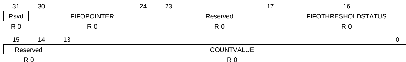
Figure 9-74. GPMC_PREFETCH_STATUS
