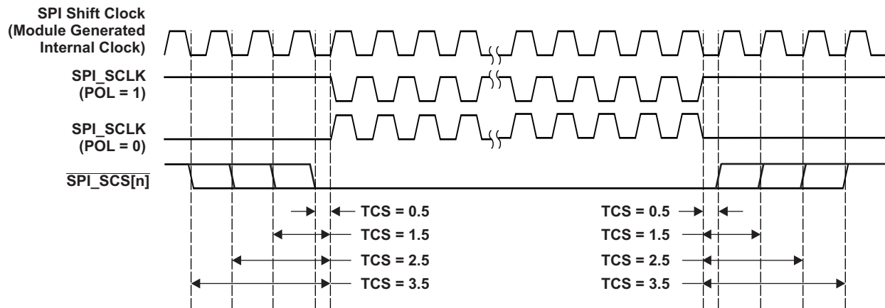
Figure 16-11. Chip-Select \overline{\text{SPI\_SCS}}[n] Timing Controls
