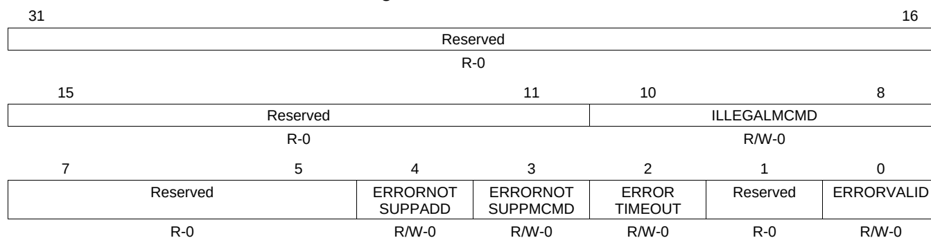
Figure 9-58. GPMC_ERR_TYPE
