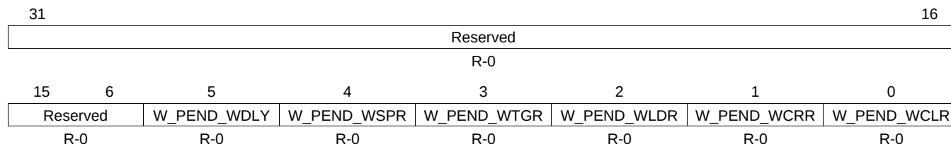
Figure 22-13. WDT_WWPS Register
