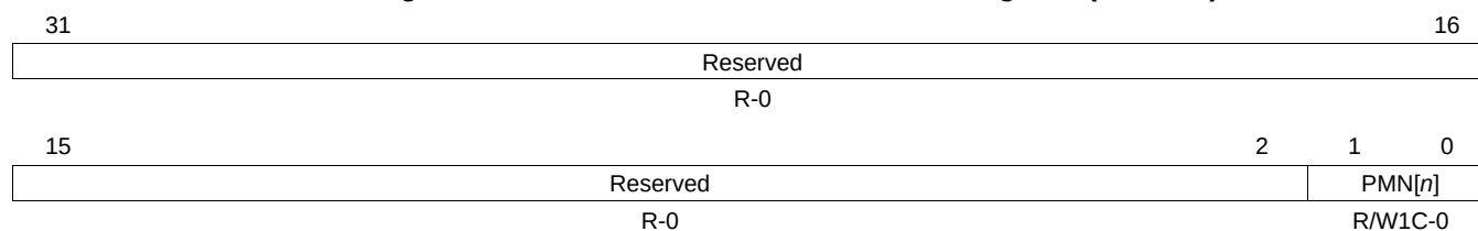
Figure 20-33. Port Serial ATA Notification Register (P#SNTF)
