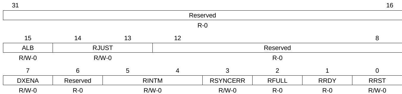
Figure 15-49. McBSP_SPCR1_REG
