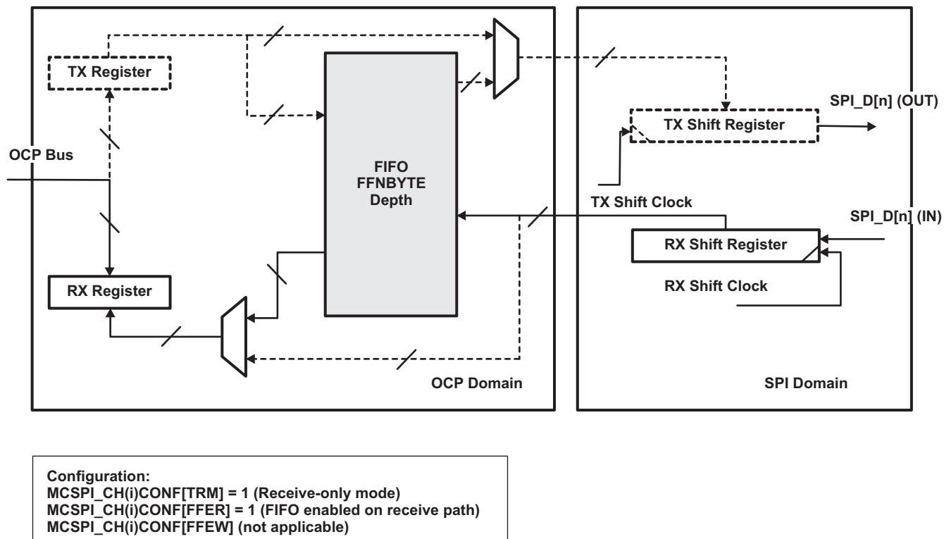
Figure 16-17. Receive-Only Mode With FIFO Used
