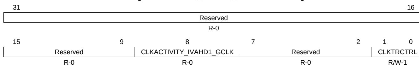
Figure 18-74. CM_IVAHD1_CLKSTCTRL Register
