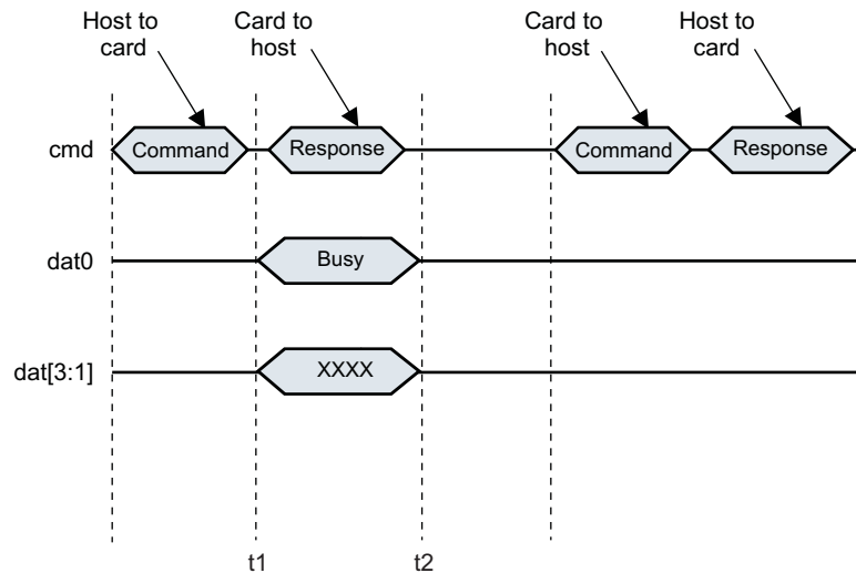
Figure 13-13. Busy Timeout for R1b, R5b Responses
