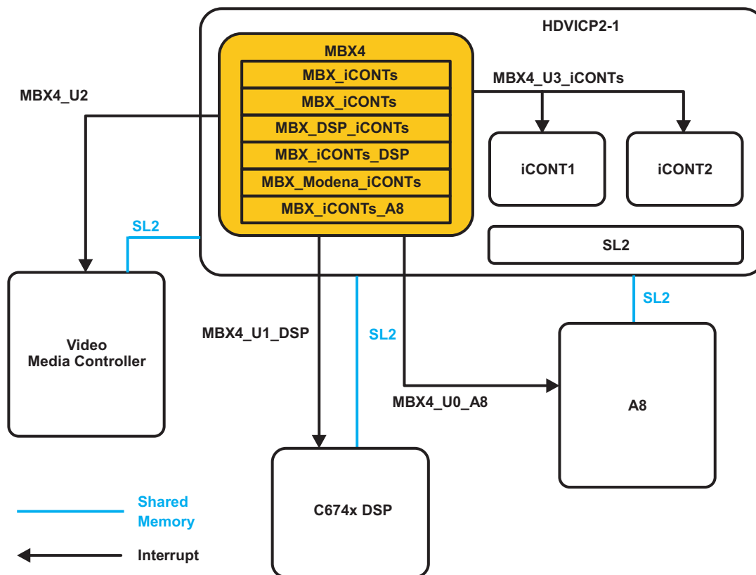
Figure 1-79. HDVICP2-1 IPC
