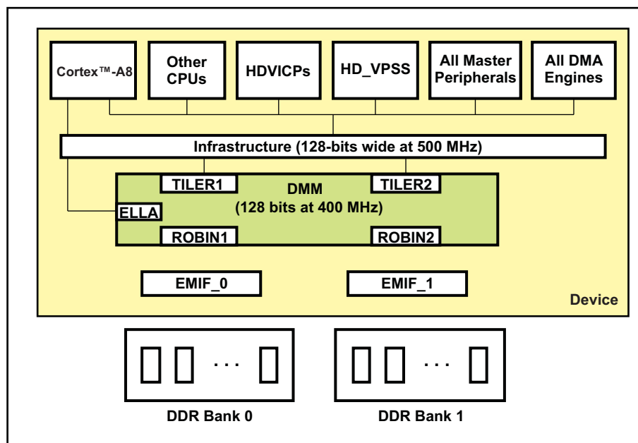
Figure 4-1. DMM Integration
