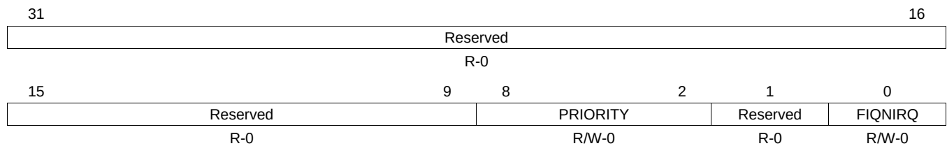
Figure 12-25. INTCPS_ILRm Register
