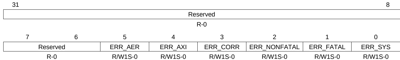
Figure 17-44. ERR_IRQ_ENABLE_SET Register
