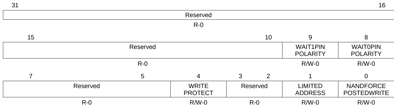
Figure 9-59. GPMC_CONFIG
