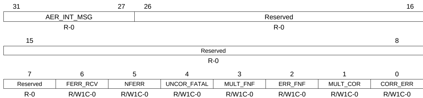
Figure 17-128. RC_ERR_ST Register
