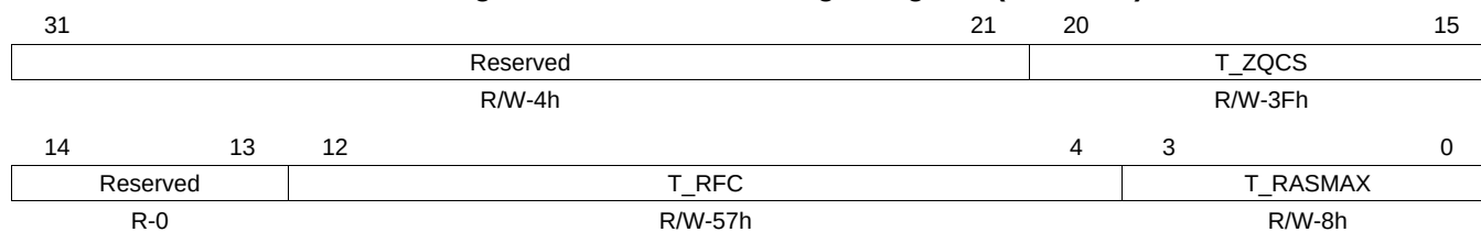
Figure 7-13. SDRAM Timing 3 Register (SDRTIM3)
