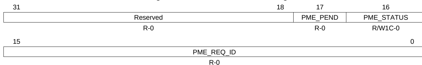
Figure 17-112. ROOT_STATUS Register
