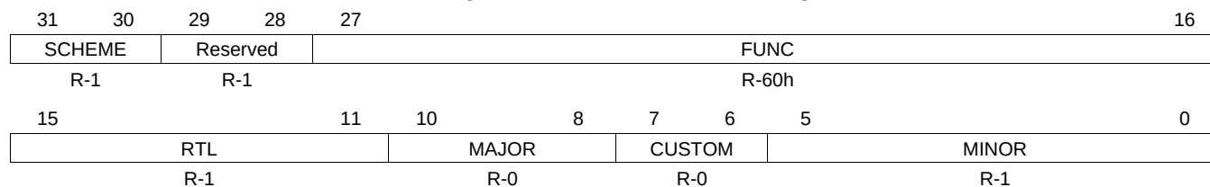
Figure 8-7. GPIO_REVISION Register
