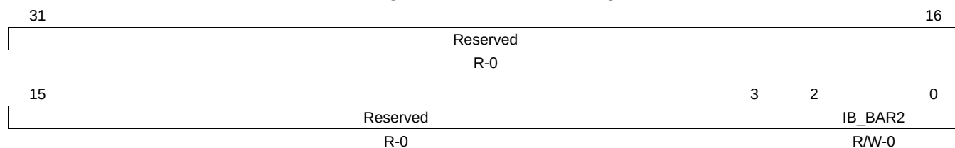
Figure 17-60. IB_BAR2 Register
