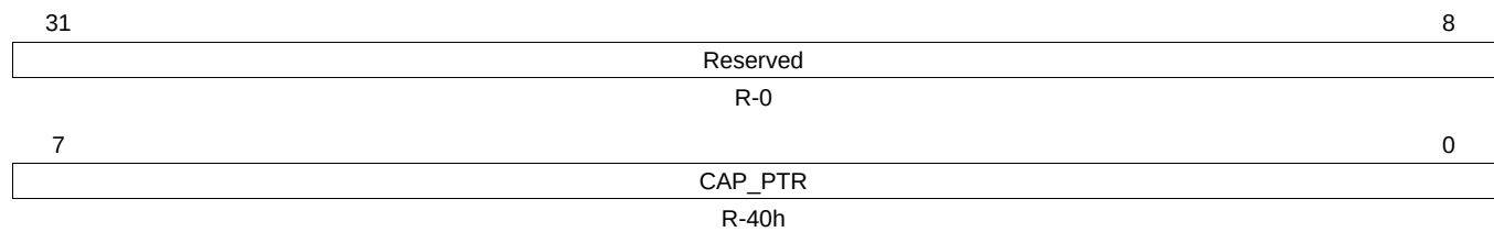
Figure 17-101. CAP_PTR Register
