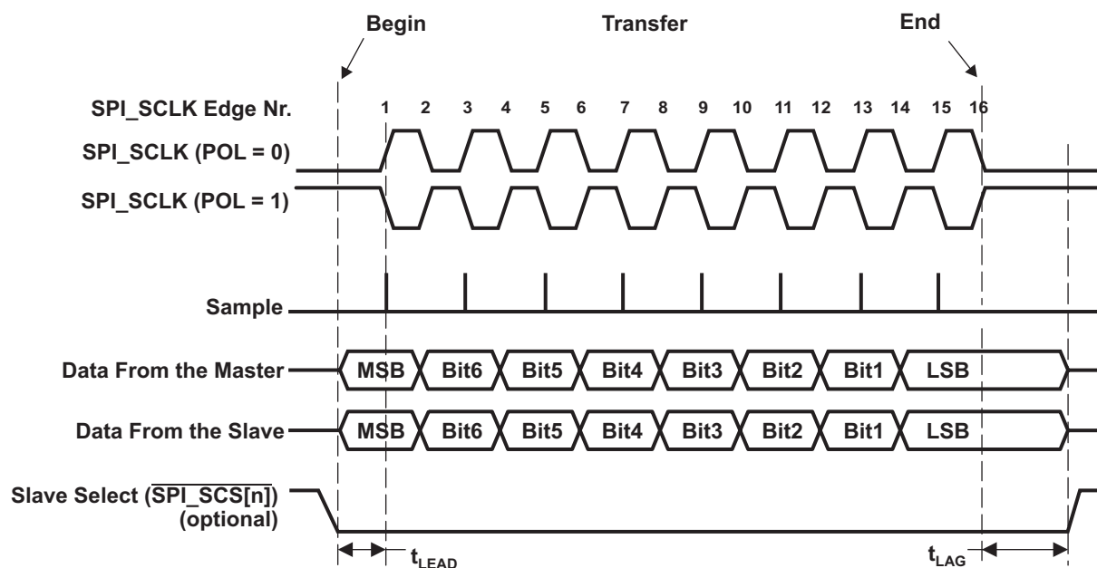
Figure 16-6. Full Duplex Single Transfer Format with PHA = 0
