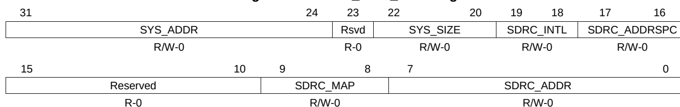
Figure 4-60. DMM_LISA_MAP Registers
