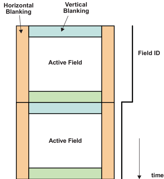
Figure 2-4. Digitized Video
