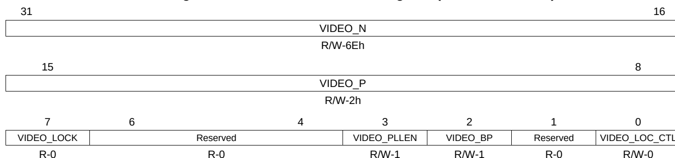
Figure 1-145. Video PLL Control Register (VIDEOPLL_CTRL)
