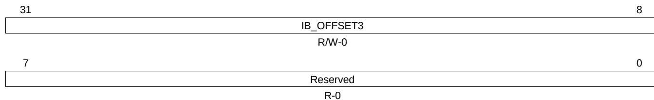
Figure 17-67. IB_OFFSET3 Register
