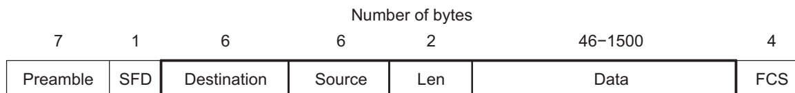
Figure 6-3. Ethernet Frame Format
