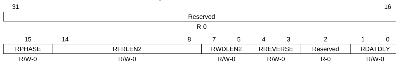
Figure 15-50. McBSP_RCR2_REG
