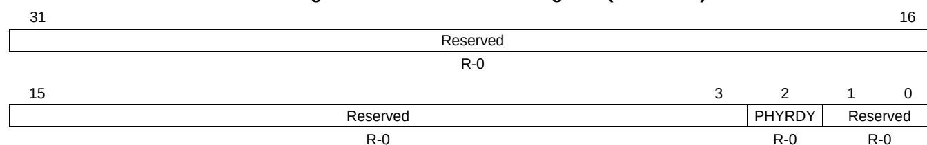
Figure 7-4. SDRAM Status Register (SDRSTAT)
