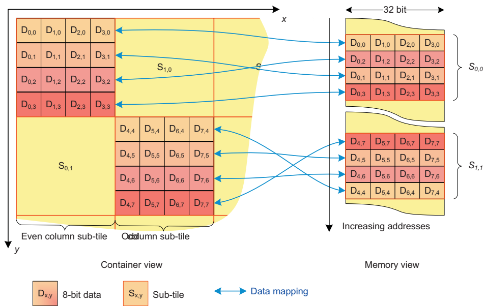
Figure 4-19. 8-bit Sub-tile
