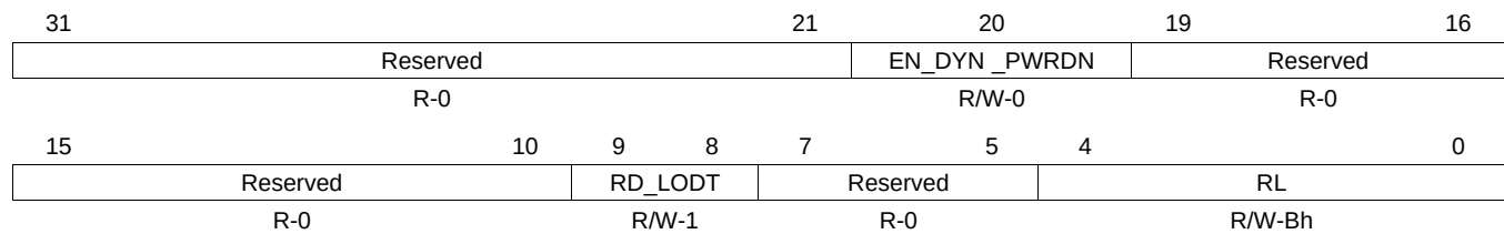
Figure 7-29. DDR PHY Control Register (DDRPHYCR)
