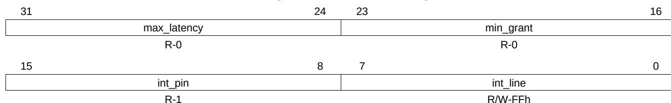
Figure 17-89. INT_PIN Register
