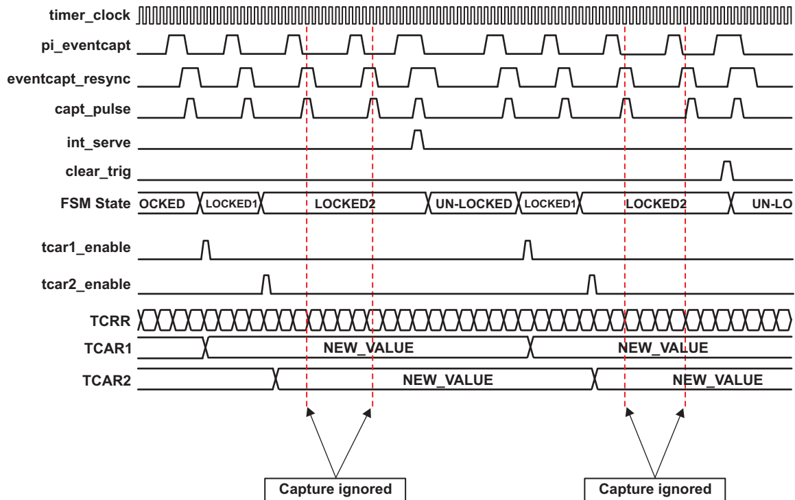
Figure 21-5. Capture Wave Example for CAPT_MODE = 1
