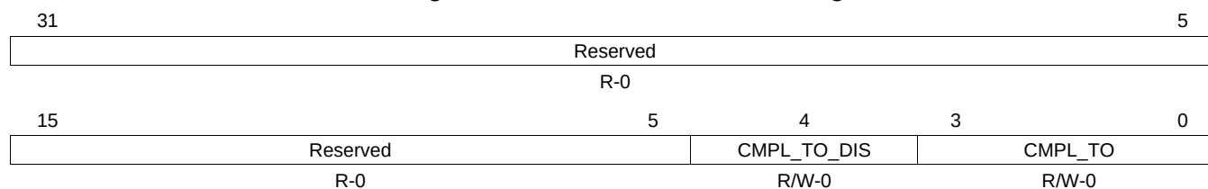
Figure 17-114. DEV_STAT_CTRL2 Register
