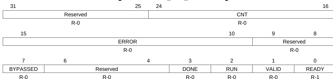
Figure 4-71. DMM_PAT_STATUS Registers
