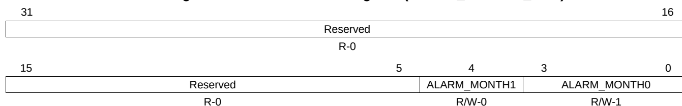
Figure 19-17. Alarm Month Register (ALARM_MONTHS_REG)
