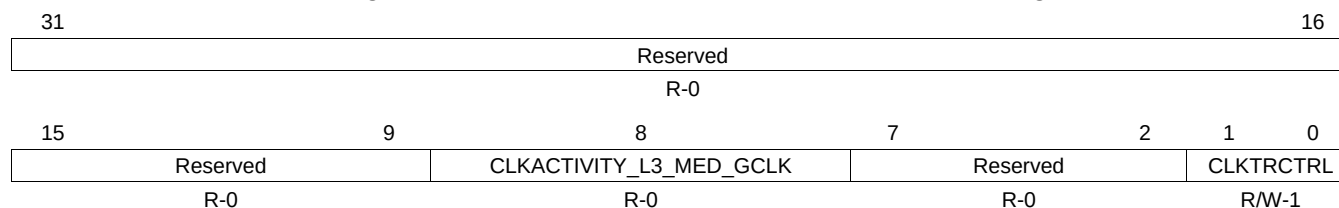
Figure 18-58. CM_DEFAULT_L3_MED_CLKSTCTRL Register
