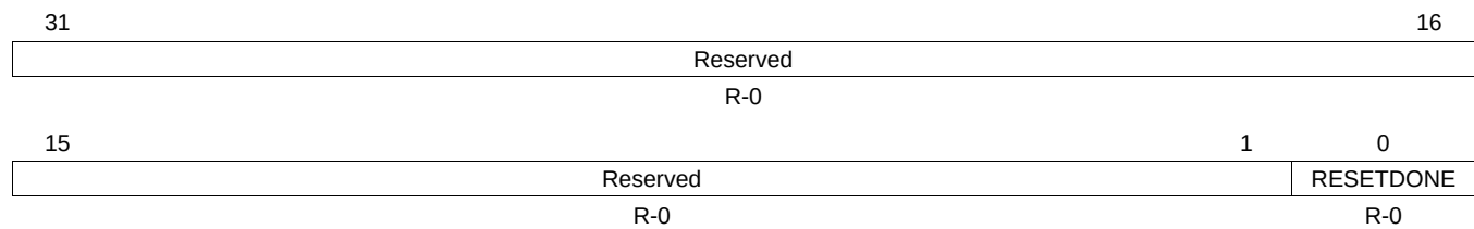
Figure 12-8. INTCPS_SYSSTATUS Register
