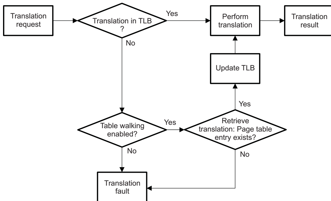
Figure 1-14. MMU Address Translation Process
