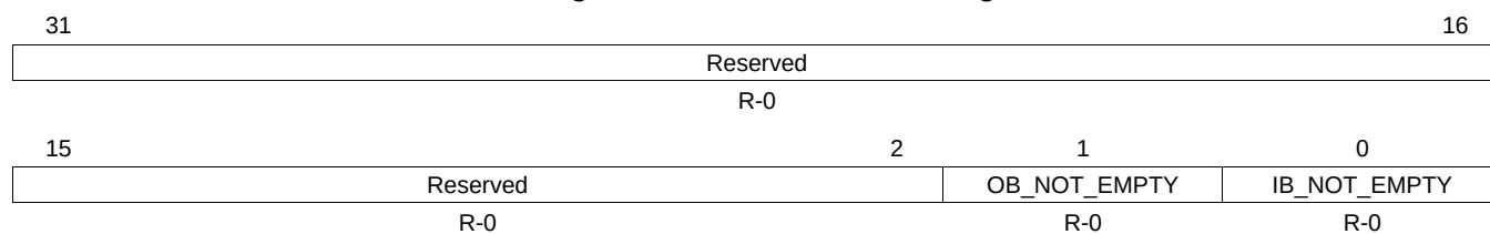
Figure 17-21. ACT_STATUS Register
