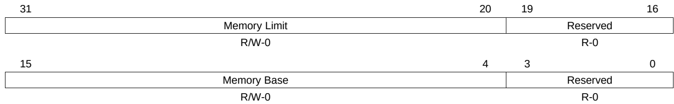
Figure 17-96. MEMSPACE Register
