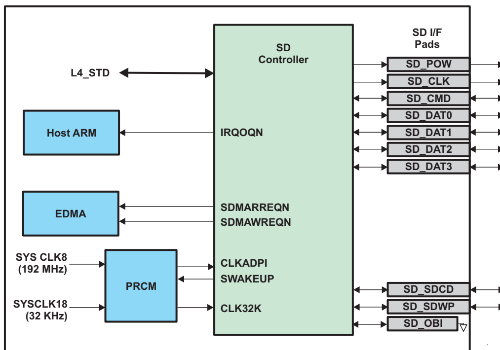
Figure 13-1. SD/SDIO1 Overview
