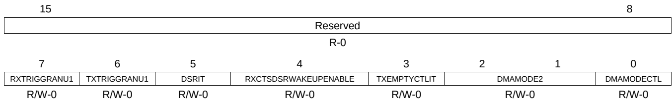
Figure 23-55. Supplementary Control Register (SCR)
