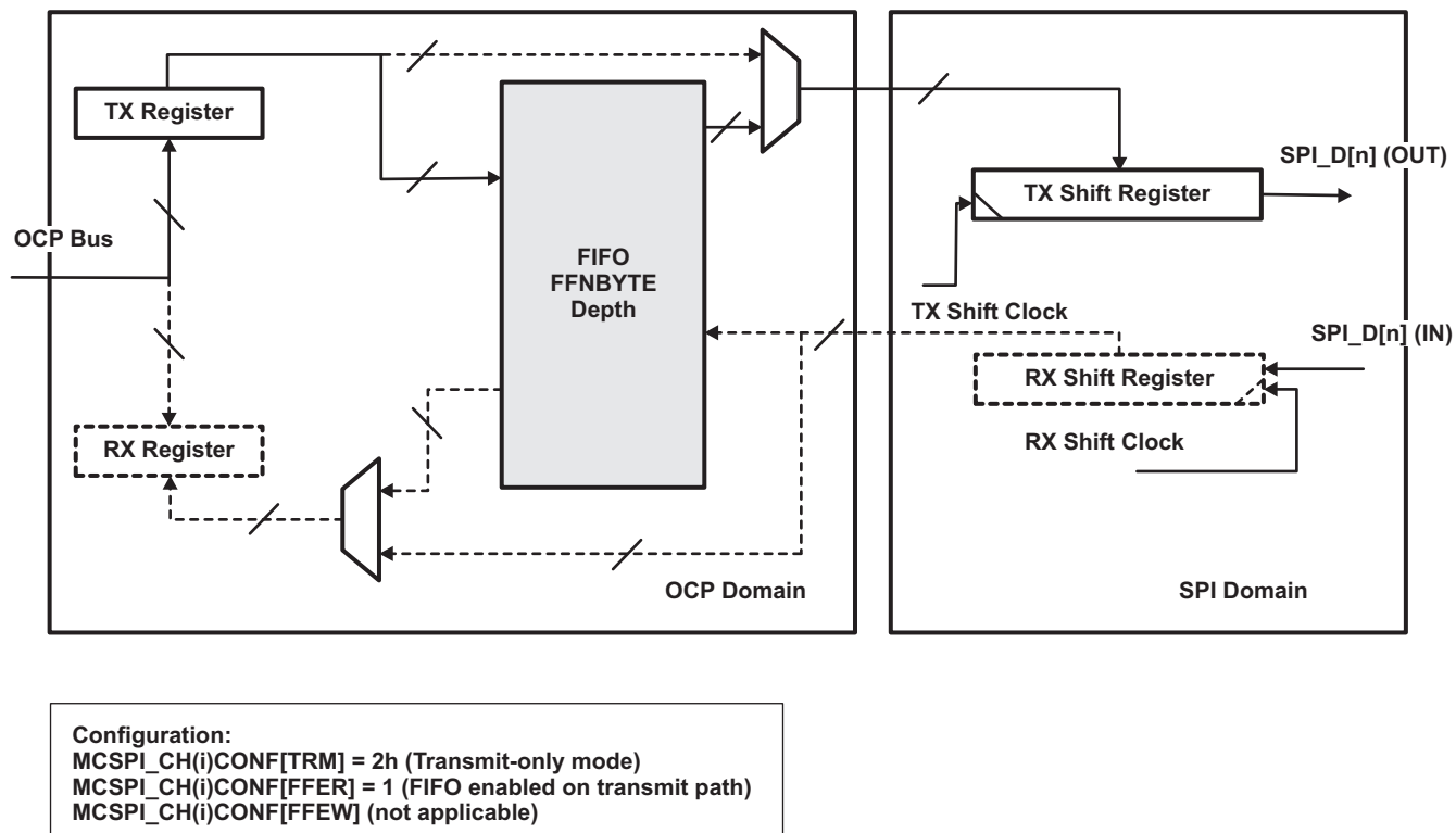
Figure 16-16. Transmit-Only Mode With FIFO Used
