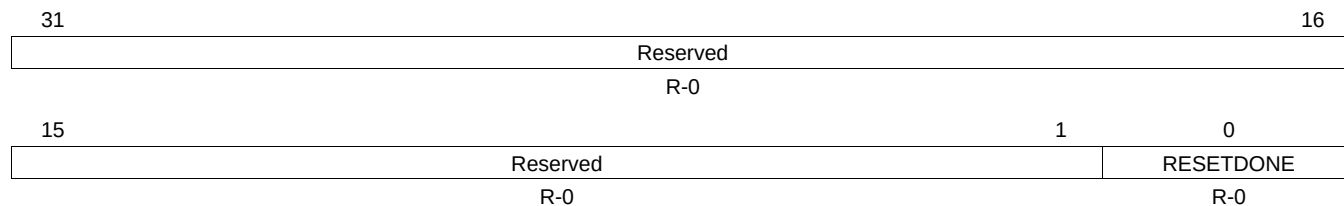
Figure 8-18. GPIO_SYSSTATUS Register
