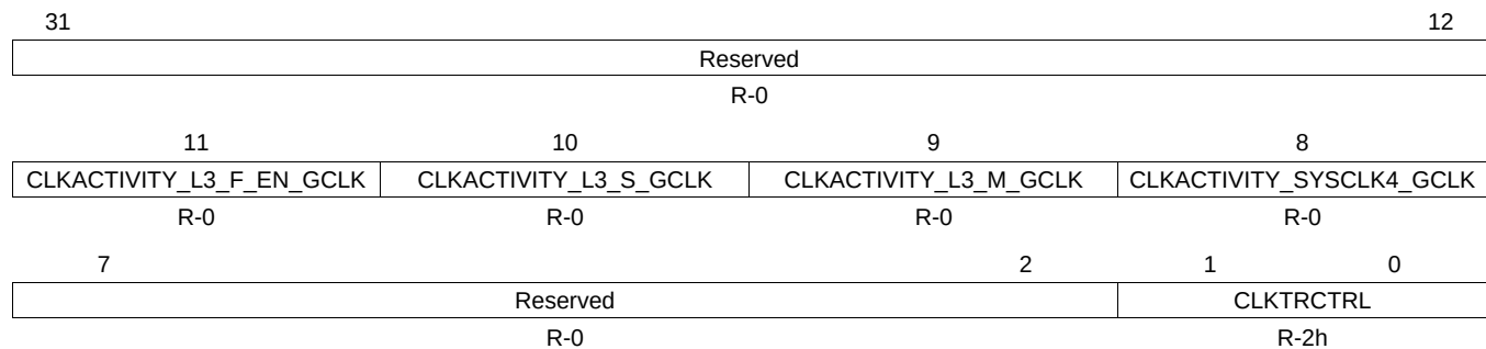
Figure 18-114. CM_ALWON_SYSCCLK4_CLKSTCTRL Register
