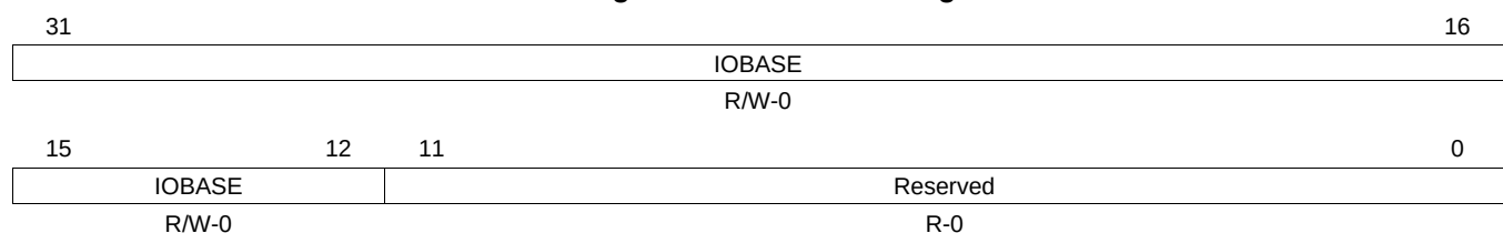
Figure 17-16. IOBASE Register
