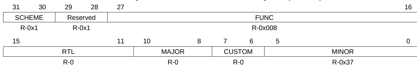
Figure 15-33. Revision Number Register (REVNB)
