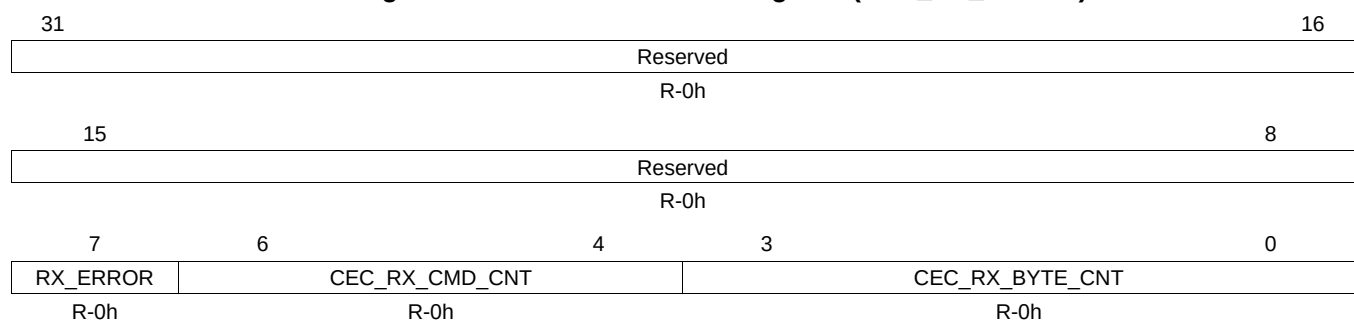
Figure 10-227. CEC Rx Count Register (CEC_RX_COUNT)
