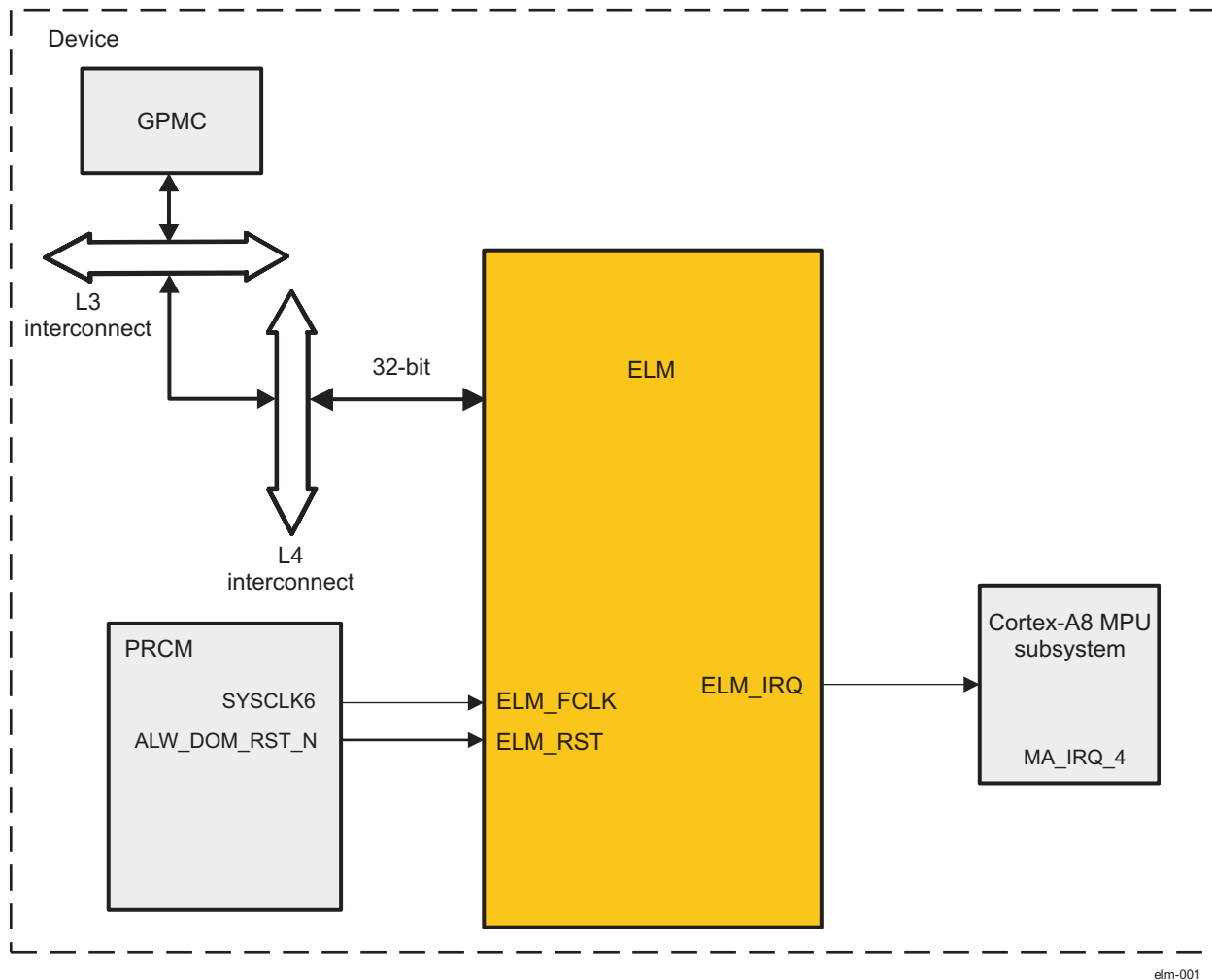
Figure 1-100. ELM Integration
