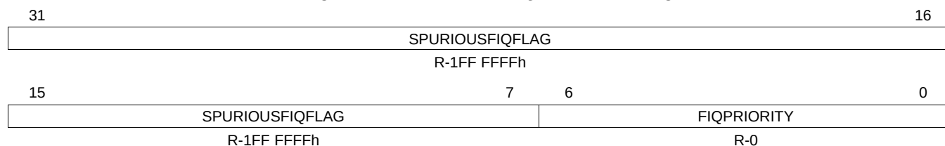
Figure 12-15. INTCPS_FIQ_PRIORITY Register
