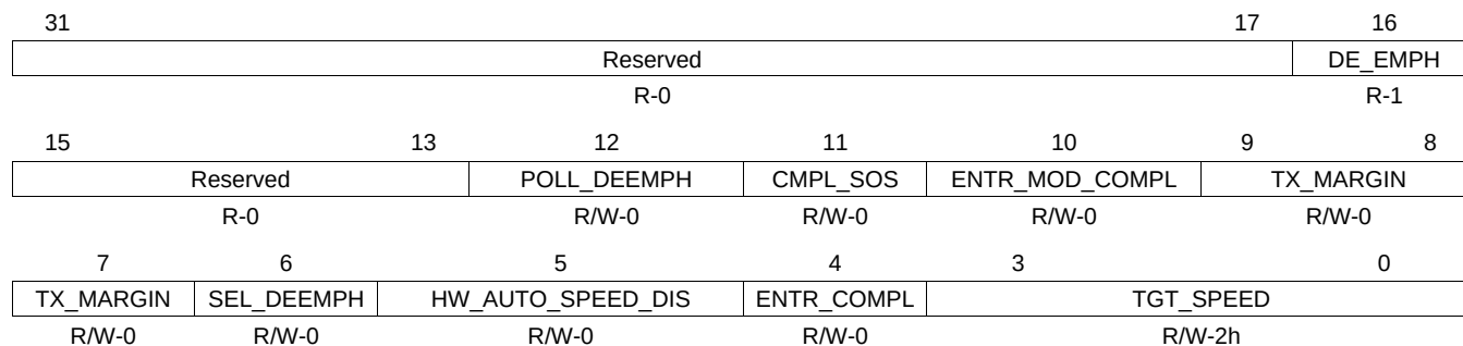
Figure 17-115. LINK_CTRL2 Register
