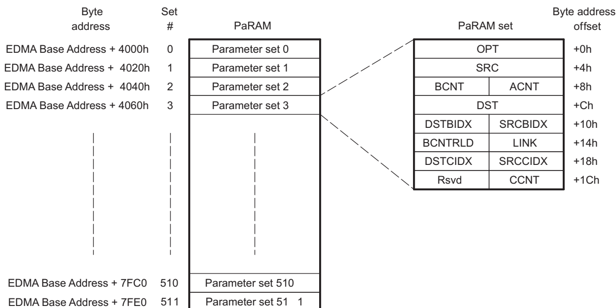
Figure 5-7. PaRAM Set
