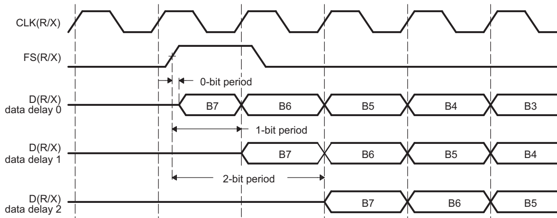
Figure 15-30. Range of Programmable Data Delay
