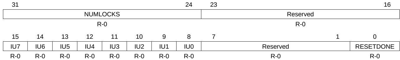
Figure 1-98. System Status Register (SPINLOCK_SYSSTAT)
