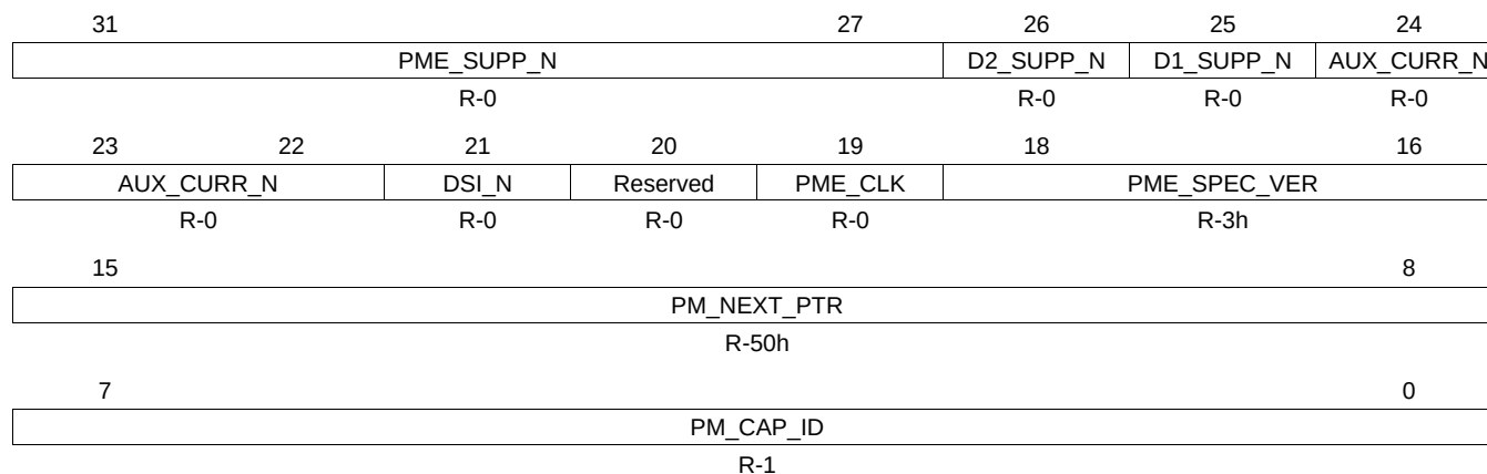
Figure 17-134. PMCAP Register
