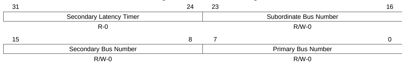
Figure 17-94. BUSNUM Register
