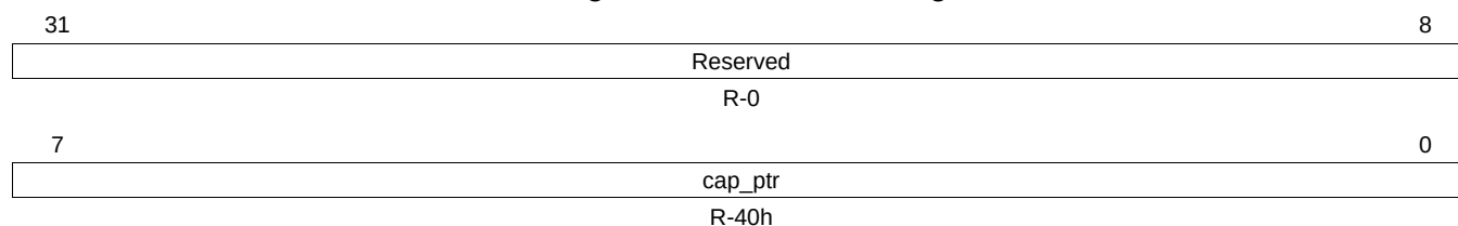
Figure 17-88. CAP_PTR Register
