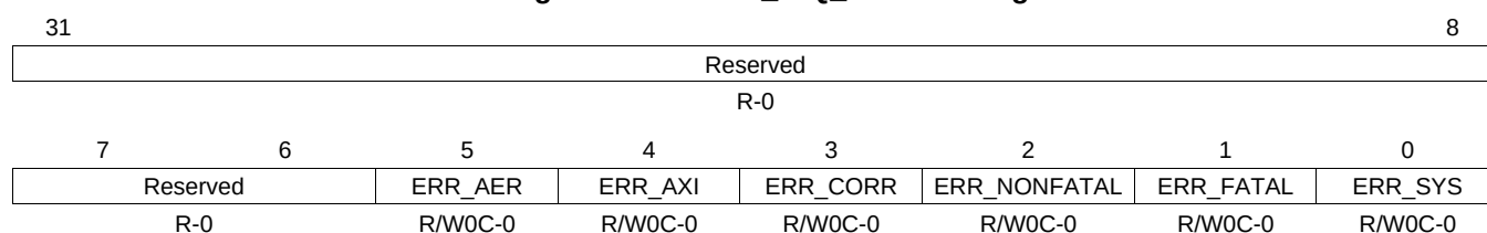
Figure 17-43. ERR_IRQ_STATUS Register
