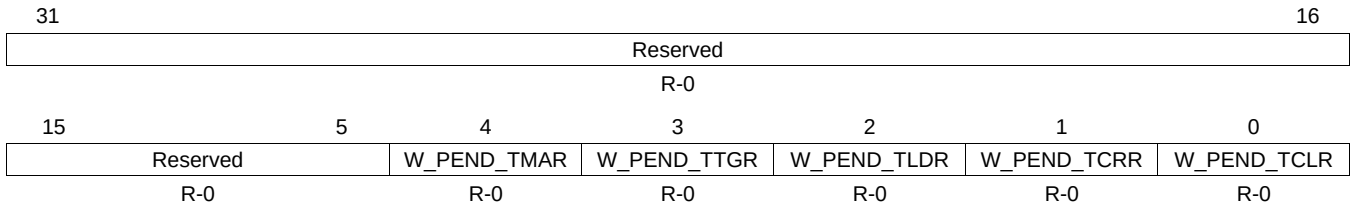
Figure 21-20. TWPS Register
