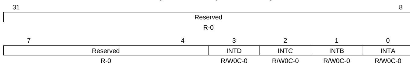
Figure 17-39. IRQ_STATUS Register
