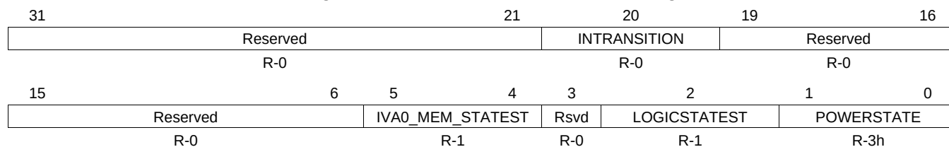
Figure 18-91. PM_IVAHD0_PWRSTST Register
