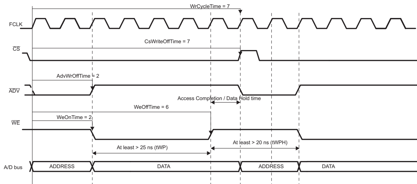
Figure 9-50. Asynchronous Single Write Access (Timing Parameters in Clock Cycles)
