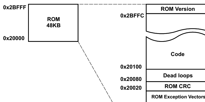
Figure 25-3. ROM Memory Map
