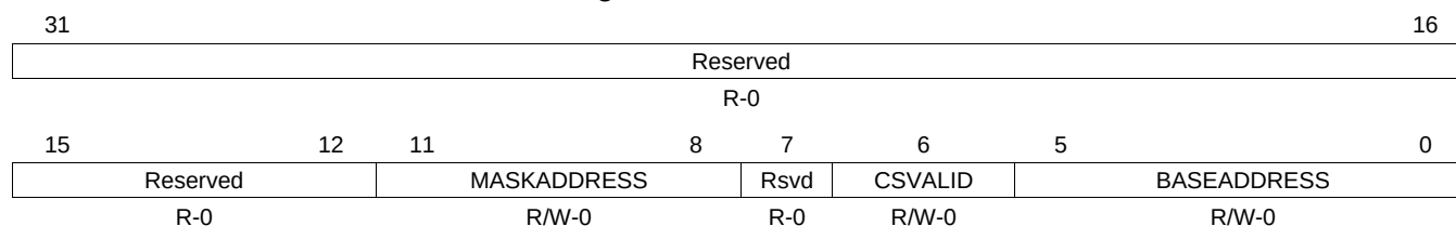
Figure 9-67. GPMC_CONFIG7_i
