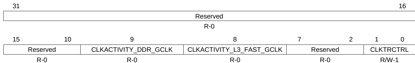
Figure 18-59. CM_DEFAULT_L3_FAST_CLKSTCTRL Register
