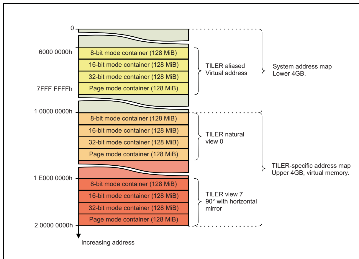
Figure 4-10. Memory Map
