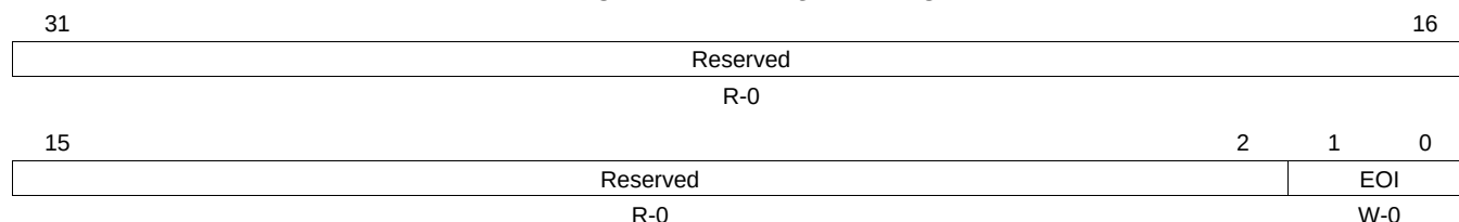
Figure 17-25. IRQ_EOI Register
