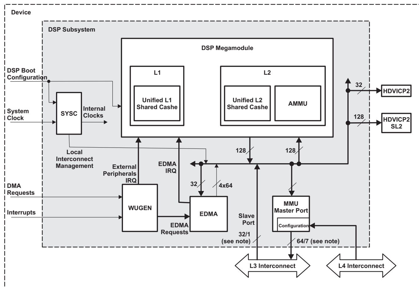
Figure 1-8. DSP Subsystem Block Diagram
