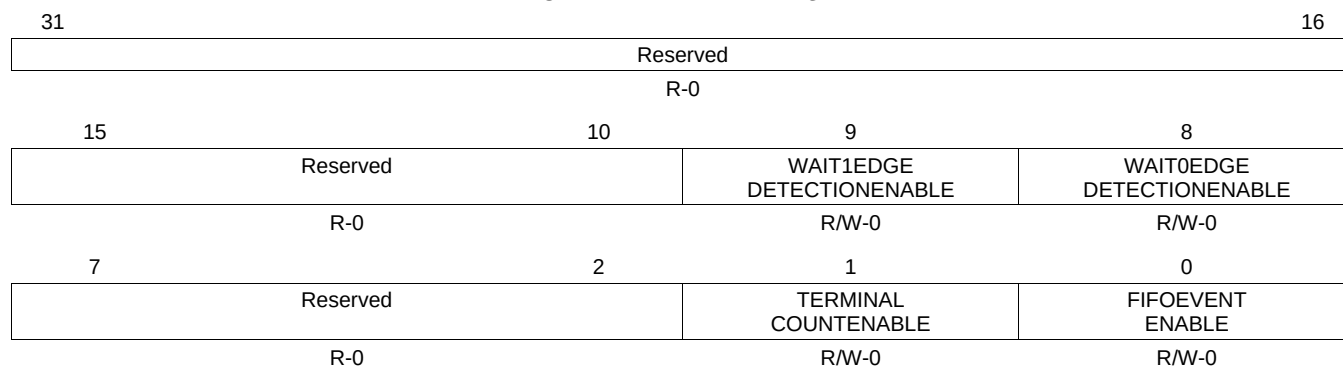
Figure 9-55. GPMC_IRQENABLE
