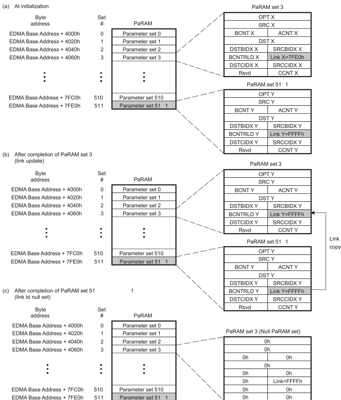
Figure 5-9. Linked Transfer
