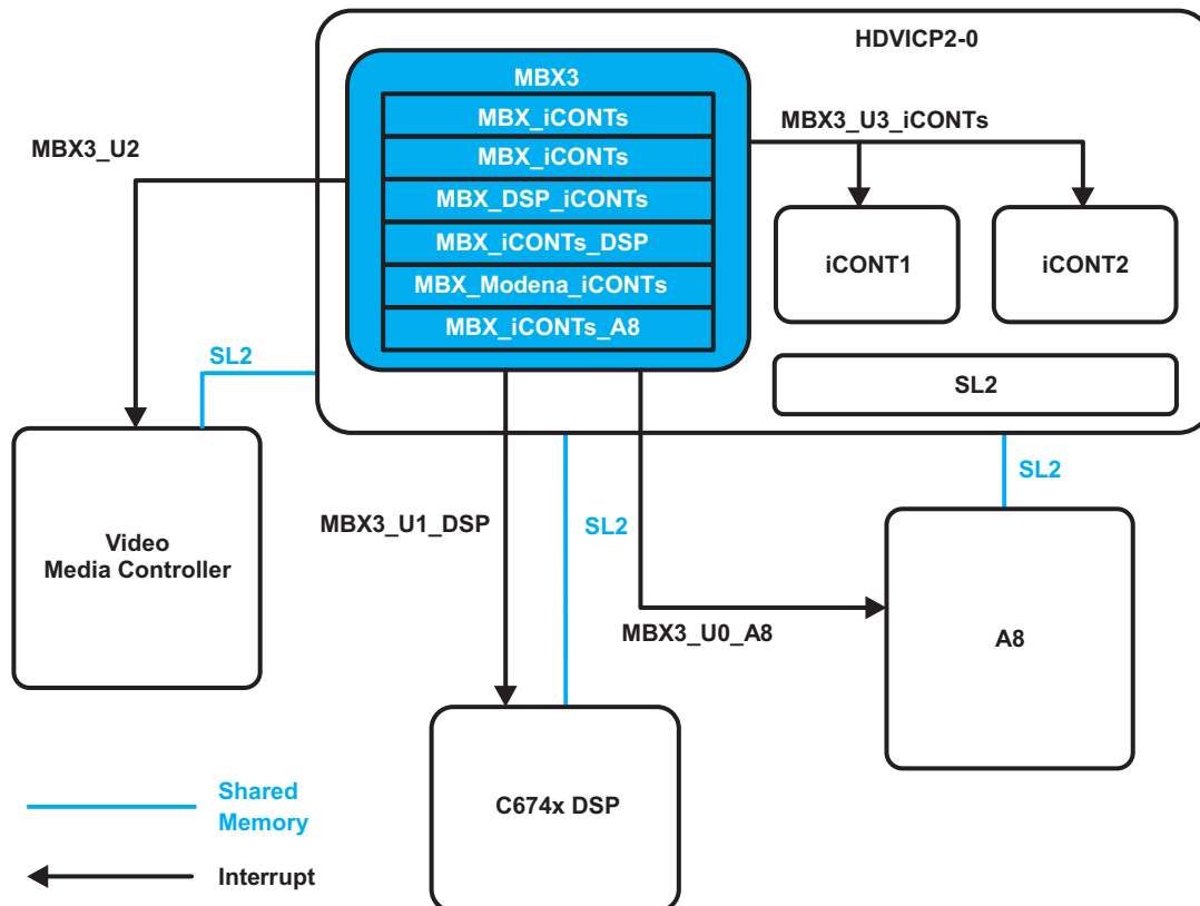
Figure 1-78. HDVICP2-0 IPC
