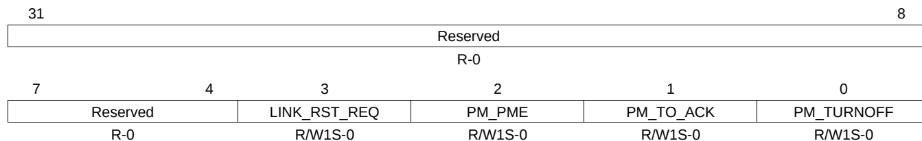
Figure 17-48. PMRST_ENABLE_SET Register
