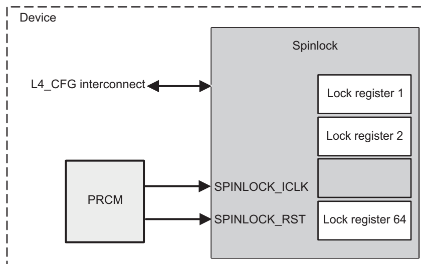
Figure 1-92. Spinlock Module
