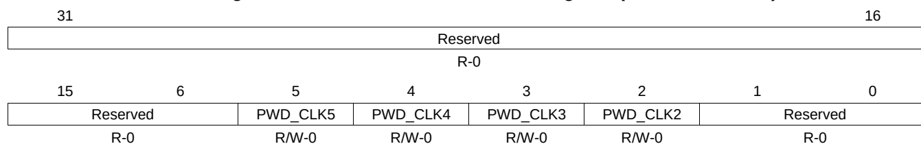
Figure 1-154. Audio PLL Powerdown Register (AUDIOPLL_PWD)
