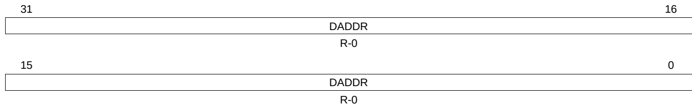
Figure 5-122. Destination FIFO Destination Address Register (DFDST n )
