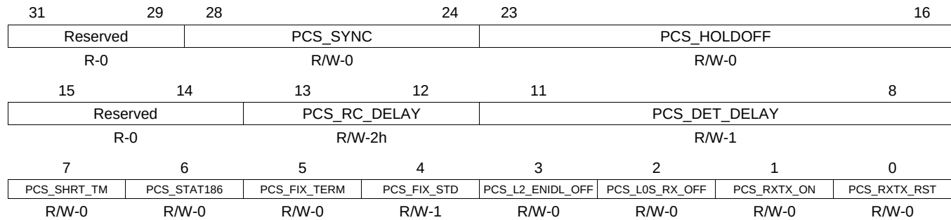
Figure 17-68. PCS_CFG0 Register
