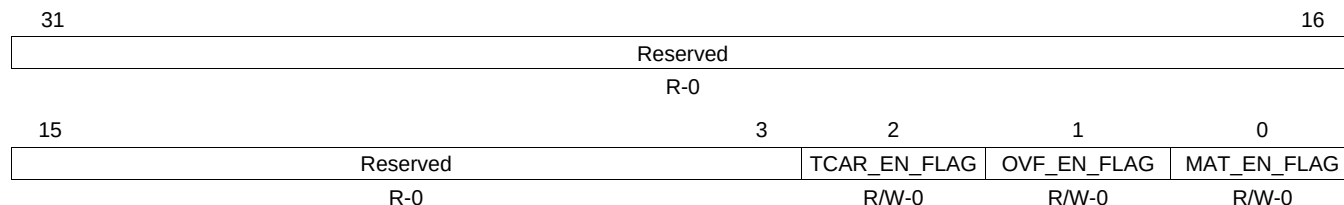
Figure 21-14. IRQENABLE_CLR Register
