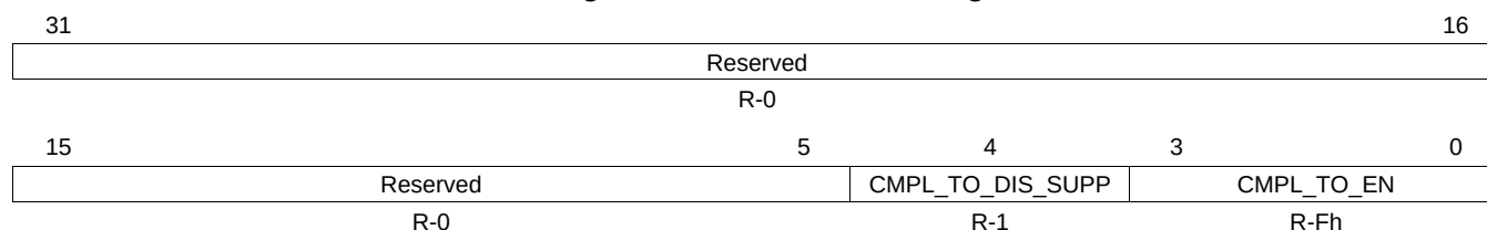
Figure 17-113. DEV_CAP2 Register
