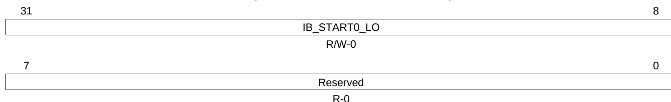
Figure 17-53. IB_START0_LO Register
