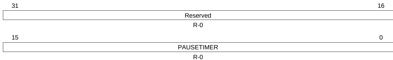
Figure 6-66. Transmit Pause Timer Register (TXPAUSE)
