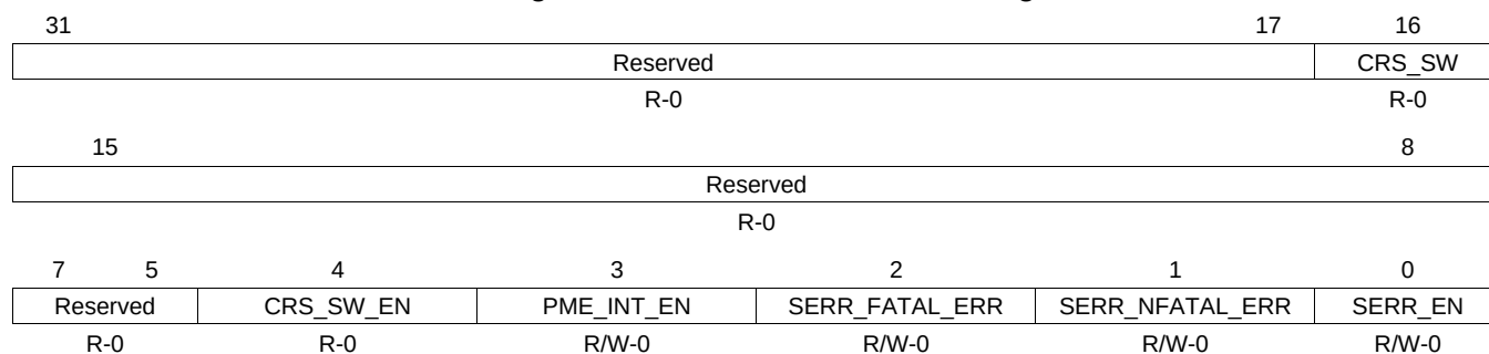
Figure 17-111. ROOT_CTRL_CAP Register
