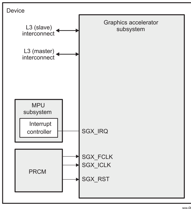
Figure 1-45. Graphics Accelerator Highlight
