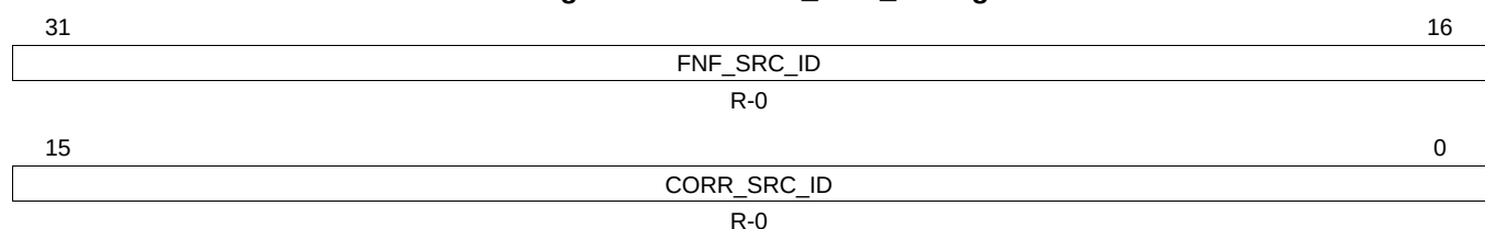
Figure 17-129. ERR_SRC_ID Register
