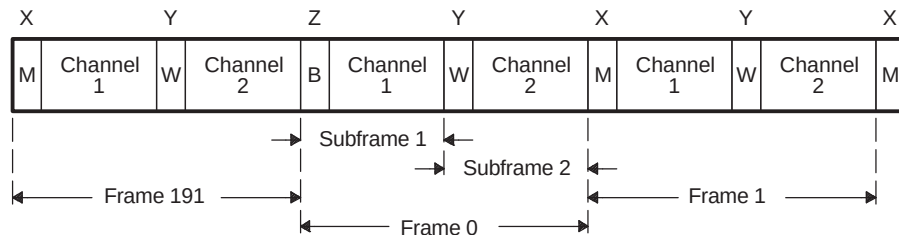
Figure 14-12. S/PDIF Frame Format
