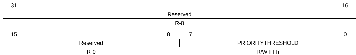
Figure 12-16. INTCPS_THRESHOLD Register
