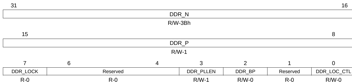
Figure 1-134. DDR PLL Control Register (DDRPLL_CTRL)
