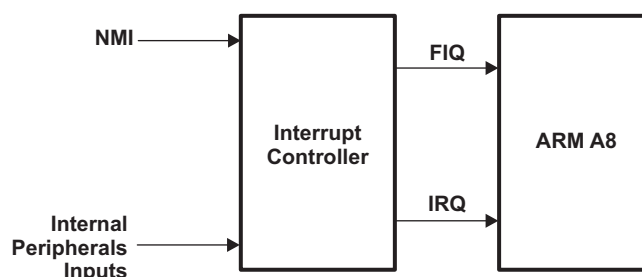
Figure 12-1. Interrupt Controller
