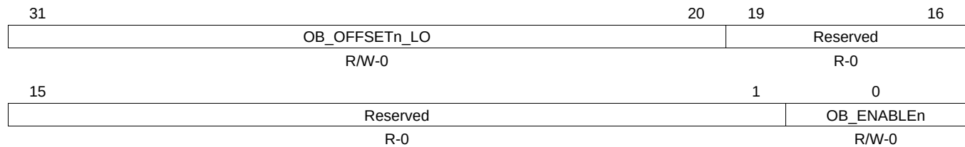
Figure 17-50. OB_OFFSET_INDEXn Register
