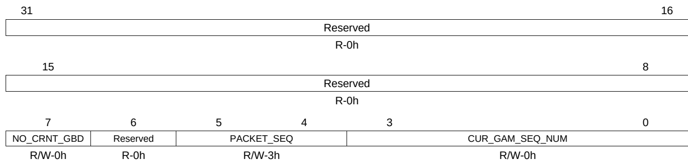
Figure 10-145. Gamut Metadata Register (GAMUT_HEADER3)
