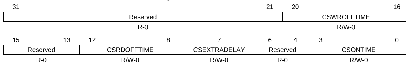
Figure 9-62. GPMC_CONFIG2_i
