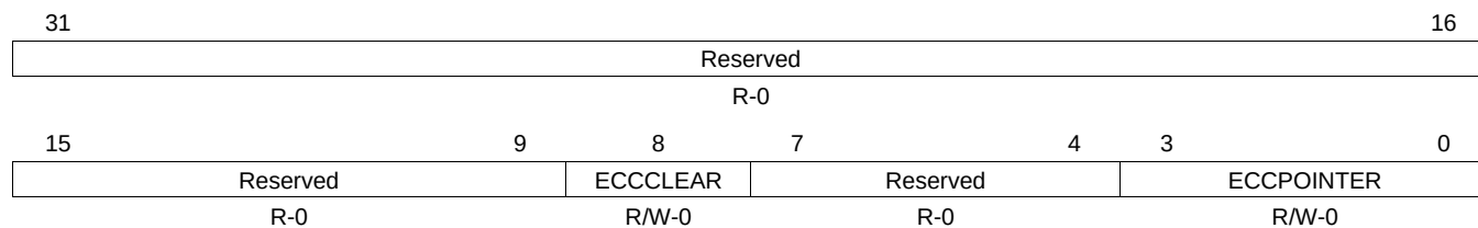
Figure 9-76. GPMC_ECC_CONTROL
