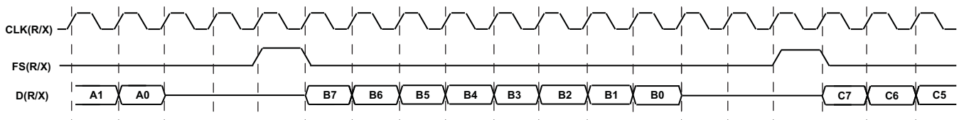
Figure 15-5. Single-Phase Frame for a McBSP Data Transfer
