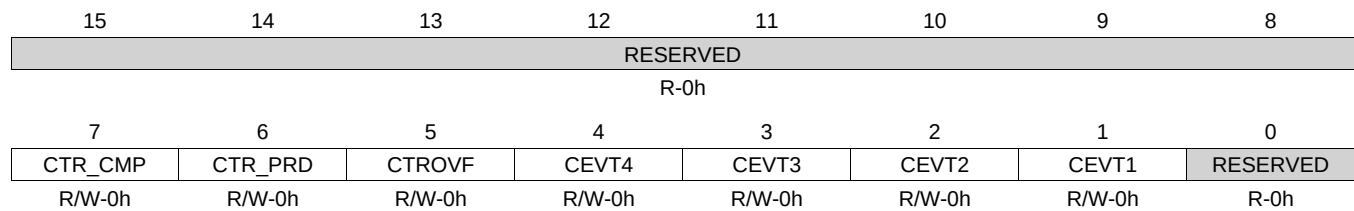
Figure 20-19. ECFRC Register
