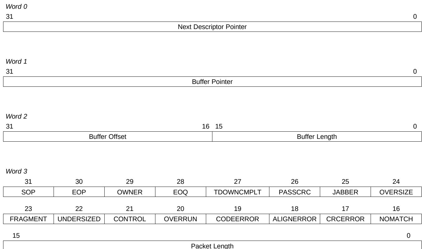
Figure 32-8. Receive Buffer Descriptor Format
