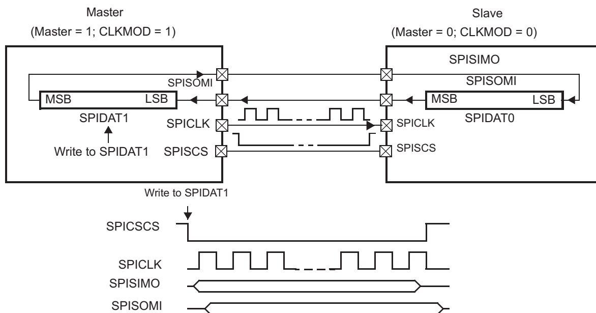
Figure 28-3. Operation with \overline{\text{SPISCS}}
