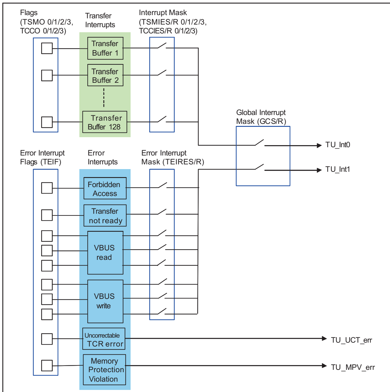
Figure 26-28. Transfer Unit Interrupt Structure
