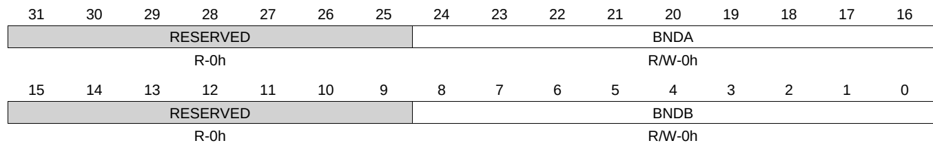
Figure 22-42. ADBNDCR Register
