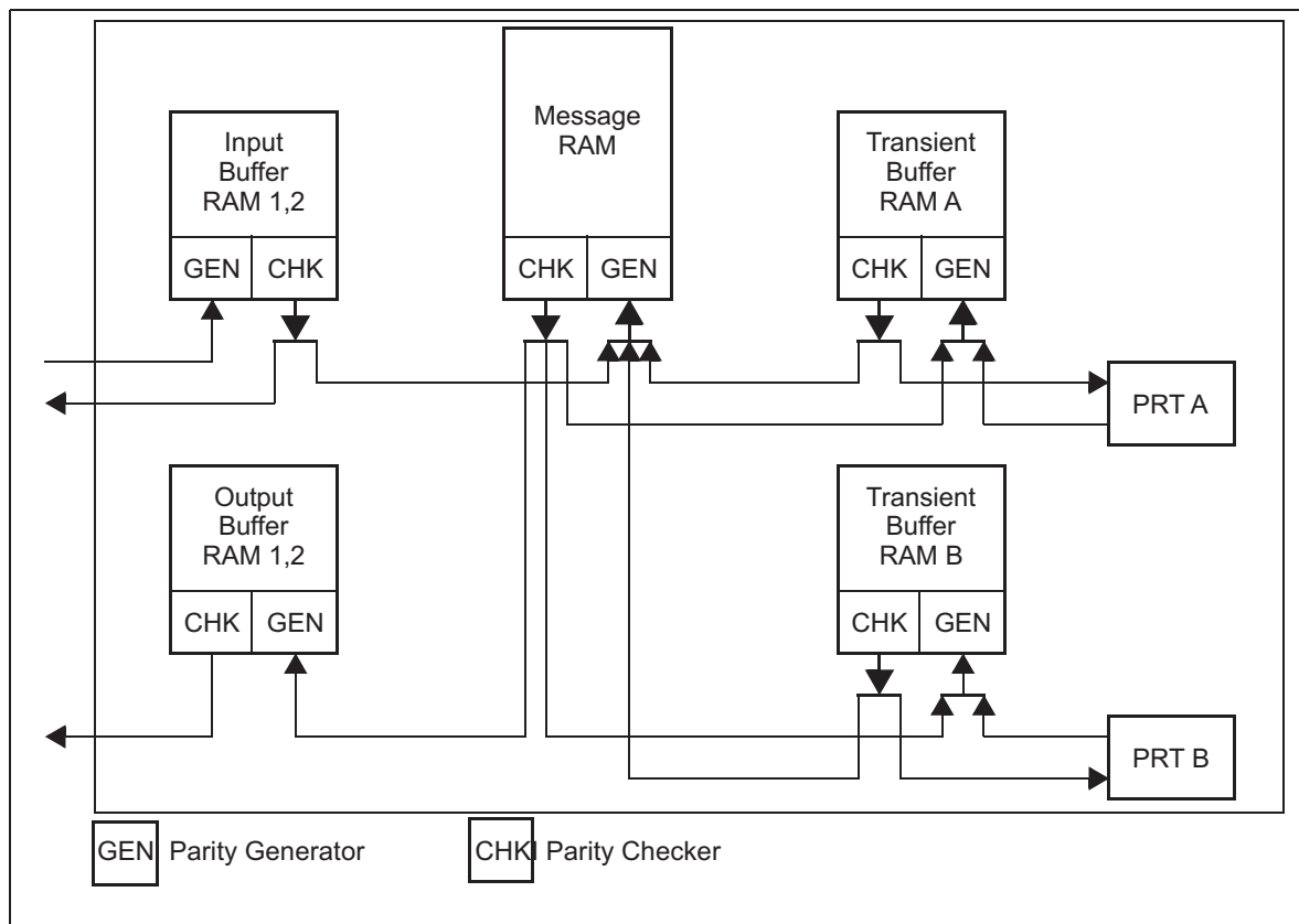
Figure 26-27. Parity Generation and Check
