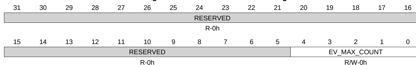
Figure 22-96. ADEVMAXCOUNT Register
