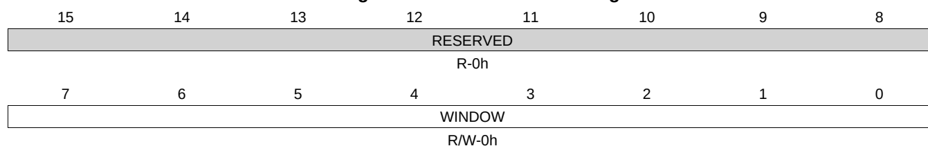
Figure 19-97. DCFWINDOW Register
