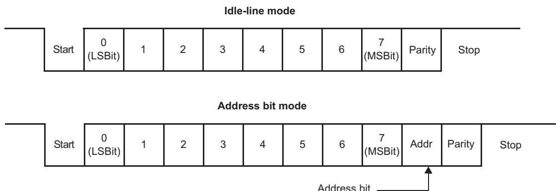
Figure 30-2. Typical SCI Data Frame Formats
