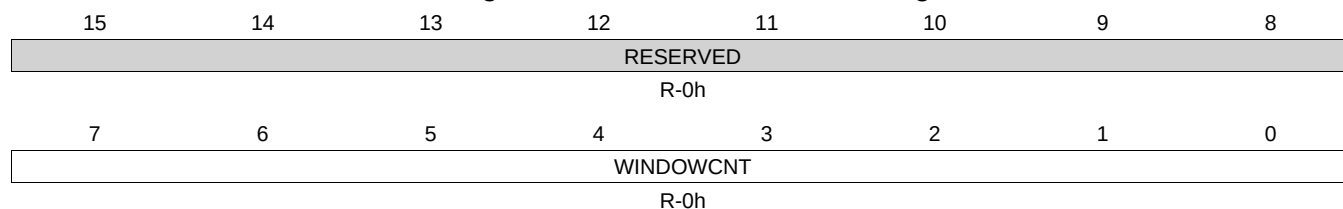
Figure 19-100. DCFWINDOWCNT Register
