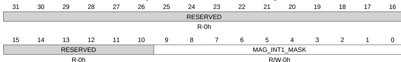
Figure 22-74. ADMAGINT1MASK Register
