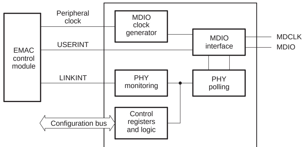
Figure 32-10. MDIO Module Block Diagram
