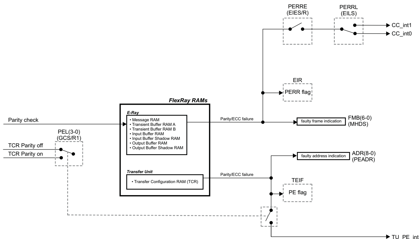
Figure 26-26. Parity Structure
