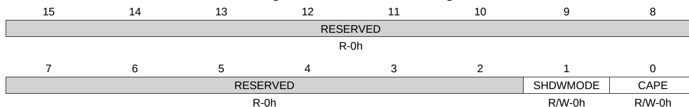
Figure 19-96. DCCAPCTL Register
