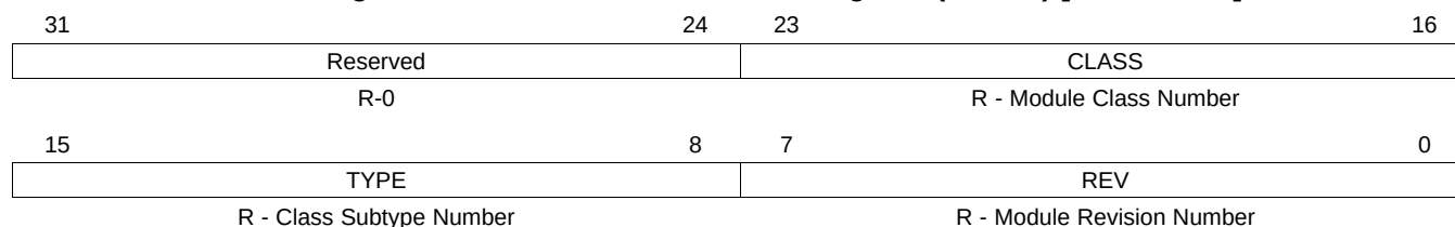
Figure 24-36. Module Identification Register (HTU ID) [offset = 60h]
