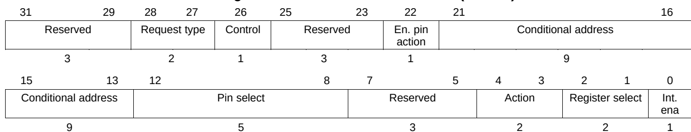
Figure 23-127. PWCNT Control Field (C31:C0)
