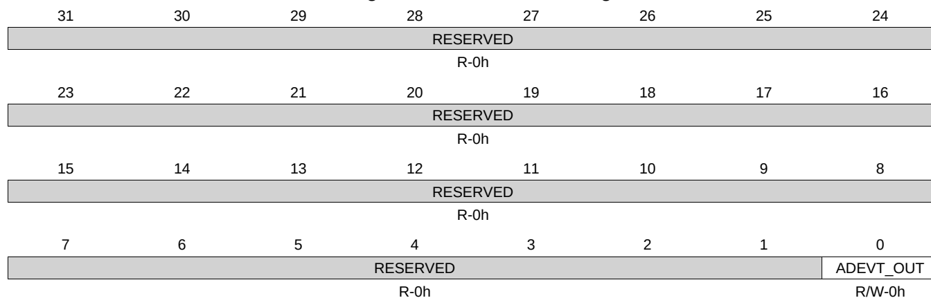
Figure 22-63. ADEVTOUT Register
