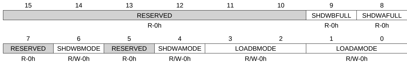
Figure 19-68. CMPCTL Register
