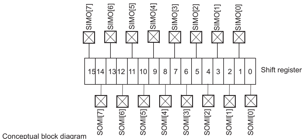
Figure 28-20. Eight-data Line Mode (Phase 0, Polarity 0)
