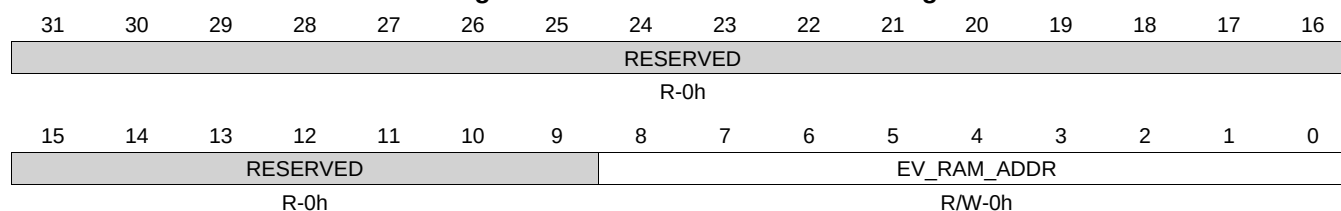
Figure 22-86. ADEVRAMWRADDR Register
