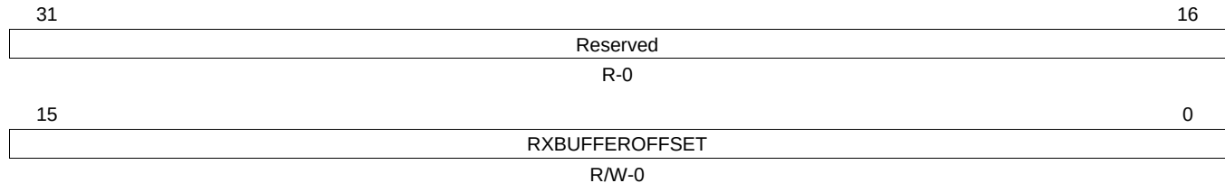
Figure 32-63. Receive Buffer Offset Register (RXBUFFEROFFSET)
