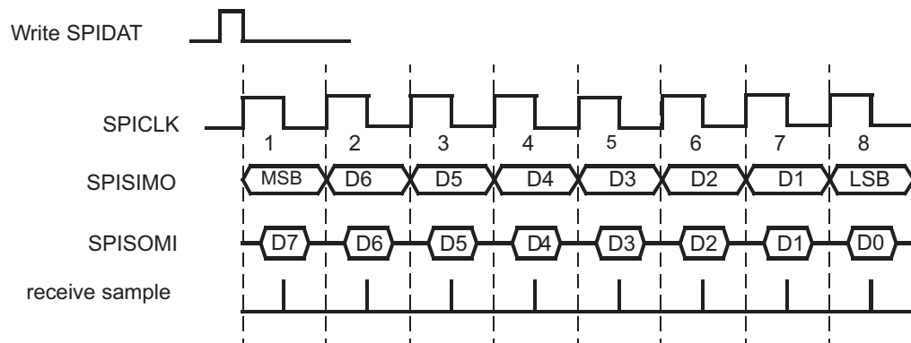
Figure 28-8. Clock Mode with Polarity = 0 and Phase = 0
