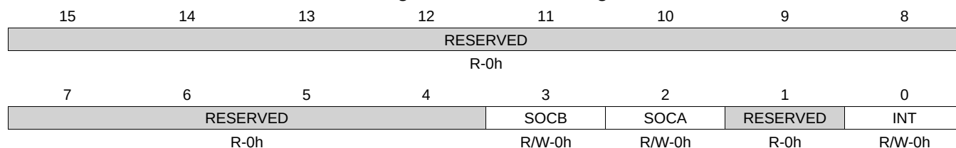
Figure 19-88. ETFRC Register
