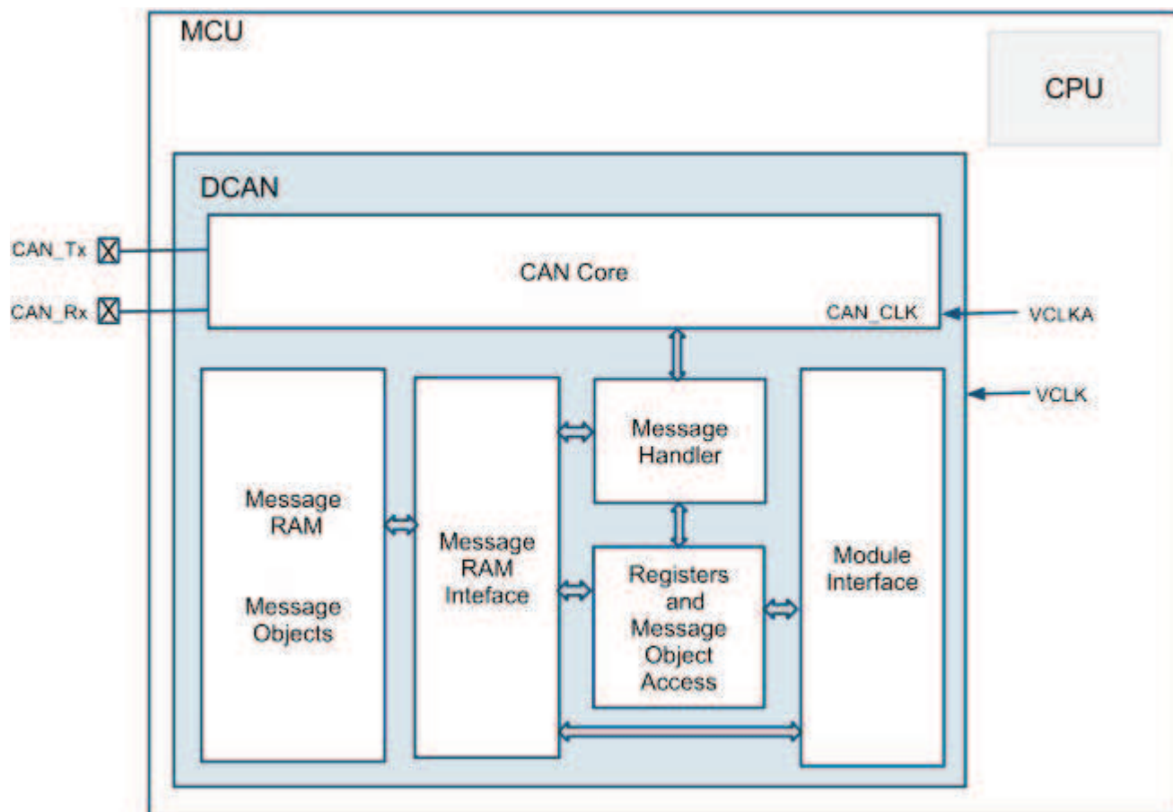
Figure 27-1. Block Diagram
