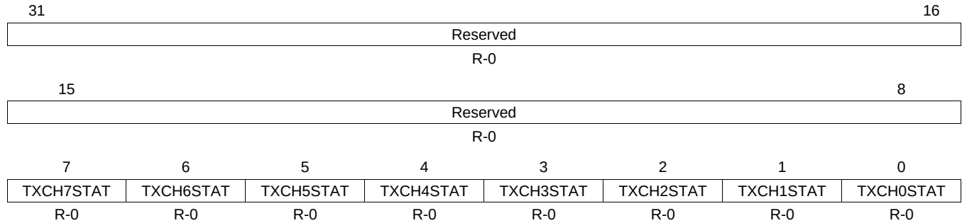
Figure 32-21. EMAC Control Module Transmit Interrupt Status Register (C0TXSTAT)
