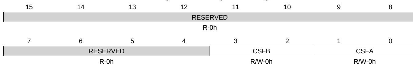
Figure 19-75. AQCSFRC Register
