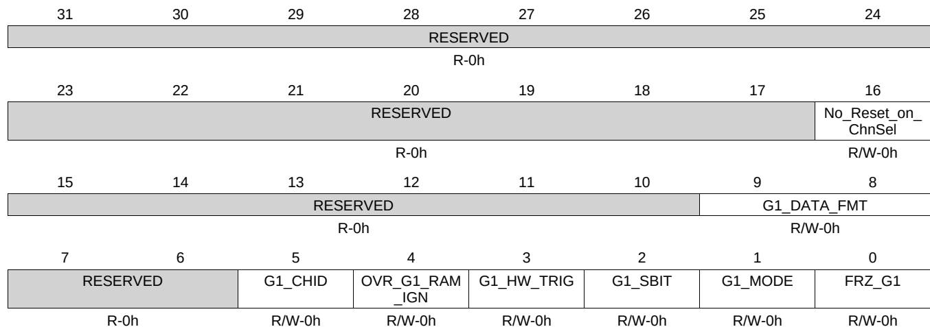
Figure 22-25. ADG1MODECR Register
