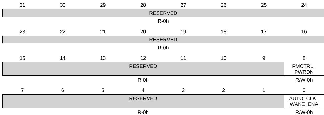
Figure 3-14. GLOBALCTRL1 Register
