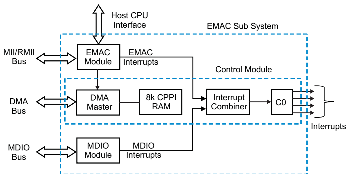
Figure 32-1. EMAC and MDIO Block Diagram
