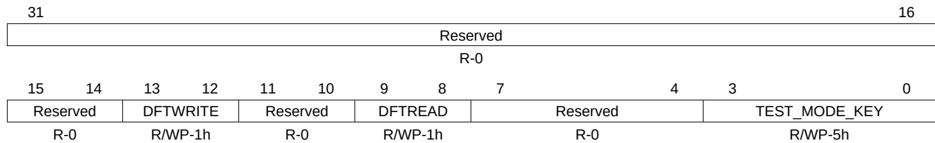
Figure 2-37. DFT Control Register (DFTCTRLREG) [offset = 90h]
