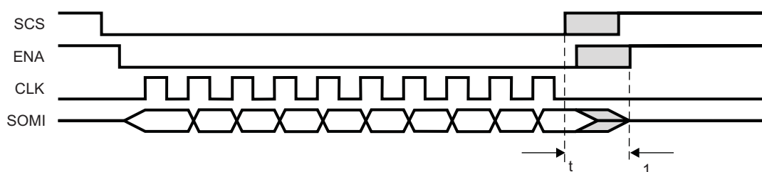
Figure 28-47. Transmit-Data-Finished-to-ENA-Inactive-Timeout
