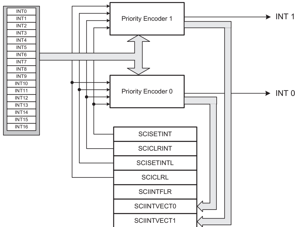
Figure 30-6. General Interrupt Scheme
