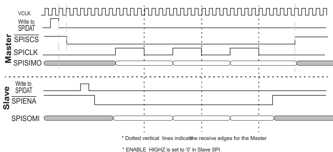
Figure 28-83. SPI/MibSPI pins during Master/Slave mode with 5-pin configuration
