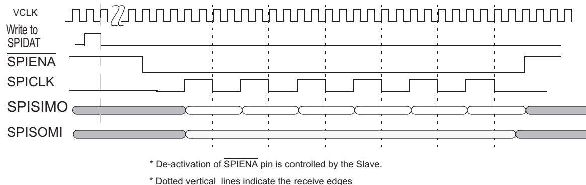
Figure 28-82. SPI/MibSPI pins during Master mode in 4pin with \overline{\text{SPIENA}} configuration
