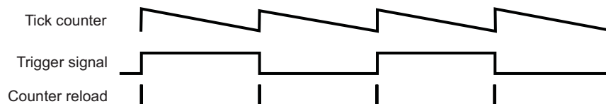
Figure 28-60. Tick Counter Operation
