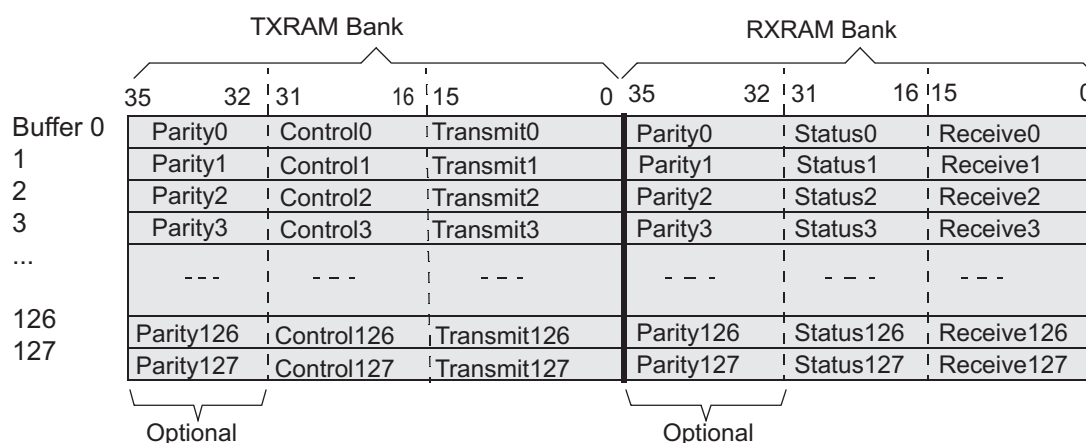
Figure 28-75. Multi-Buffer RAM Configuration
