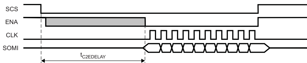
Figure 28-48. Chip-Select-Active-to-ENA-Signal-Active-Timeout
