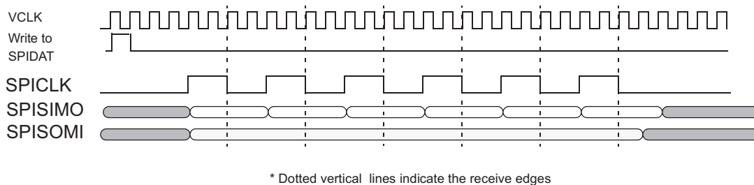
Figure 28-80. SPI/MibSPI Pins during Master mode 3-pin configuration
