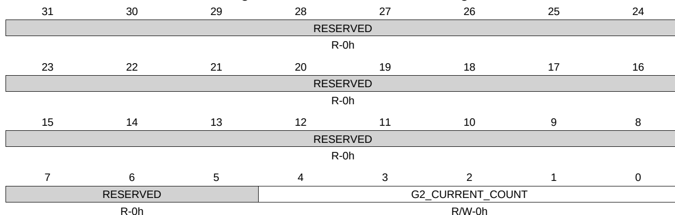
Figure 22-99. ADG2CURRCOUNT Register
