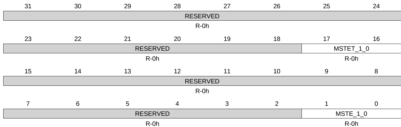
Figure 3-20. MPDDCSTAT2 Register
