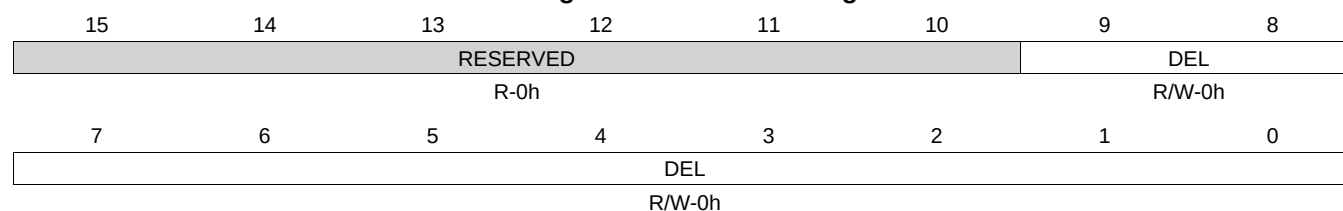
Figure 19-76. DBFED Register
