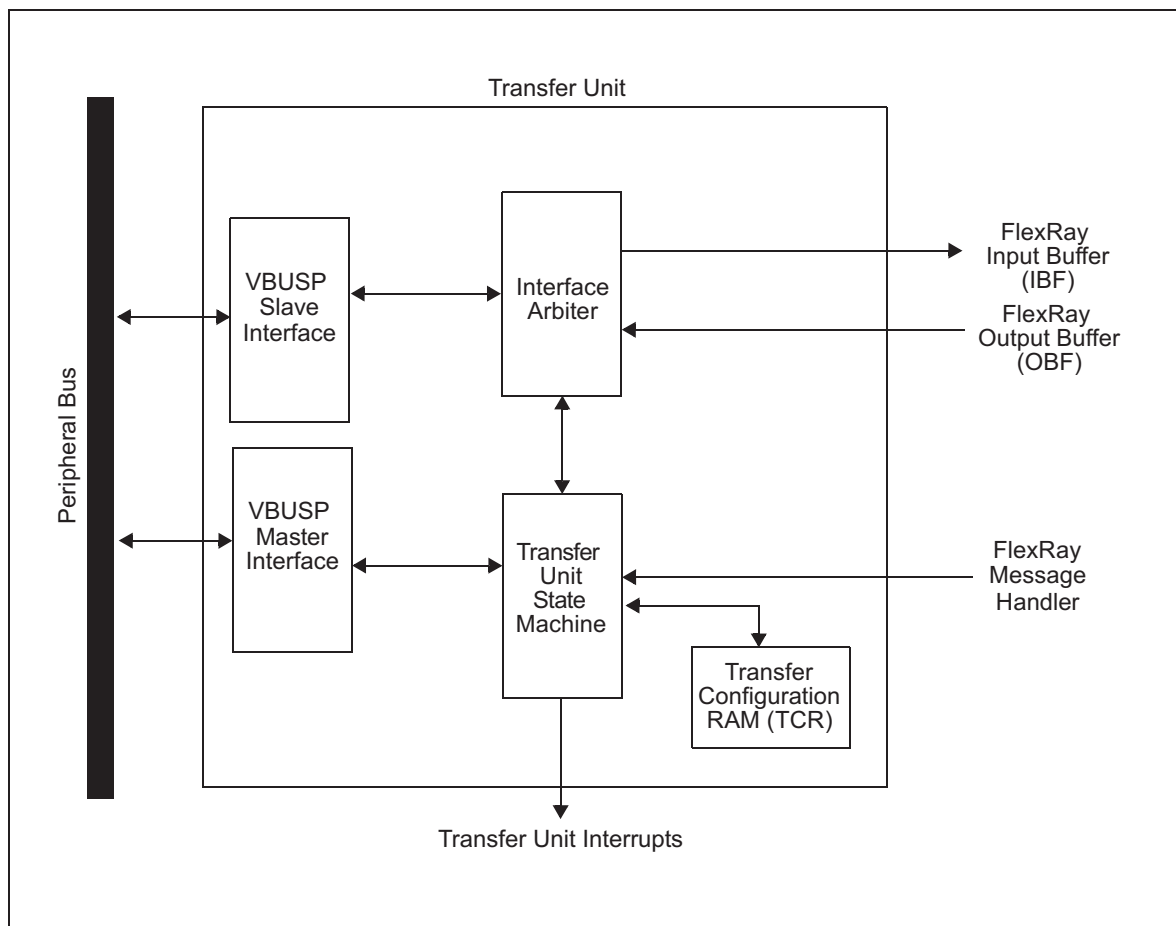
Figure 26-3. Transfer Unit
