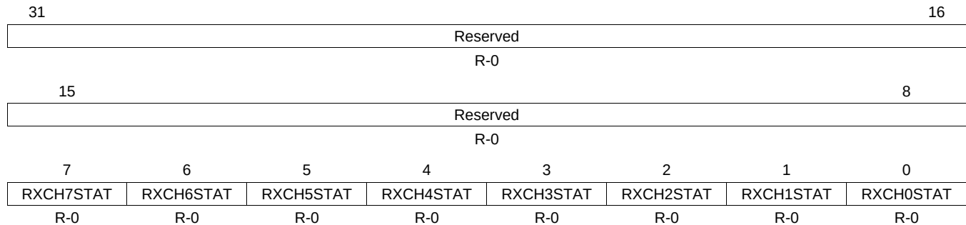
Figure 32-20. EMAC Control Module Receive Interrupt Status Register (C0RXSTAT)
