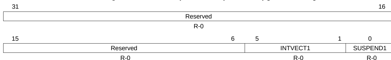
Figure 28-52. Interrupt Vector 1 (INTVECT1) [offset = 64h]
