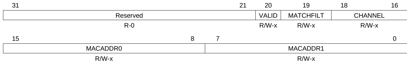
Figure 32-81. MAC Address Low Bytes Register (MACADDRLO)
