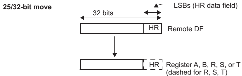
Figure 23-118. MOV32 Move Operation for REMTOREG (Case 11)
