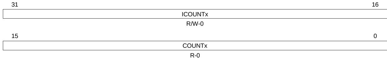
Figure 28-65. DMAxCOUNT Register (ICOUNT) [offset = F8h-114h]
