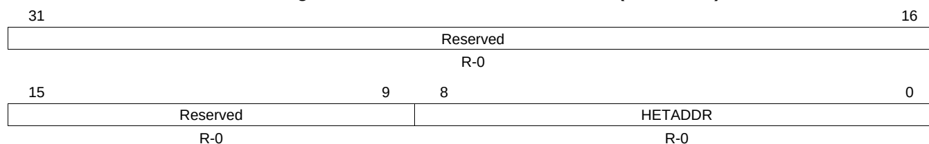
Figure 23-37. N2HET Current Address (HETADDR)
