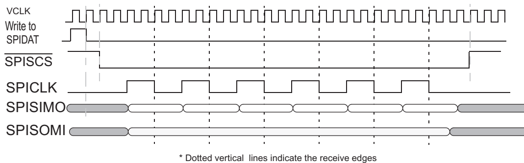
Figure 28-81. SPI/MibSPI pins during Master mode 4-pin with \overline{\text{SPISCS}} configuration.
