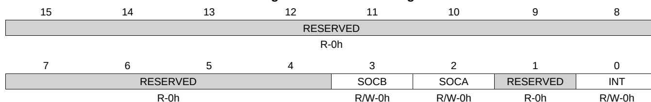
Figure 19-89. ETCLR Register
