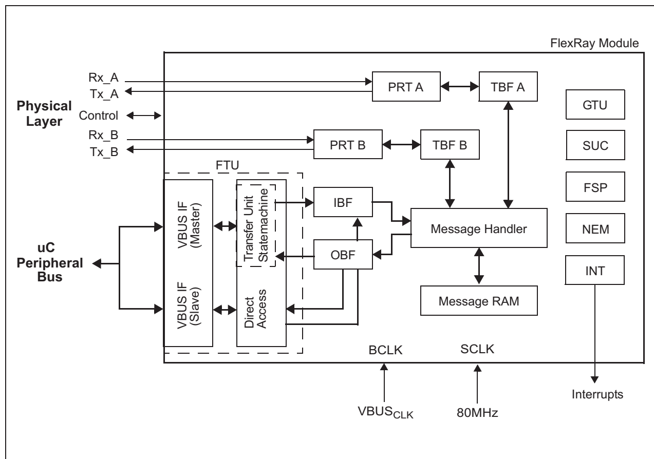
Figure 26-1. Block Diagram
