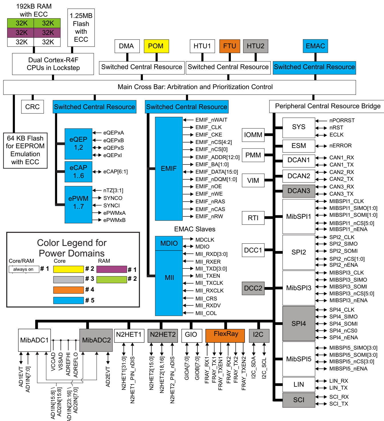
Figure 1-1. Block Diagram
