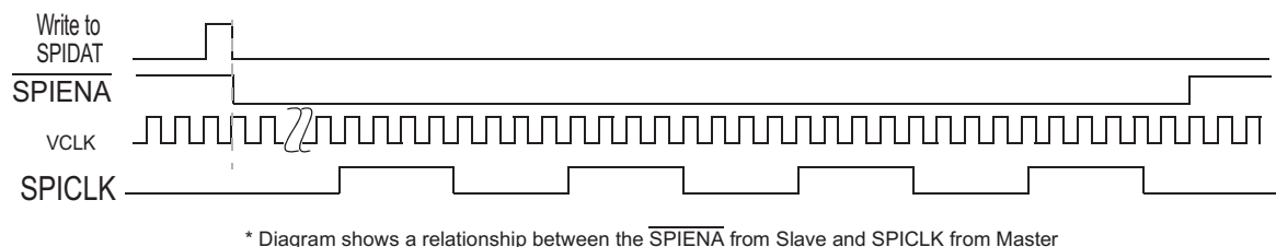
Figure 28-85. SPI/MibSPI pins during Slave mode in 4pin with \overline{\text{SPIENA}} configuration
