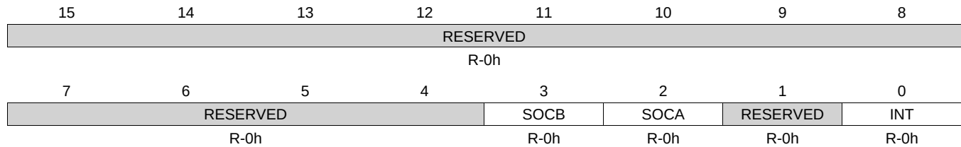
Figure 19-86. ETFLG Register
