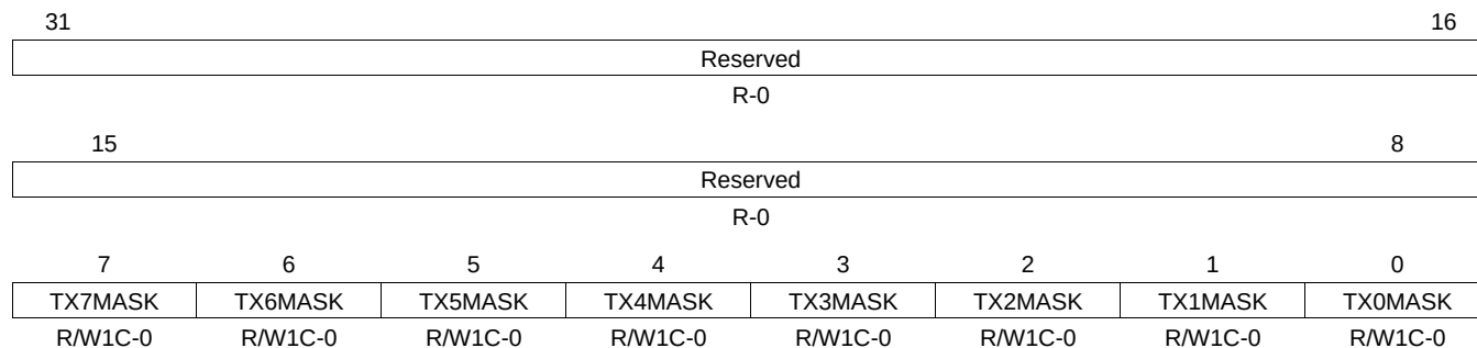
Figure 32-48. Transmit Interrupt Mask Clear Register (TXINTMASKCLEAR)
