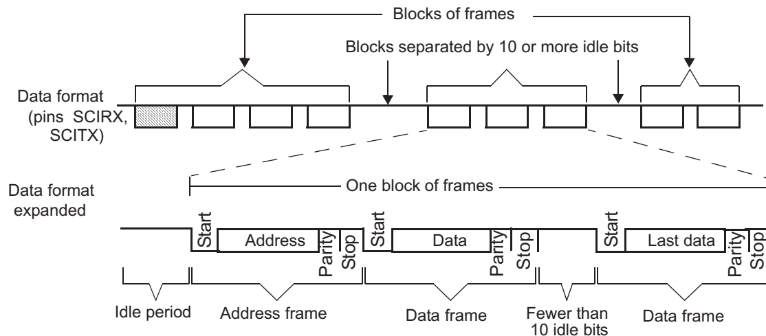
Figure 30-4. Idle-Line Multiprocessor Communication Format
