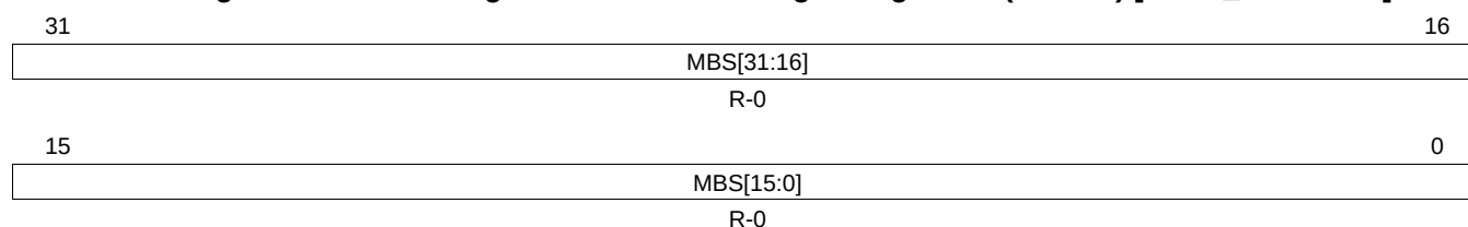
Figure 26-170. Message Buffer Status Changed Register 1 (MBSC1) [offset_CC = 340h]
