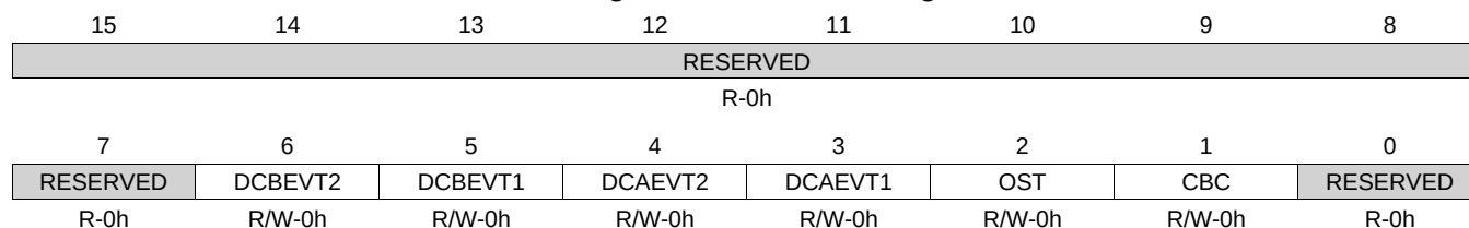
Figure 19-80. TZEINT Register
