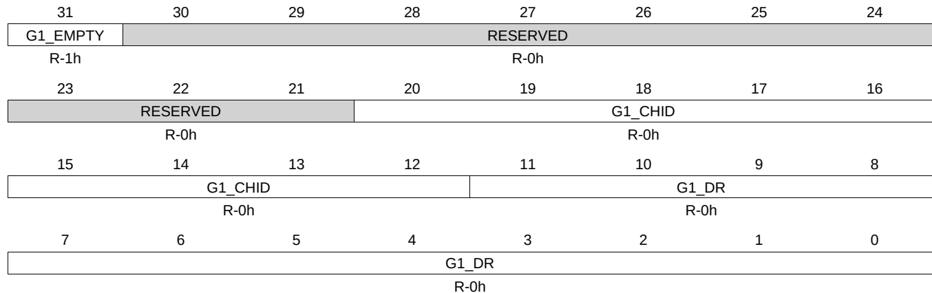
Figure 22-60. ADG1EMUBUFFER Register
