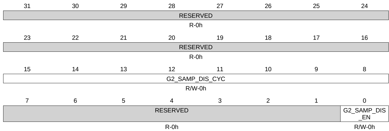
Figure 22-72. ADG2SAMPDISEN Register
