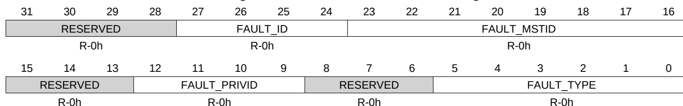
Figure 4-15. FAULT_STATUS_REG Register
