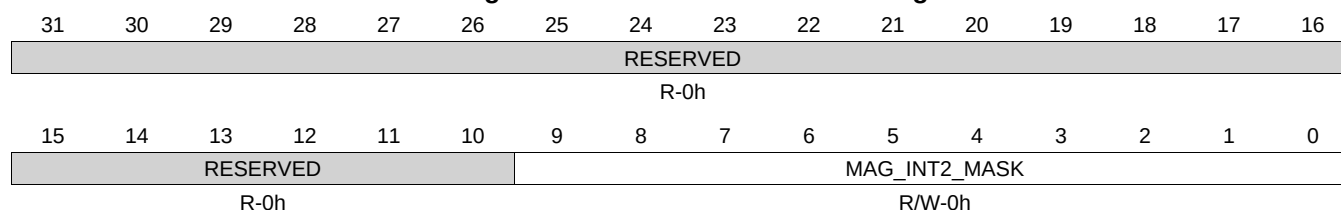
Figure 22-76. ADMAGINT2MASK Register
