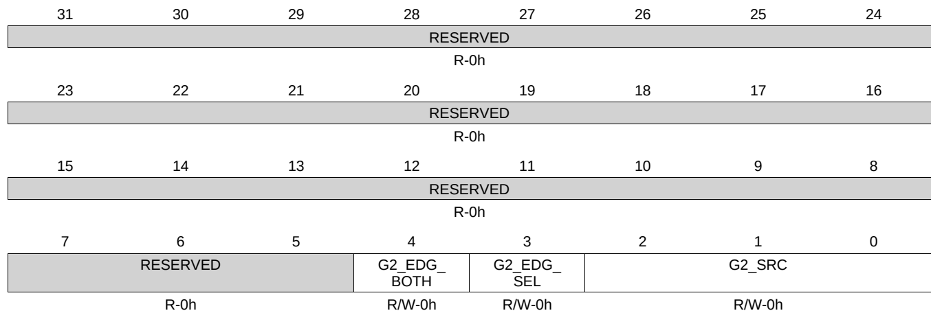
Figure 22-29. ADG2SRC Register
