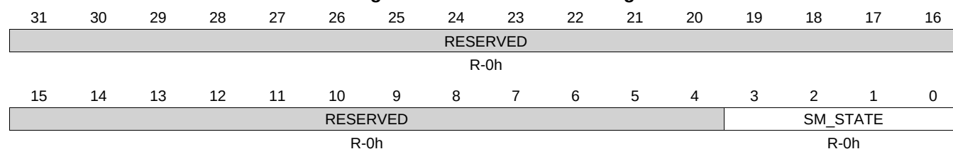
Figure 22-54. ADSTMSTATE Register
