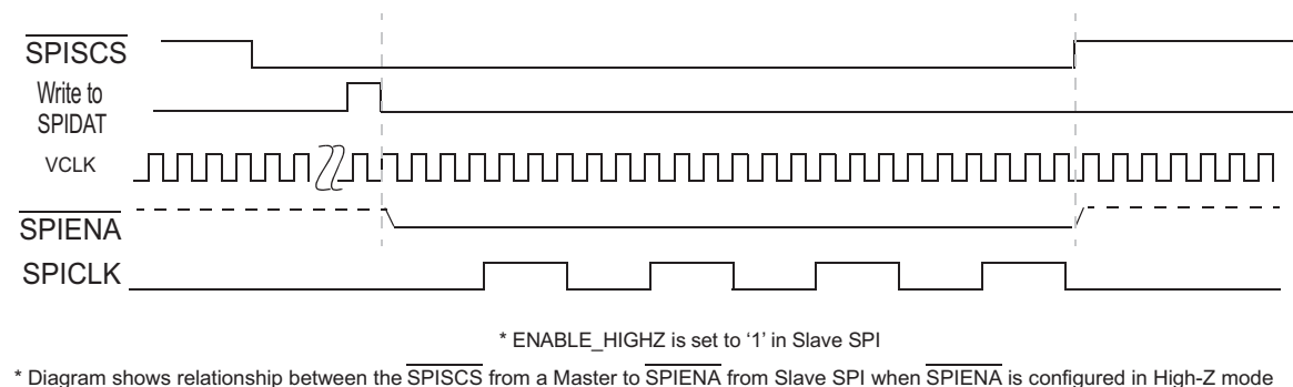
Figure 28-87. SPI/MibSPI pins during Slave mode in 5pin configuration - (Single/Multi Slave).
