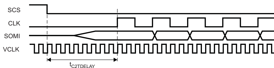
Figure 28-45. Example: t_{C2TDELAY} = 8 VCLK Cycles
