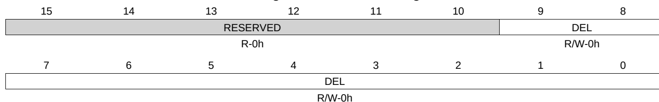
Figure 19-77. DBRED Register
