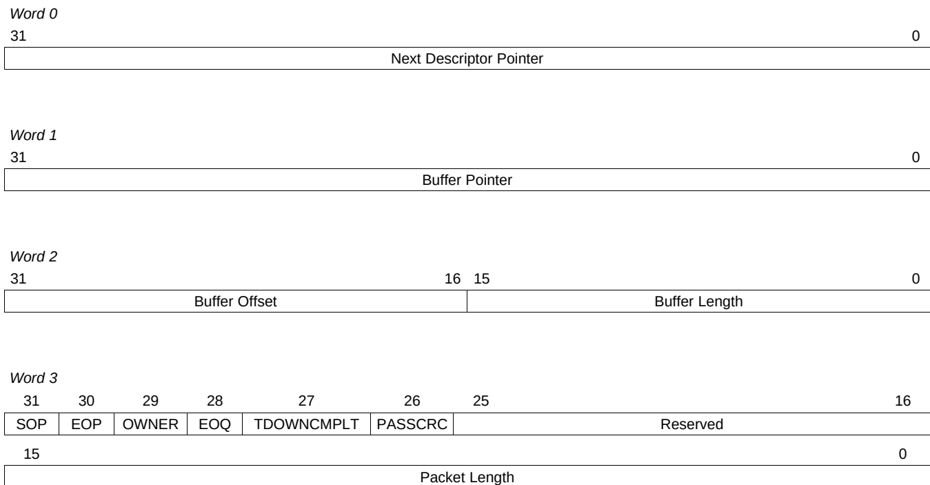
Figure 32-7. Transmit Buffer Descriptor Format
