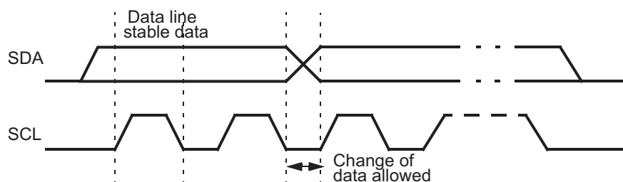
Figure 31-4. Bit Transfer on the I2C Bus
