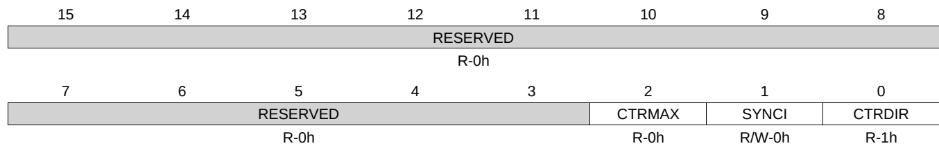
Figure 19-63. TBSTS Register
