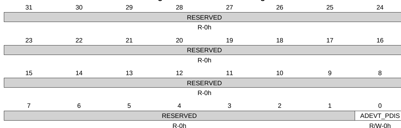
Figure 22-68. ADEVTPDIS Register
