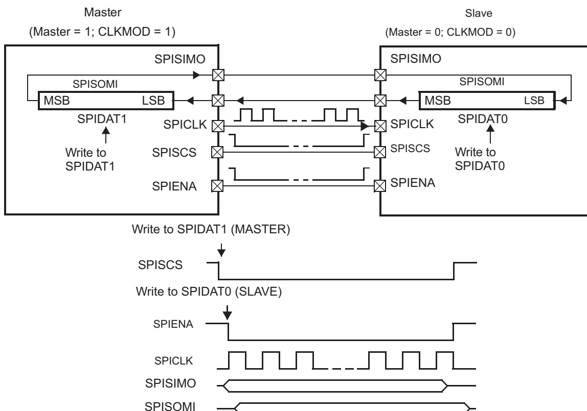
Figure 28-5. SPI Five-Pin Option with \overline{\text{SPIENA}} and \overline{\text{SPISCS}}
