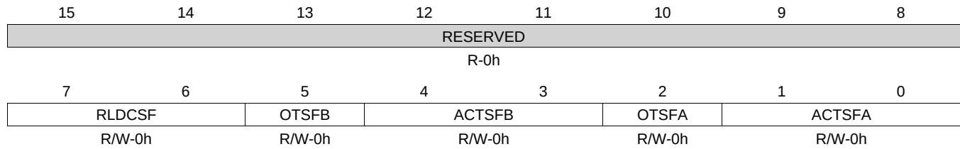
Figure 19-72. AQSFRFC Register
