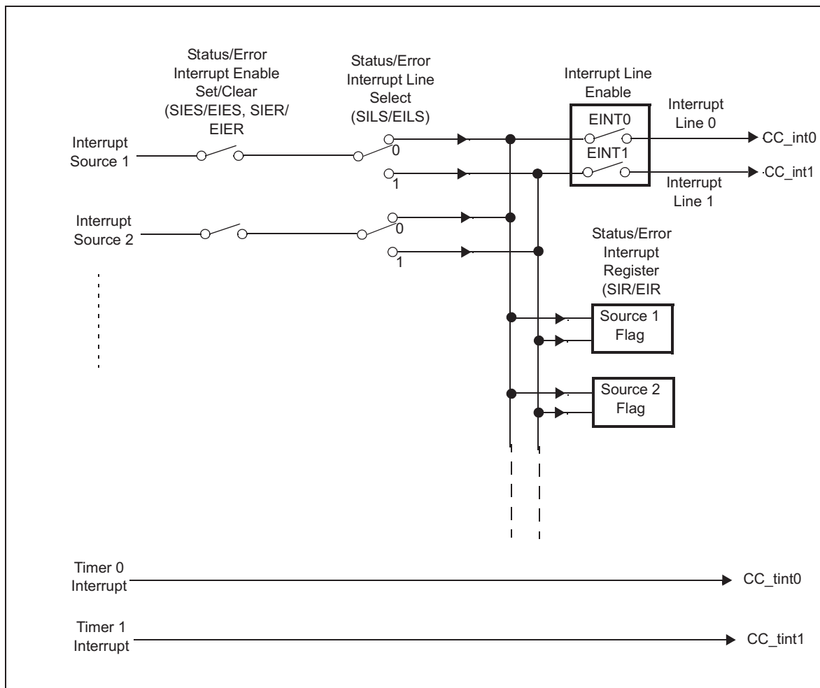
Figure 26-29. Interrupt Structure
