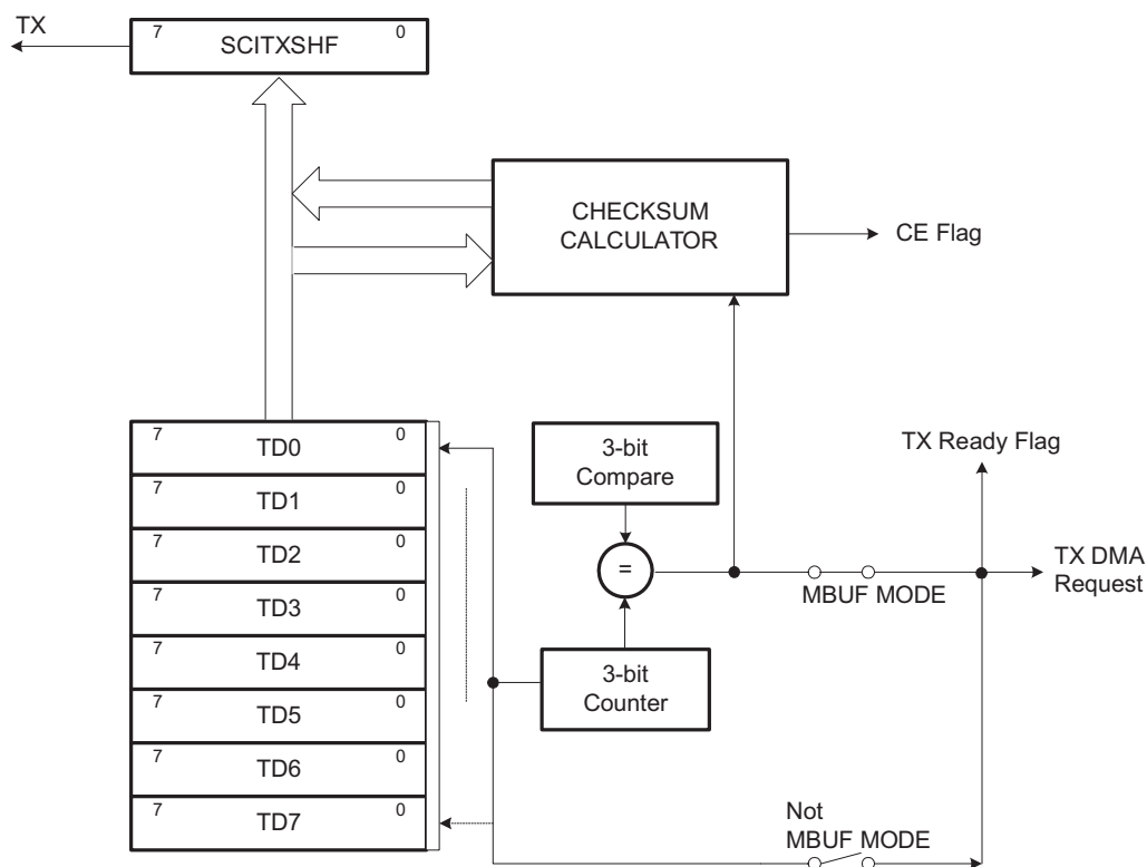
Figure 29-9. Transmit Buffers
