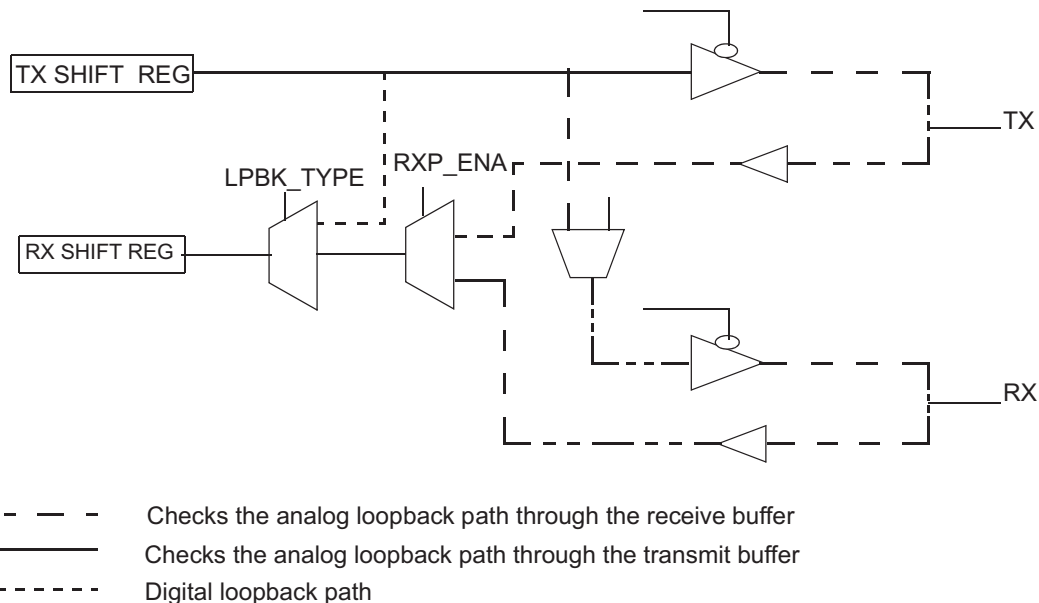
Figure 28-22. I/O Paths during I/O Loopback Modes
