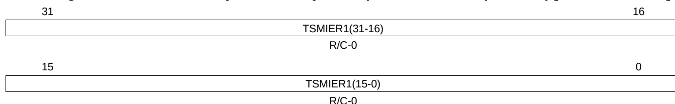
Figure 26-88. Transfer to System Memory Interrupt Enable Reset 1 (TSMIER1) [offset_TU = 104h]
