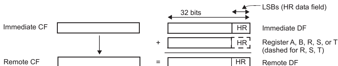
Figure 23-132. RADM64 Add and Move Operation
