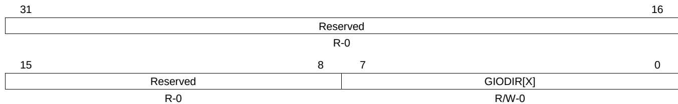
Figure 25-17. GIO Data Direction Registers [A-H][7:0] (GIODIR[A-H]) [address = FFF7BC34h, FFF7BC54h, FFF7BC74h, FFF7BC94h, FFF7BCB4h, FFF7BCD4h, FFF7BCF4h, FFF7BD14h]
