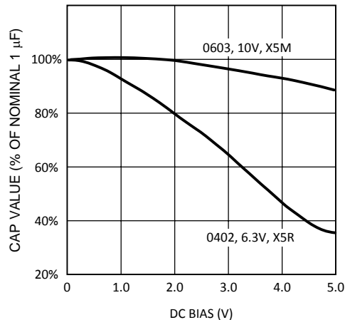
Figure 31. Graph Showing a Typical Variation in Capacitance vs. DC Bias
