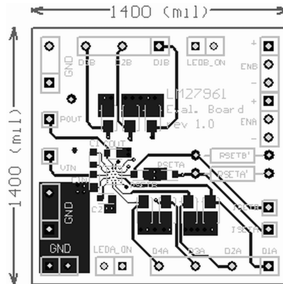
Figure 1. Top Layer
