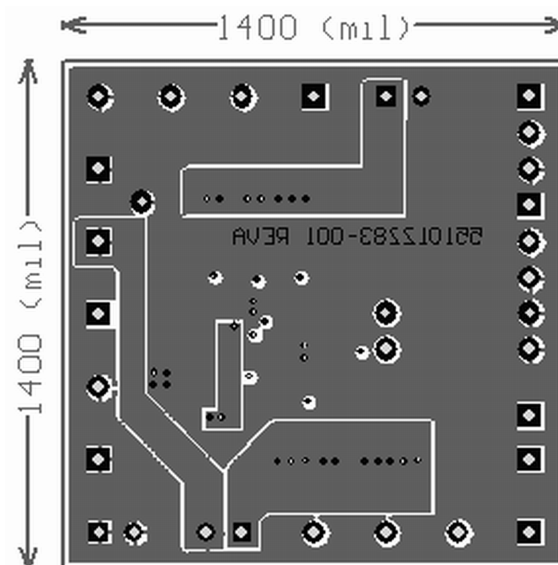
Figure 2. Bottom Layer (top view, unmirrored)
