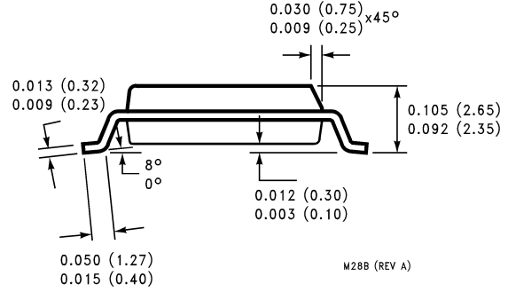
Small Outline Molded Dual-In-Line Package (M) Order Number COP881C-XXX/WM, COP981C-XXX/WM, COP681C-XXX/WM or COP981CH-XXX/WM NS Package Number M28B
