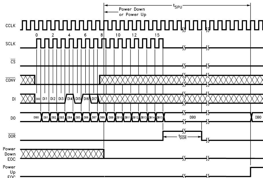
Figure 33. ADC12L038 Software Power Up/Down with \overline{CS} Continuously Low and 16-Bit Digital Output Format
