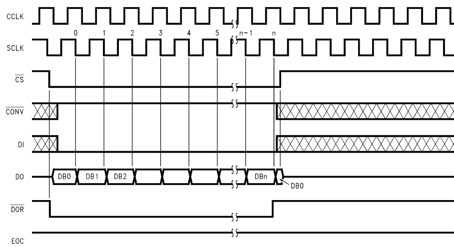
Figure 26. ADC12L038 Read Data without Starting a Conversion Using CS
