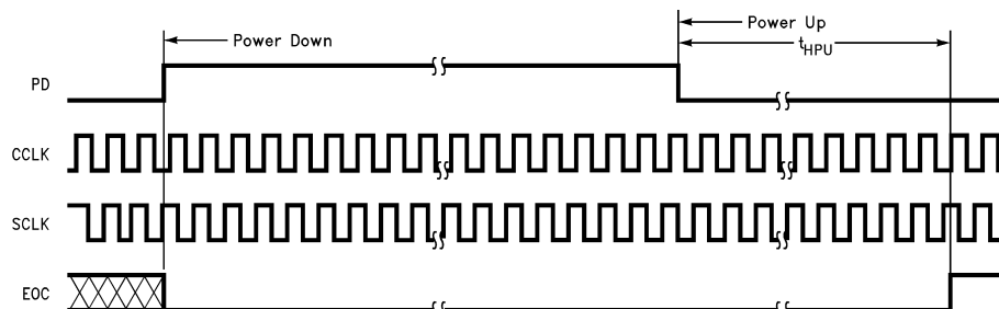
Figure 33. ADC12L038 Software Power Up/Down with \overline{CS} Continuously Low and 16-Bit Digital Output Format
