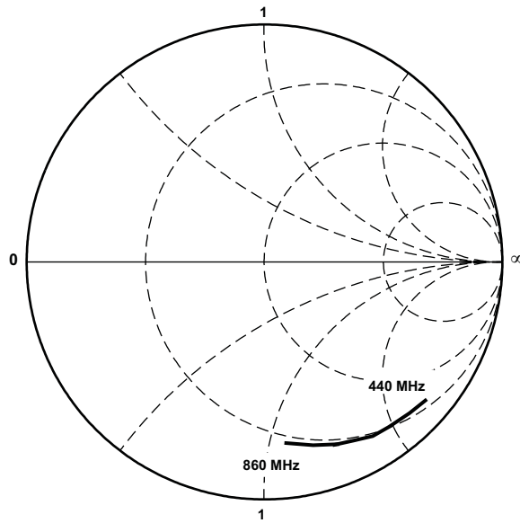
Figure 30. UHF RFIN
