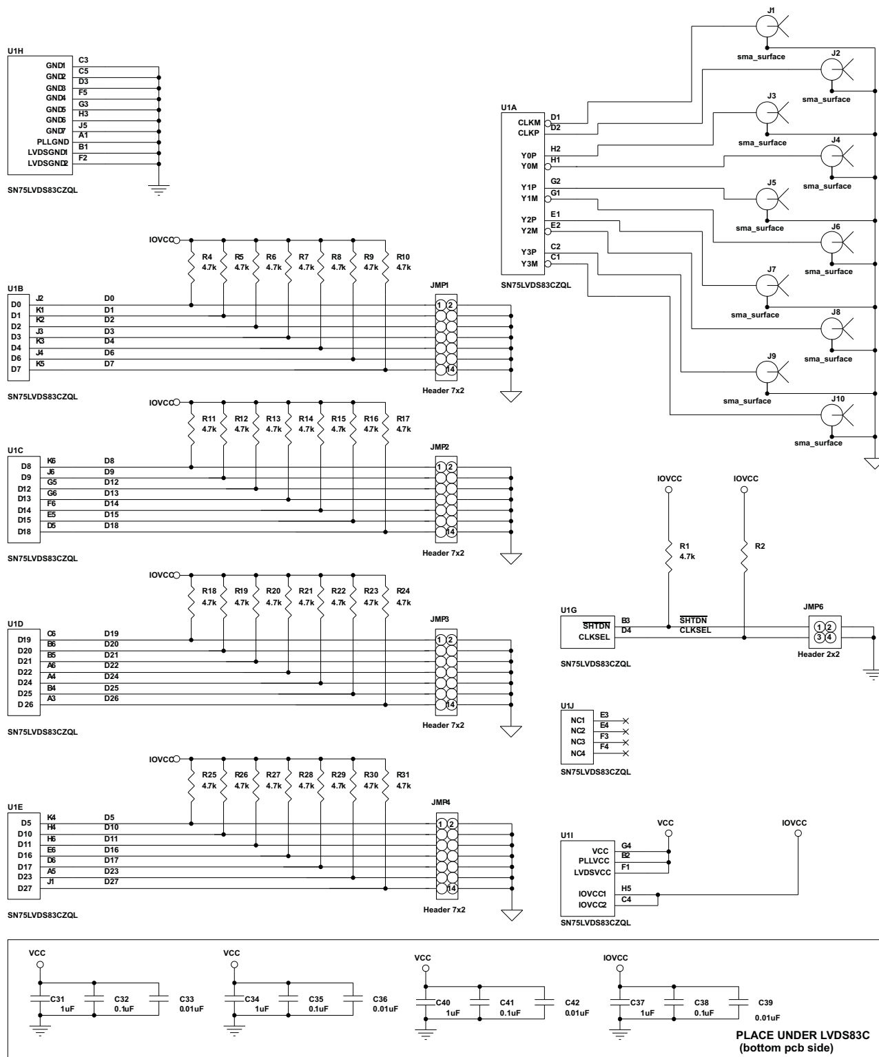
Figure 15. Schematic Example (SN75LVDS83C Evaluation Board)
