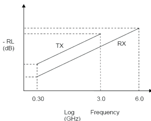
Figure 5. TX, RX Differential Return Loss Limits
