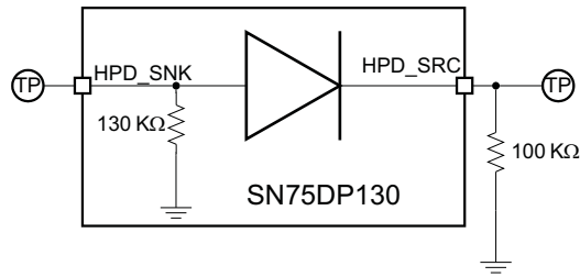
Figure 10. HPD Test Circuit
