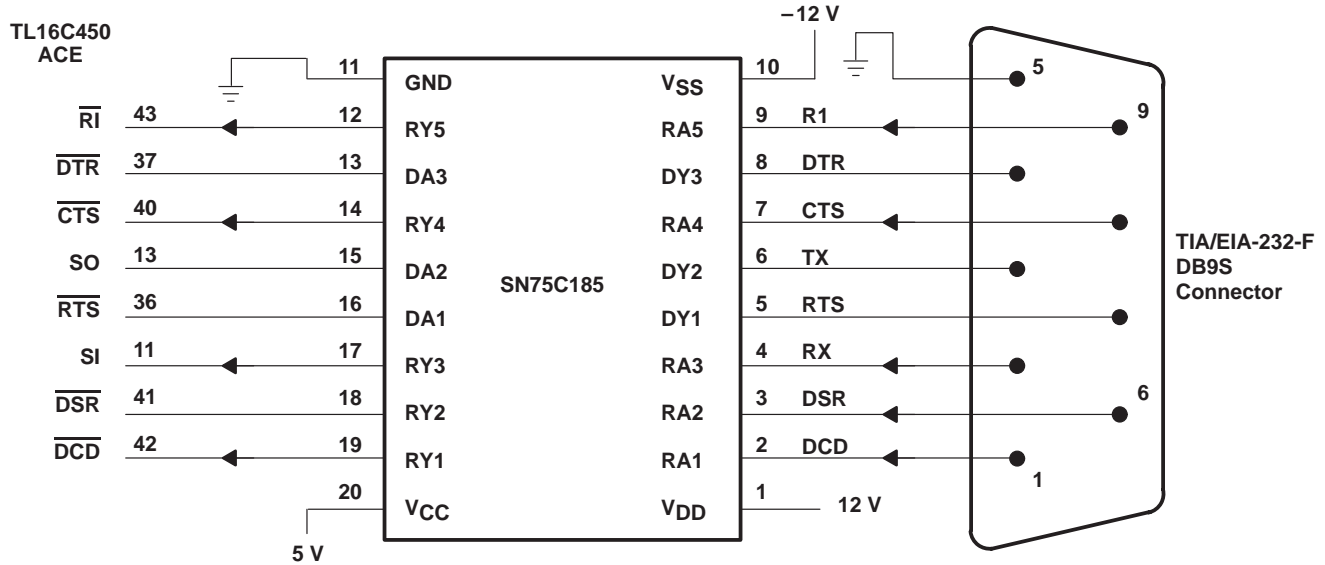
Figure 7. Typical Connection
